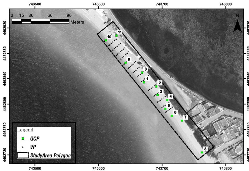
Figure 4.2 Study area highlighted. GCPs used as reference points (green square); VPs for validation purposes as black triangle.
