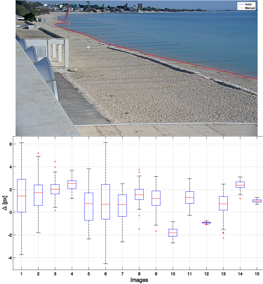
Figure 3.8 Top: Example of comparison between manually and automatic shoreline contours with transects overlapped (cam PC_{vs1} ); Bottom: Statistic box plots of results for 15 images analysed.
