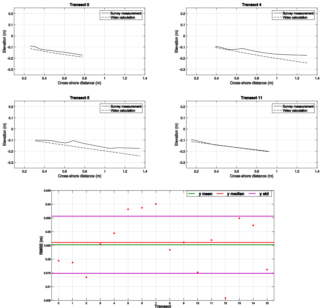
Figure 3.10 Top: Comparison of intertidal bathymetry derived from video analysis with the field measured profiles for transects n. 0, 4, 5 and 11 (see Figure 3.9). Bottom: Vertical RMS error (m) for all transects analysed.
