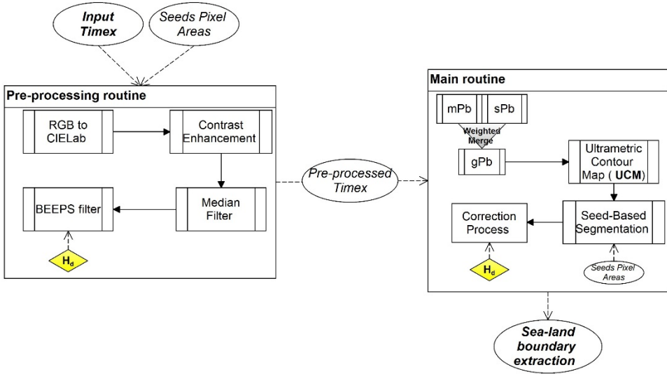
Figure 2.3 Block diagram of algorithms implemented for image pre-processing and main routine.
