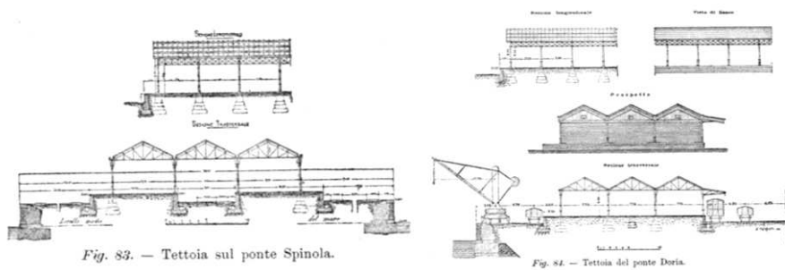
Figure 1.46 Iron sheds built in XIX century in the port of Genoa, located on the docks and served by mechanical cranes for loading/unloading (Giaccone, 1891)
