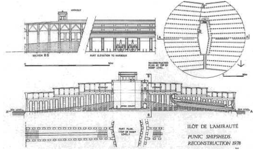
Figure 1.10 Reconstruction of the Admiralty Palace in Carthage ancient port (Franco, 1996)
