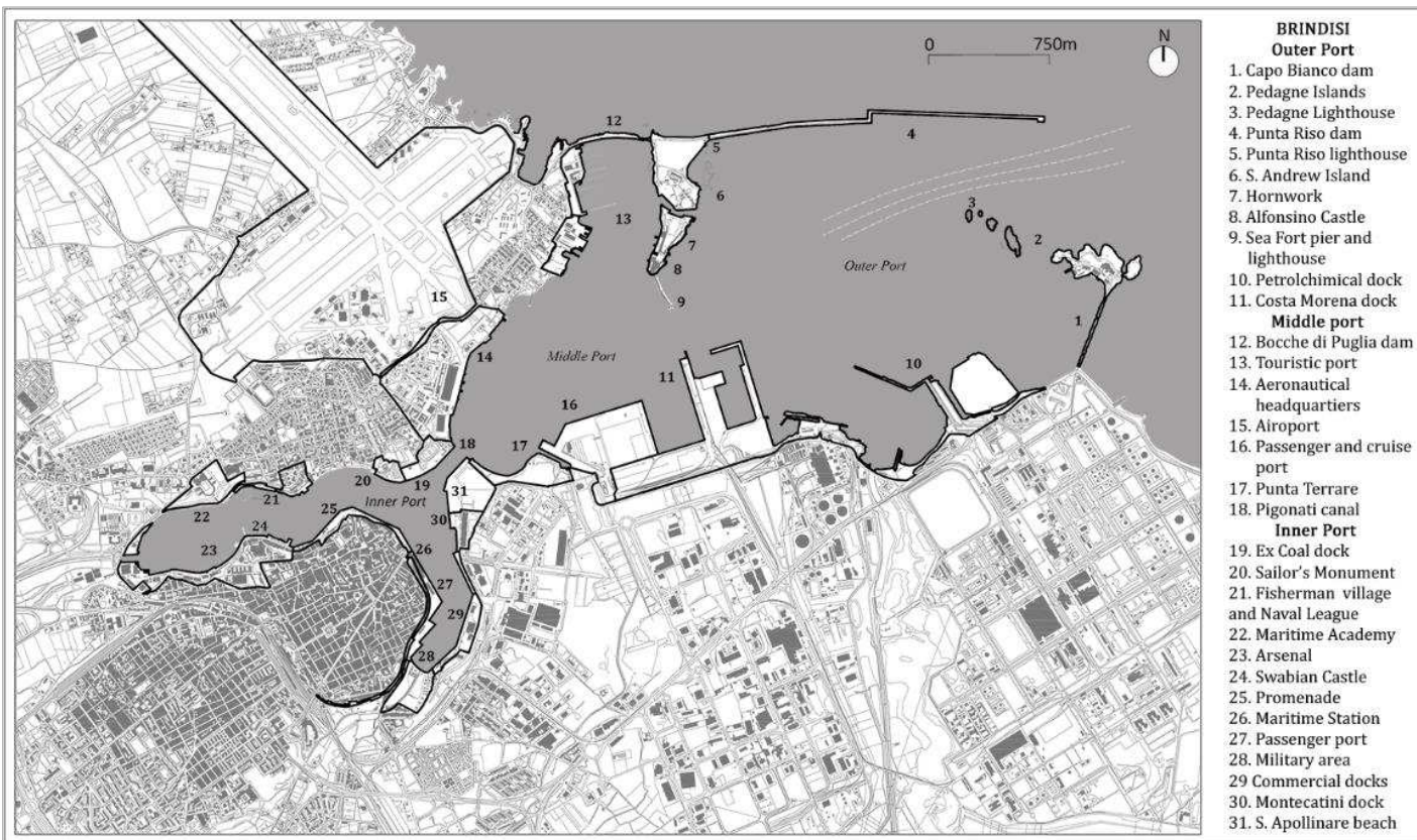
Figure 7. 6 Morphology of the port of Brindisi
