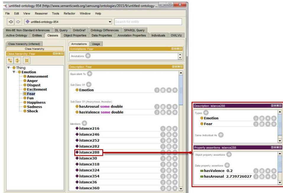
Figure 3.21: Knowledge Base
