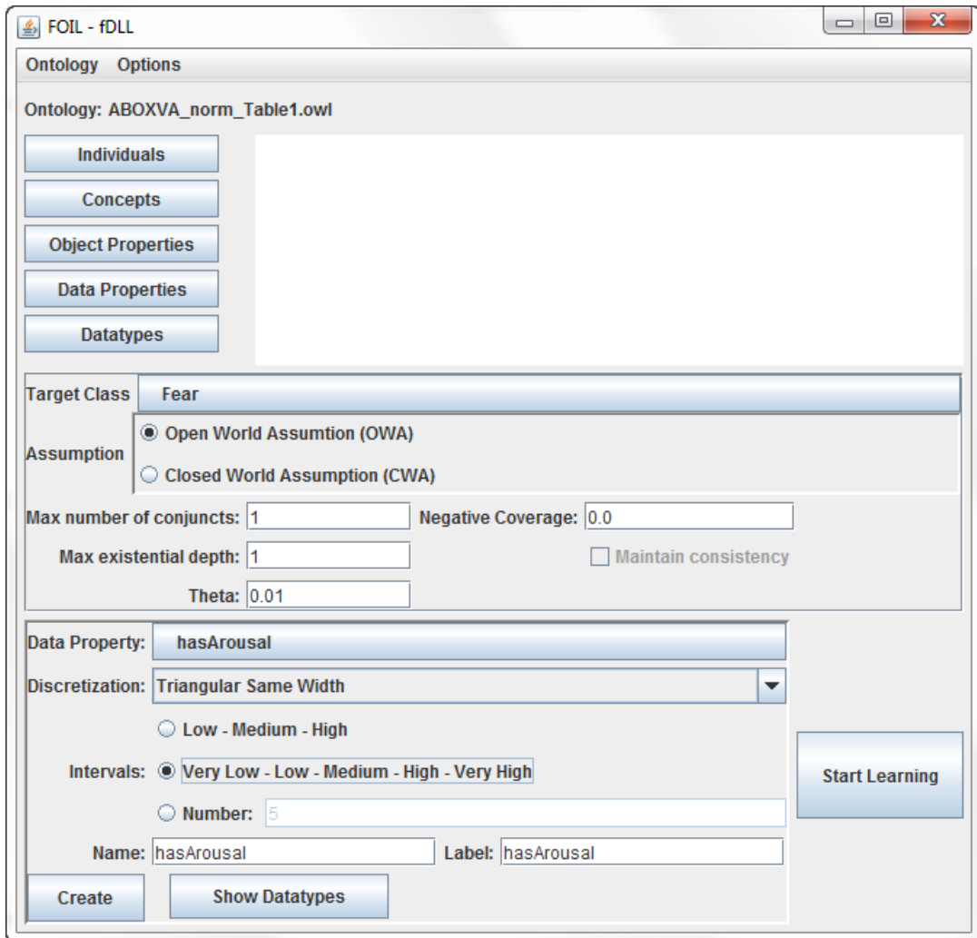
Figure 3.22: Fuzzy DL learner GUI.
