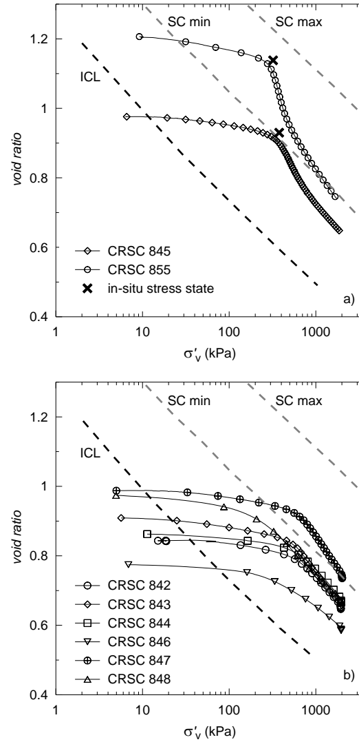
Figure 3. Results from CRSC tests on: a) natural NC BBC; b) natural OC BBC (adapted from Nikolic et al. , 2010)
