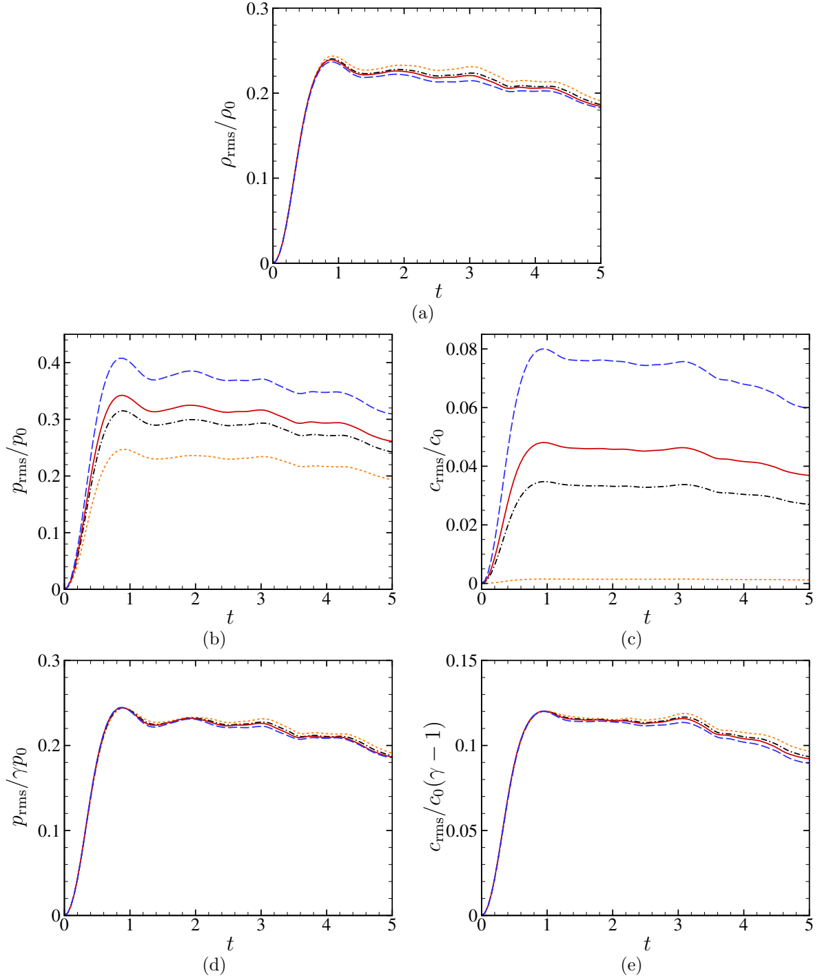
Figure 3.10. PFG simulations: influence of the specific heat ratio. Time evolution of the r.m.s. of the density (a), the pressure (b), the sound speed (c), and the rescaled values of p_{\text{rms}} (d) and c_{\text{rms}} (e) according to equations (3.13) and (3.11), respectively. \cdots : \gamma = 1.0125 ; -\cdot-\cdot- : \gamma = 1.289 ; — : \gamma = 1.4 ; - - - : \gamma = 1.667 .
