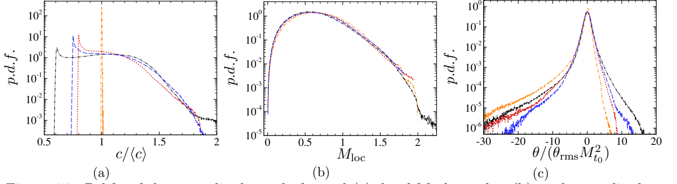
Figure 4.8. P.d.f.s of the normalized speed of sound (a), local Mach number (b), and normalized dilatation (c) for M_{t_0} = 1 ( t = 2 ). — · — ·: PP11-PFG; — · — · — ·: PP11-VDW; - - - -: PP11-MAH-IC1; - - - -: PP11-MAH-IC2.
