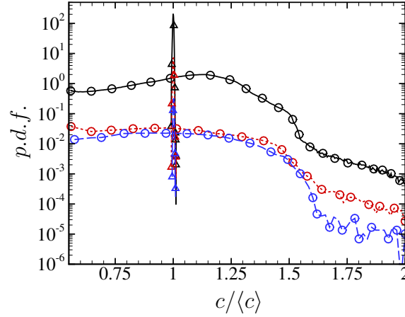
Figure 3.23. Probability density function of the normalized sound speed conditioned on \theta/\theta_{\text{rms}} at M_{t_0} = 1 . .....: [-\infty, -2] ; ---: [2, \infty] ; —: [-\infty, \infty] ; \circ : VDW; \triangle : PFG.
