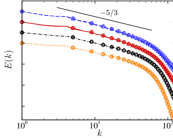
Figure 3.13. PFG and DG simulations. Kinetic energy spectra at t = 2.5 at various initial turbulent Mach numbers. \cdots : M_{t_0} = 0.2 ; -\cdot-\cdot- : M_{t_0} = 0.5 ; — : M_{t_0} = 0.8 ; --- : M_{t_0} = 1 . \circ : VDW; \triangle : PFG.
