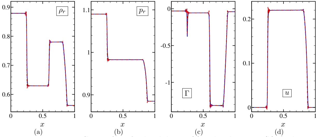
Figure 2.15. Test case DG2. Profiles of reduced density (a), reduced pressure (b), fundamental derivative (c) and velocity (d). Grid: 400 cells, t^* = 0.45 . ---: DRP11 ( r_{th} = 10^{-5} ); -.-.: DNC9 ( k_2 = 1 ); —: Cinnella (2006).
