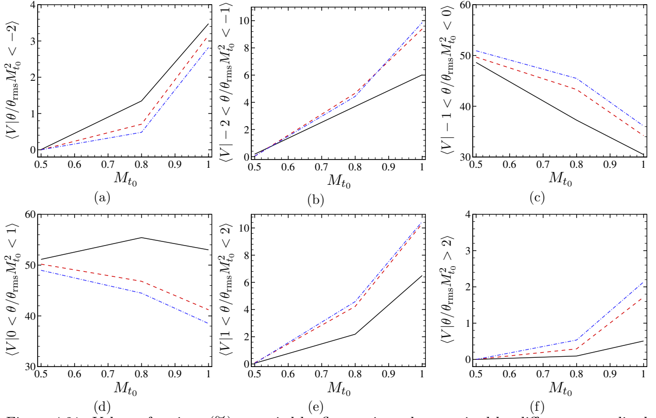
Figure 4.21. Volume fractions (%) occupied by flow regions characterized by different normalized dilatation intervals as a function of M_{t_0} ( t = 2 ). —: Air; ---: PP11-MAH-IC1; -.-.: PP11-MAH-IC2. (a) Strong compressions; (b) moderate compressions; (c) weak compressions; (d) weak expansions; (e) moderate expansions; (f) strong expansions.
