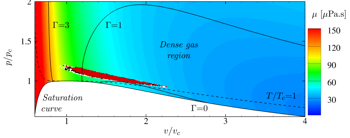
(b) Influence of Reynolds number on the distribution of p - v states for a slice at y^* \approx 10 and M_B = 3 : ● Re_B = 3000 ; ● Re_B = 7000 ; ○ Re_B = 12000 . The background colourmap shows isocontours of the viscosity.
