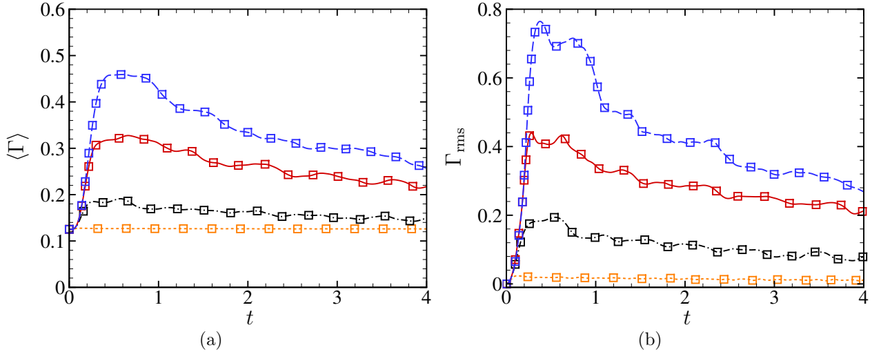
Figure 4.17. Time history of the average (a) and r.m.s. (b) fundamental derivative of gas dynamics at various M_{t_0} . ---: M_{t_0} = 0.2 ; -.-.-: M_{t_0} = 0.5 ; —: M_{t_0} = 0.8 ; ---: M_{t_0} = 1 . \Delta : Air; \square : PP11-MAH.
