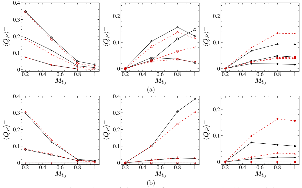
Figure 4.27. Fractional contribution of the various flow structures to the dilatational dissipation \langle Q_P \rangle^+ (a) and \langle Q_P \rangle^- (b) at various M_{t_0} ( t = 2 ). Left column: incompressible structures; central column: compressed structures; right column: expanding structures. —: Air; - - - : PP11-MAH-IC1. +, EI; ×, CI; ◇, SI; □, EC; ○, CC; △, SC; ■, EE; ●, CE; ▲, SE.
