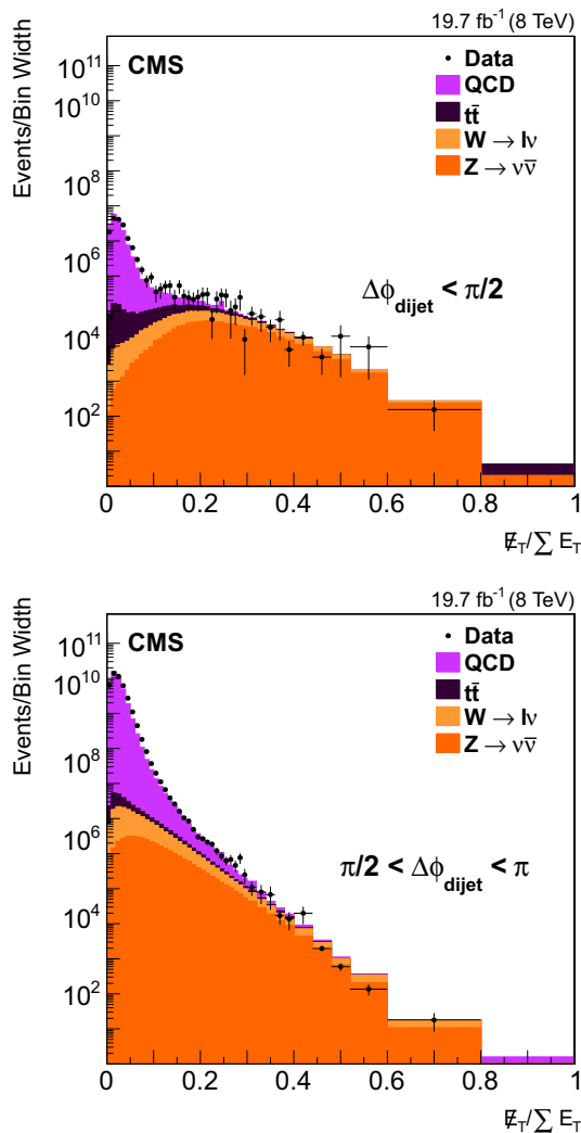
Fig. 1 Distribution of E_T / \sum E_T for data (points) in comparison with simulated jet production and other processes with large E_T (stacked) separately for the two regions \Delta\phi_{dijet} < \pi/2 (top) and \pi/2 < \Delta\phi_{dijet} < \pi (bottom). The main contribution of events with large E_T in the final state is caused by processes such as Z/W + \text{jet(s)} with Z \rightarrow \nu\bar{\nu} and W \rightarrow \ell\nu
