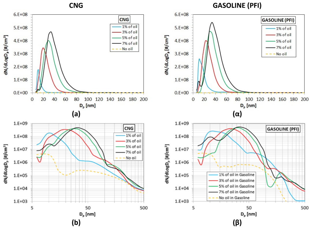
6 Figure 7 PSD functions (mean values) with a mass lubricant oil content equal to 0% (yellow line), 1% (light blue line), 7 3% (red line), 5% (green line) and 7% (black line), for both the CNG (Latin characters) and gasoline (Greek characters) 8 PFI tests. For clarity, the data are plotted by using both a linear (a) and ( \alpha ), and a logarithmic scale (b) and ( \beta ).
