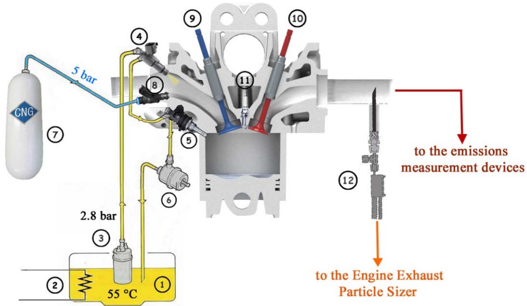
12 13 14 Figure 1. Experimental Set-up for the CNG tests. (1) Oil tank; (2) resistors for heating the oil to 55 °C; (3) oil pump; (4) 15 3-hole commercial low pressure injector; (5) 6-hole commercial high-pressure injector; (6) oil pressure regulator; (7) 16 CNG bottle; (8) CNG 1-hole injector; (9) intake and (10) exhaust valves; (11) spark-plug; (12) particle sizer probe. 17 18 19 20 21 22
