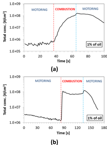
26 Figure 3 Total PN concentration measurements for CNG test with 1% of oil without (a) and with (b) “film-strategy”. 27 Red dashed line: start of combustion; light blue dashed line: end of combustion.
