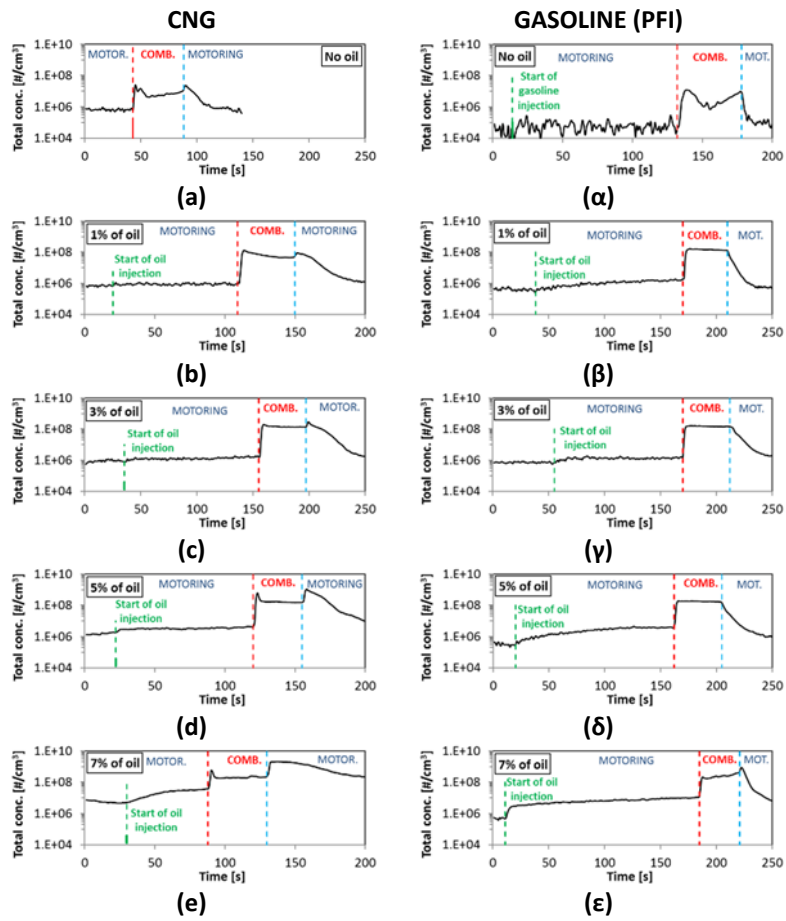
11 Figure 5 Total concentration number trace evolution with time of one representative case for each explored operating 12 condition, for both the CNG (Latin characters) and gasoline (Greek characters) PFI tests. Green dashed line: start of oil 13 injection into the intake manifold; red dashed line: start of combustion; light blue dashed line: end of combustion. 14
