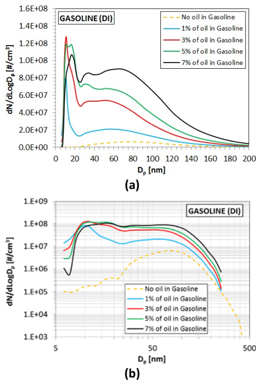
15 Figure 10 PSD functions (mean values) with mass lubricant oil content equal to 0% (yellow line), 1% (light blue line), 16 3% (red line), 5% (green line) and 7% (black line). For clarity, the data are plotted by using both a linear (a) and a 17 logarithmic scale (b).
