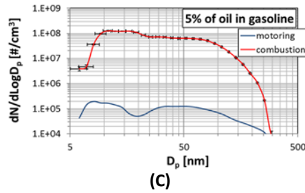
1 Figure 9 Statistical PSD functions (a), total concentration number trace evolution with time (b) and PSD functions 2 during motoring conditions and combustion (c) of one representative case (5% of oil) for gasoline DI tests.
