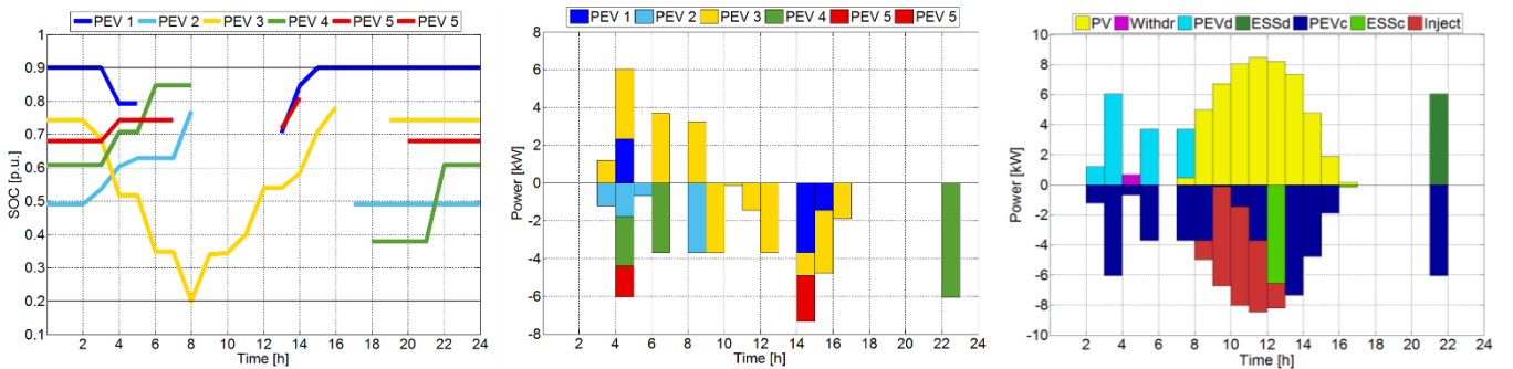
Figure 3.23. Trends of PEV energy content (left), PEV power (middle) and EVSI electric balance (right) in the maximum f(\mathbf{x}) case in a summer working day.
