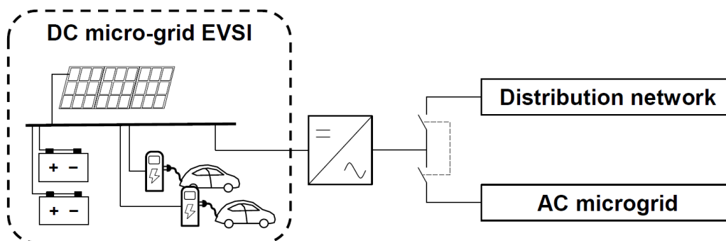
Figure 3.29. DC micro-grid EVSI structure in CONNECT Project.
