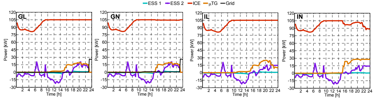
Figure 1.6. Electric power production in winter day in the four cases.
