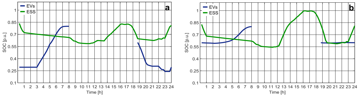
Figure 3.8. Storage state-of-charge of Residential user with f_1(\mathbf{x}) objective (a) and f_2(\mathbf{x}) objective (b).
