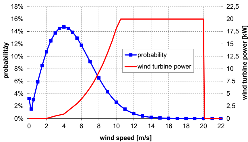
Figure 3.15. Wind Weibull distribution and wind turbine power.
