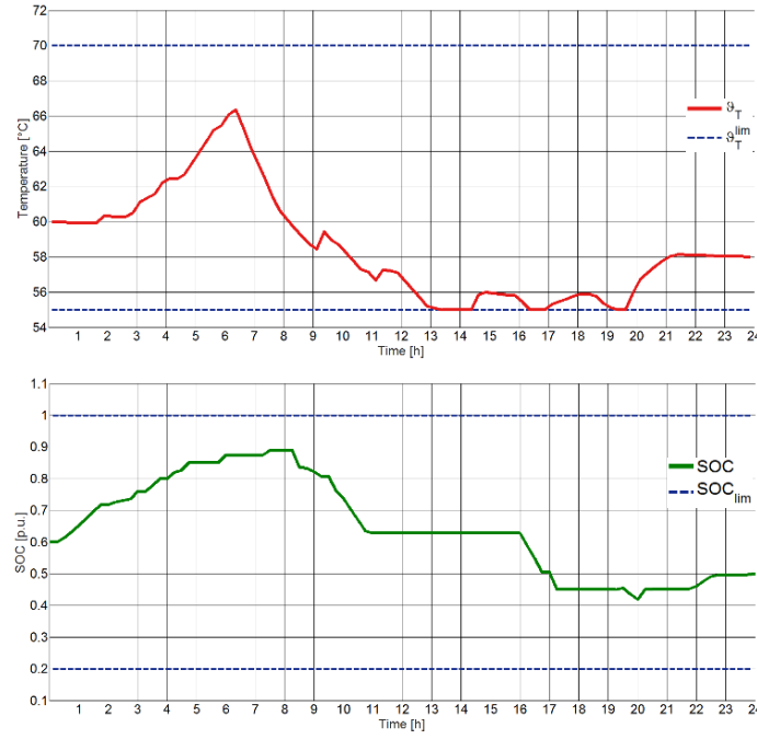
Figure 2.4 TSS temperature (upper) and ESS State Of Charge – SOC (lower) in Day 1 Case D.
