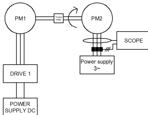
fig. 70: Slip-test setup
