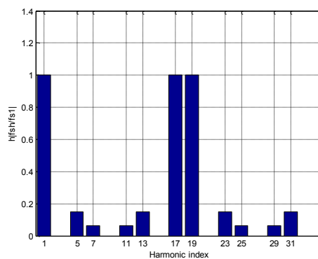
fig. 20: Normalized harmonic content of stator MMF
