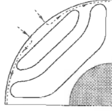
fig. 22: Leakage flux and its path through ribs
