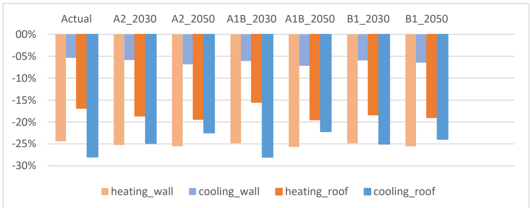
Figure 5.4-3 Yearly heating and cooling consumption of type referring to improved roof or wall
