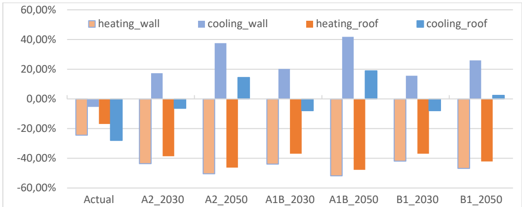
Figure 5.4-4 Yearly heating and cooling consumption variation of type referring to improved roof or wall and actual climate
