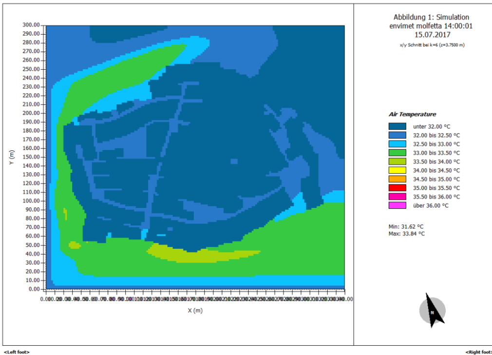
Figure 5.3-8 Horizontally variation of maximum temperatures simulated
