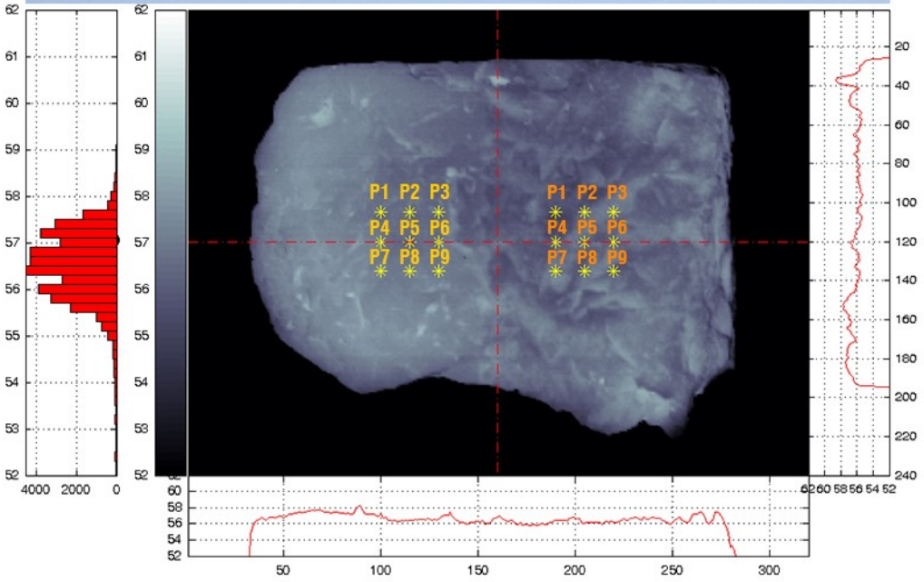
Figure Ann.A.2 Visible and thermal images of samples during the emissivity test and points of evaluation for black (yellow) and natural (orange) surfaces.
