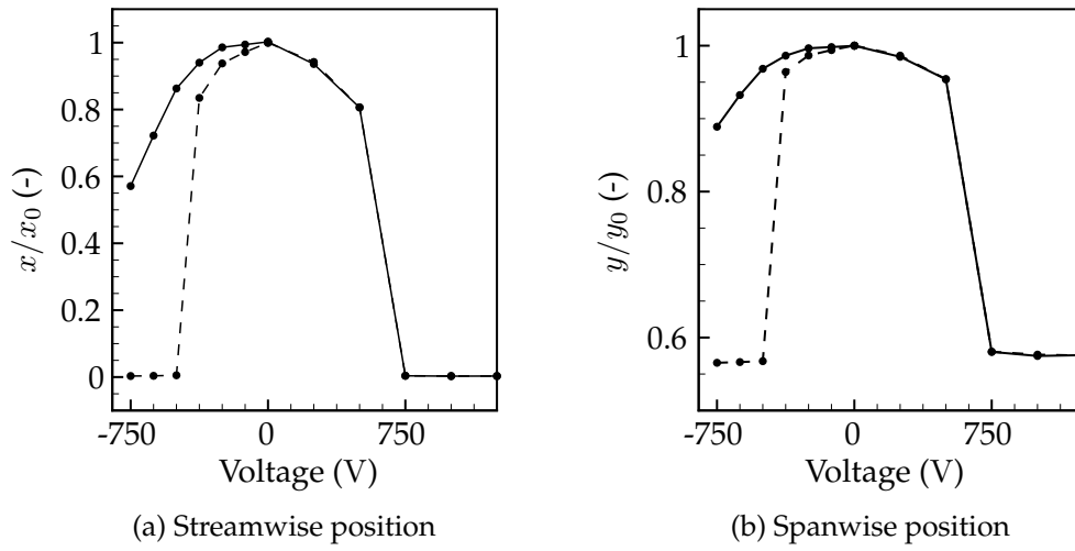
FIGURE 5.6: Flame-tip steady position in the streamwise and spanwise directions expressed as fraction of the reference position for mechanism "A" (—•—) and mechanism "B" (-•-).
