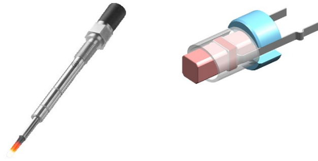
Figure 2.3 Glow Plug Combustion Pressure Sensor (left) and detail of the sensing element. [2]
