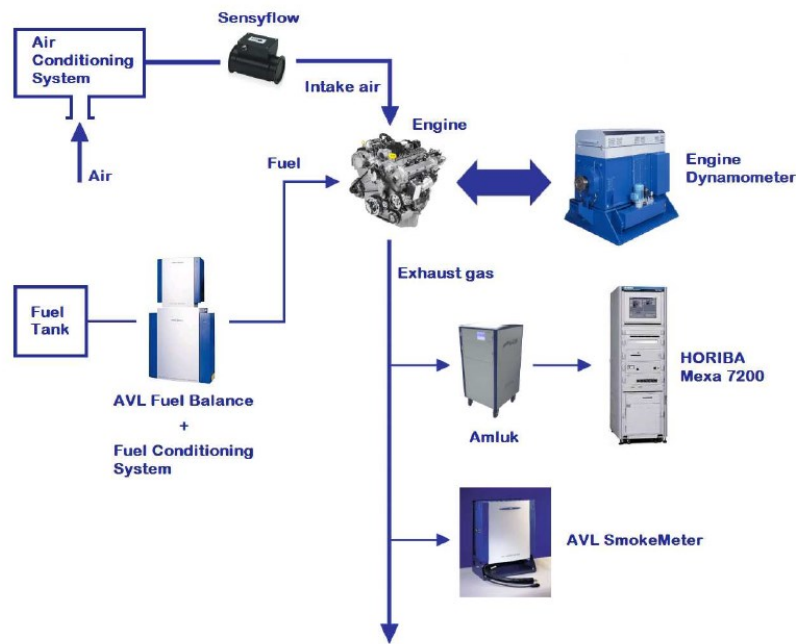
Figure 2.1 Test Bench layout
