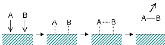
Figure 7.4 Langmuir-Hinshelwood mechanism
