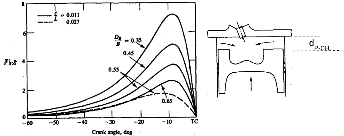
Figure 5.5 On the right, squish motions, coupled with piston stroke, are represented. On the left, theoretical squish velocity divided by mean piston speed is represented [9]
