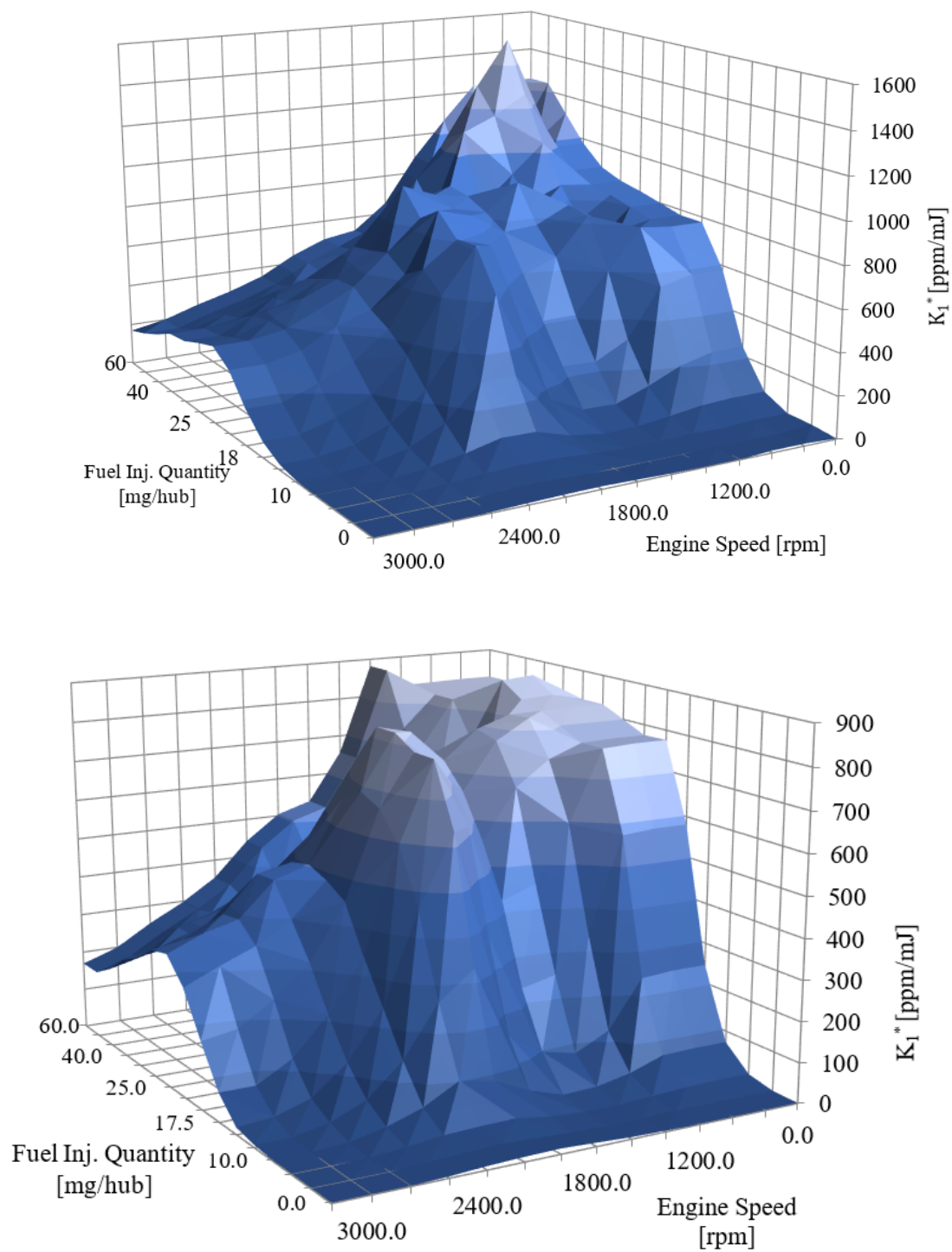
Figure 5.18 K_1' map before (a) and after (b) K_3 limitation
