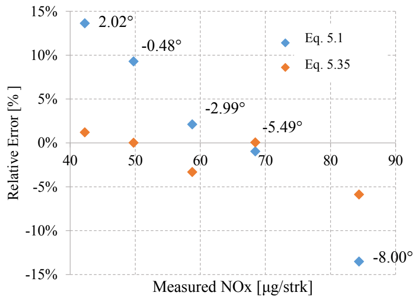
Figure 5.6 Comparison between base and improved model; labels are main injection timing in ^{\circ}\text{CAD BTDC} .
