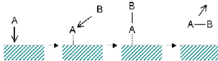
Figure 7.5 Eley-Rideal mechanism
