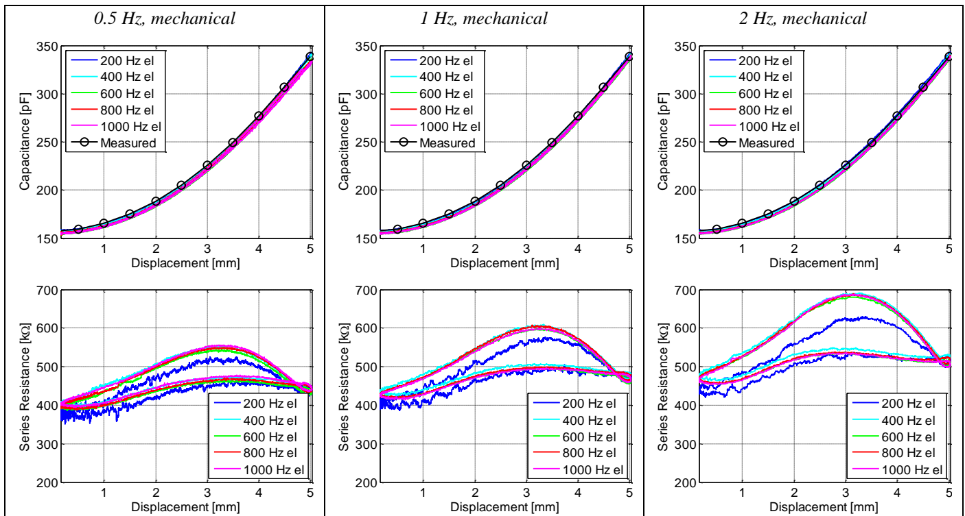
Fig. 10. DEA membrane capacitance and series resistance estimations using 100 V sinusoidal signals at different electrical frequencies (200, 400, 600, 800, 1000 Hz), and deforming the DEA by 5 mm at different mechanical frequencies (0.5, 1, 2 Hz) with an external actuator.
