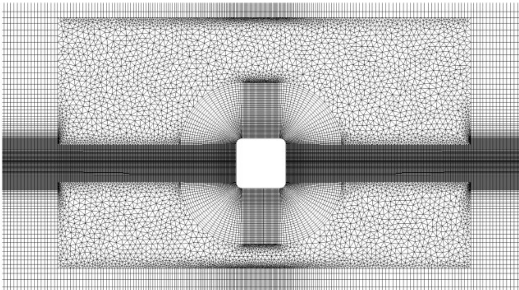
Fig. 8-3: Enlargement of the fine-mesh (156,000 cells)
