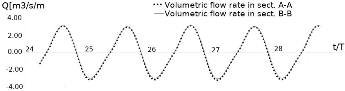
Fig. 7.2-8 Comparison between the volumetric flow rate measured in sections (A-A) and (B-B), shown in Fig. 6.2-6.
