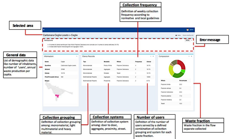
Figure 26-Web-App: planning collection service interface
