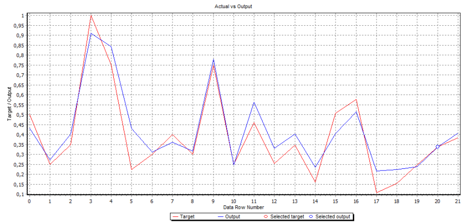
Figure 20- Actual vs. forecast in case of Pl_w value prediction
