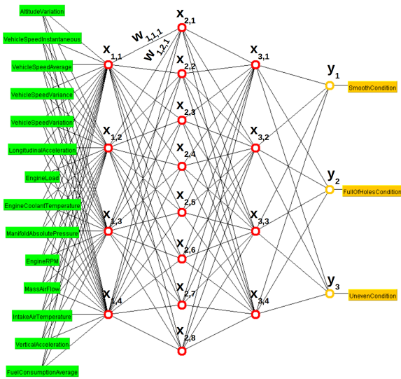
Fig. 10. Example of model for Multilayer Perceptron classifier
