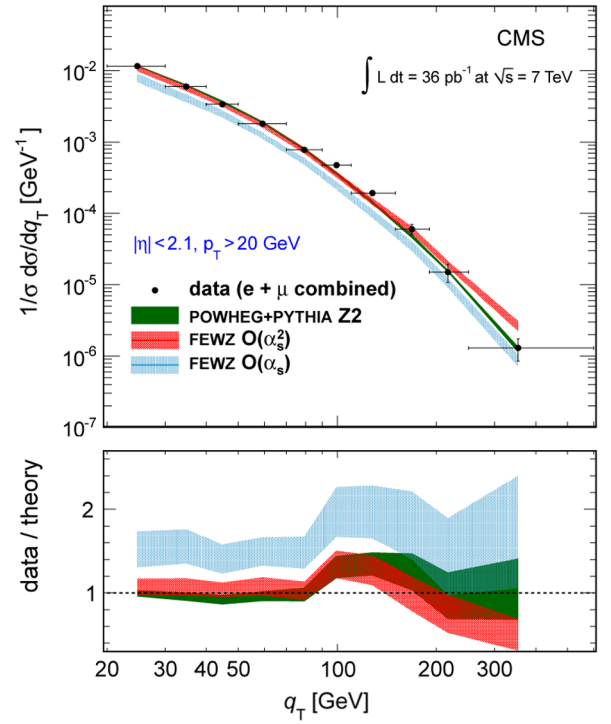
FIG. 8 (color online). The combined electron and muon Z-boson normalized differential cross section as a function of transverse-momentum (points) and the POWHEG and FEWZ predictions for q_T > 20 GeV. The horizontal error bars indicate the bin boundaries and the data points are positioned at the center-of-gravity of the bins based on the POWHEG prediction. The bands in the upper plot represent the uncertainty on the predictions from factorization and renormalization scales and PDFs. The lower plot shows the ratio between the data and the theory predictions. The bands in the lower plot represent the 1 standard deviation combined theoretical and experimental uncertainties.
