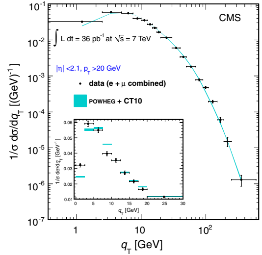
FIG. 6 (color online). The Z-boson transverse-momentum distribution found from combining the muon and electron channels, compared to the predictions of the POWHEG generator interfaced with PYTHIA using the Z2 tune. The error bars correspond to the statistical and systematic uncertainties added in quadrature. The band around the theoretical prediction includes the uncertainties due to scale variations and PDFs. The horizontal error bars indicate the bin boundaries, and the data points are positioned at the center-of-gravity of the bins, based on the POWHEG prediction. The inset figure shows the low q_T region on a linear scale.
