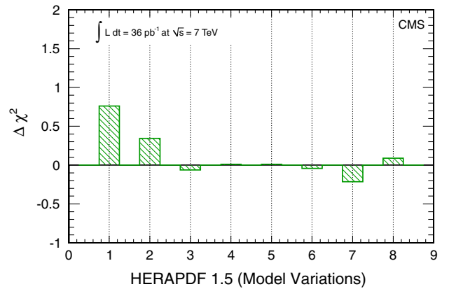
FIG. 5 (color online). The change in \chi^2 when comparing the Z rapidity differential cross section measurement with the predictions of the NLO HERAPDF 1.5 PDF set as each of the eigenvector input parameters (left) and the model parameters (right) is varied by 1 standard deviation around its default value. These together represent the full set of uncertainties in the HERAPDF 1.5 set.
