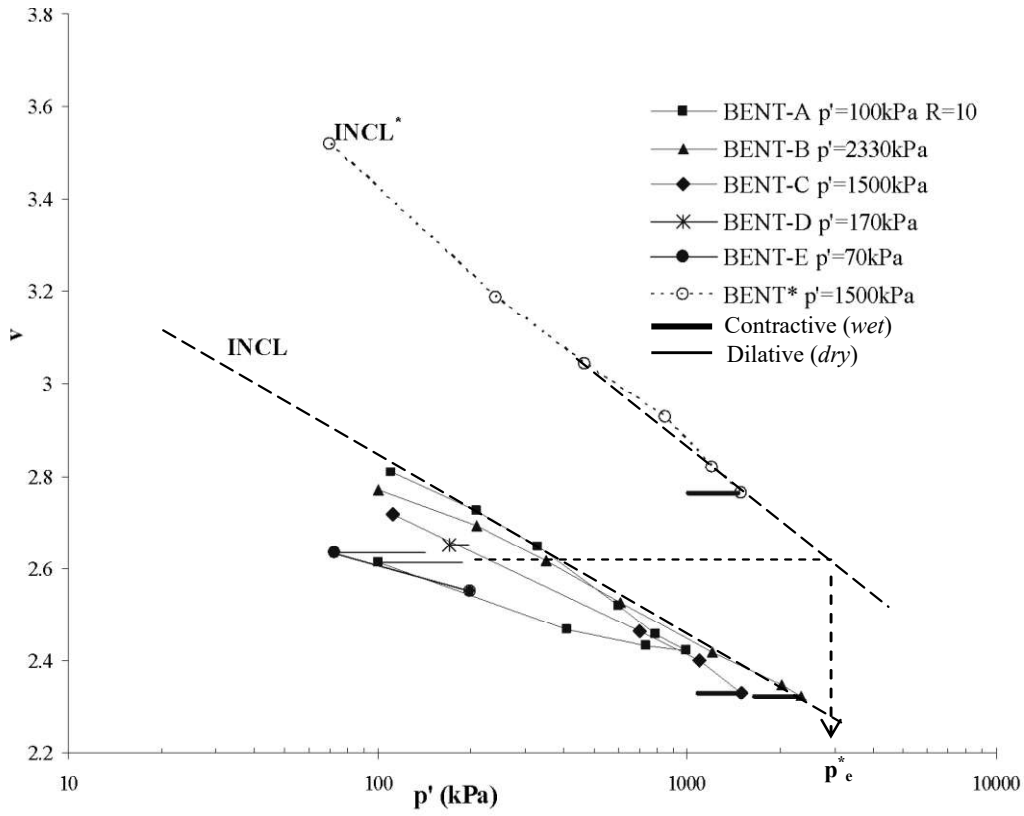
Fig. 10 Natural and reconstituted BENT: isotropic compression and undrained shear state paths.
