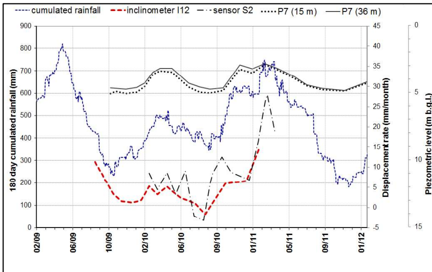
Fig. 19 Displacement rates at 19 m depth down inclinometer I12 and at ground surface (GPS sensor S2); piezometric levels at 15 m and 36 m b.g.l. down borehole P7 and 180 day cumulated rainfall (the location of the monitoring points in Fig. 5).
