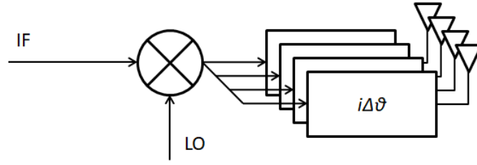
Figure 1.5 – RF phase shifting architecture block diagram
