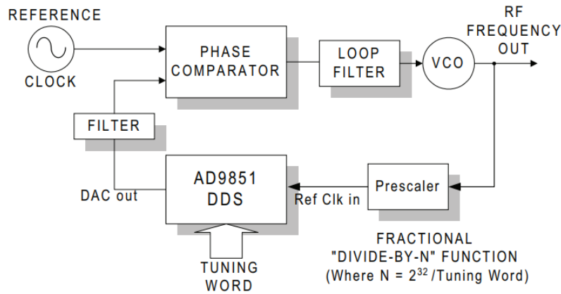
Figure 2.8 – DDS in the feedback path of the PLL acting as a fractional divide-by-N stage
