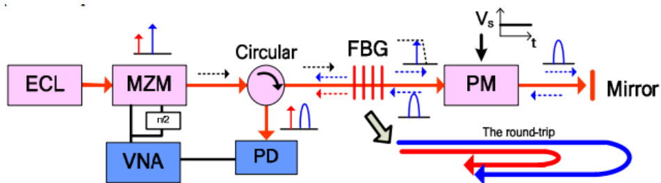
Figure 1.11 - Schematic diagram of the photonic microwave phase shifter
