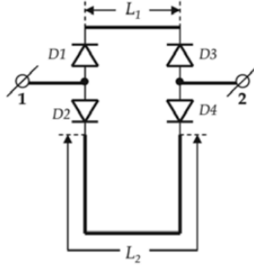
Figure 1.6 – Conventional switched-line phase shift block based on PIN diodes
