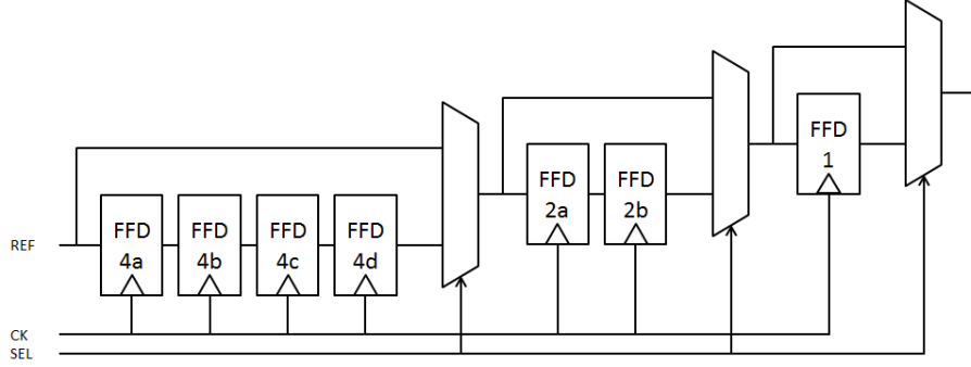
Figure 3.1 – Three shift registers chained into a SDL with programmable length ( k equal to 2, 1 and 0)
