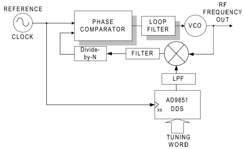
Figure 2.9 – DDS as an offset frequency generator in an offset-PLL
