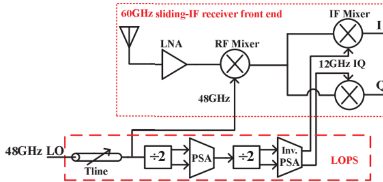
Figure 1.17 – Block diagram of the 60 GHz LO-phase shifting receiver front-end
