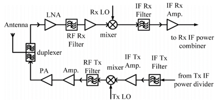
Figure 2.13 – Block diagram of the transceiver architecture assigned to each antenna
