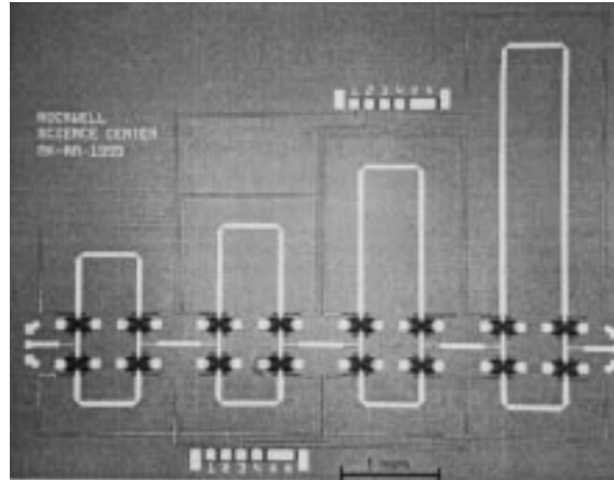
Figure 1.10 - Photograph of the four-bit RF MEMS TTD network
