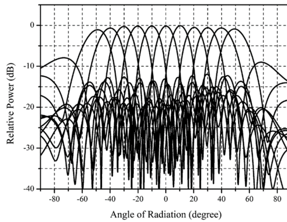
Figure 2.14 – Simulated radiation patterns for 11 equally spaced angle of radiations
