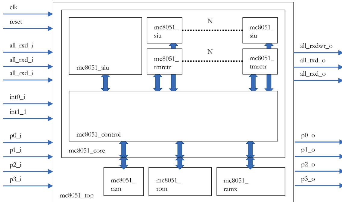
Figure 3.7 – 8051 architecture implemented by Oregano Systems
