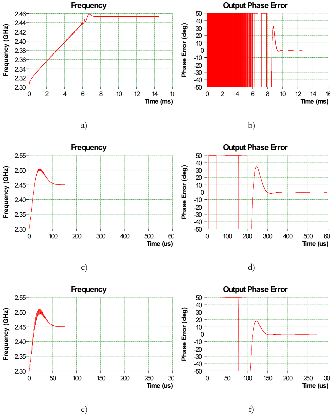
Figure 3.11 – Transient analysis of output frequency and phase error for various LBWs (1-kHz, 10-kHz, 20-kHz)
