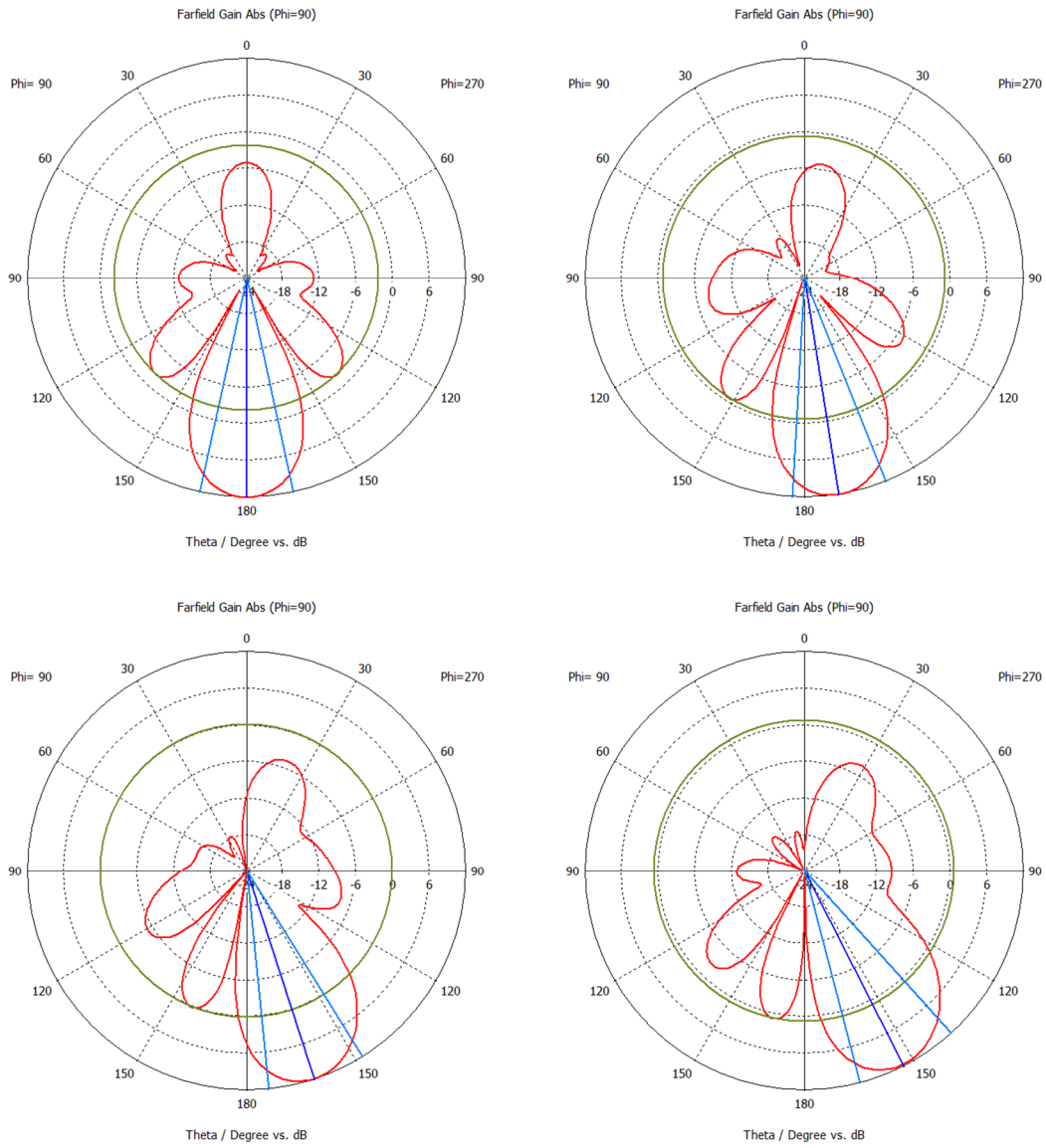
Figure 4.13 – Radiation pattern in the YZ-cut for a set of four different values of \Delta\varphi ( 0^\circ , 30^\circ , 60^\circ , 90^\circ )
