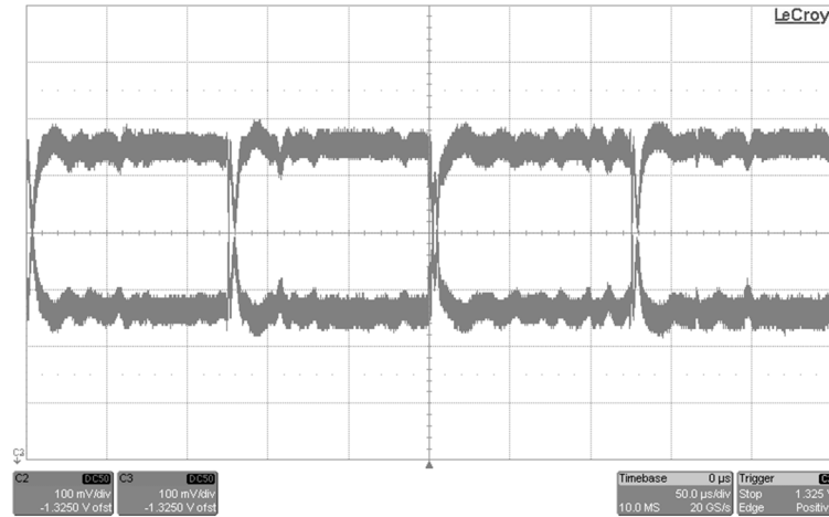
Figure 4.23 - Actual IQ signals for the signal transitions \alpha = 135^\circ and \alpha = 315^\circ
