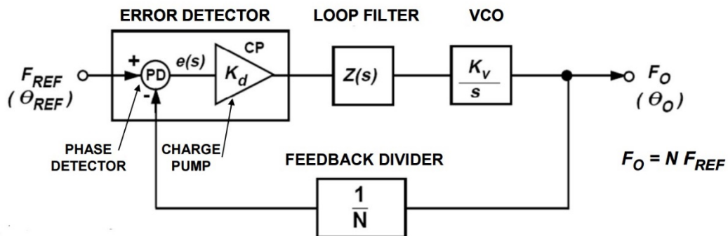
Figure 2.3 – Basic PLL block diagram
