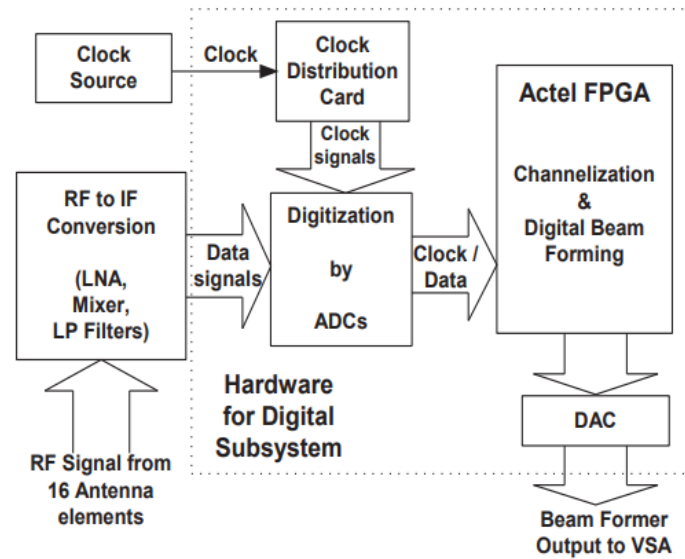
Figure 1.15 – Block diagram of the DBF system
