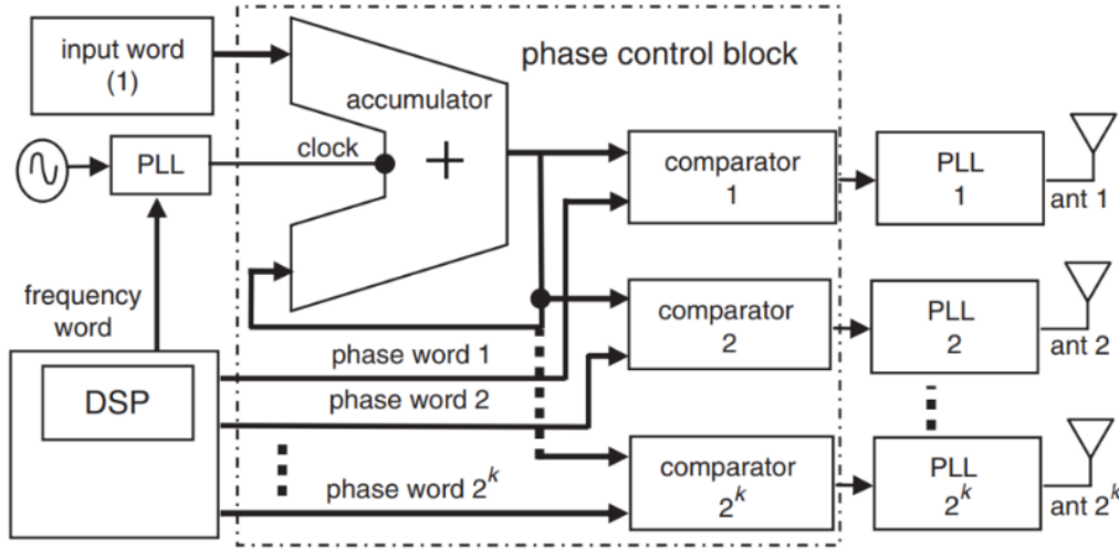
Figure 2.19 – Block diagram of the revised DDS-PLL architecture based on the accumulator register
