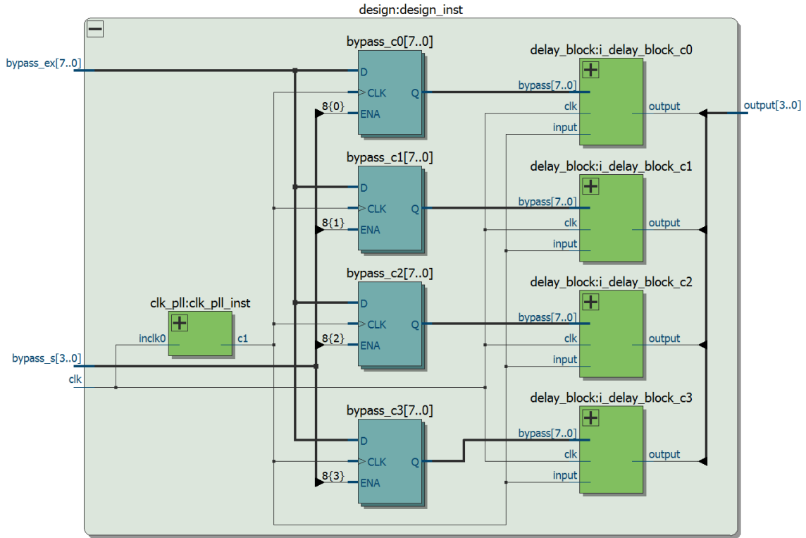
Figure 3.3 – RTL netlist view of the PCU entity
