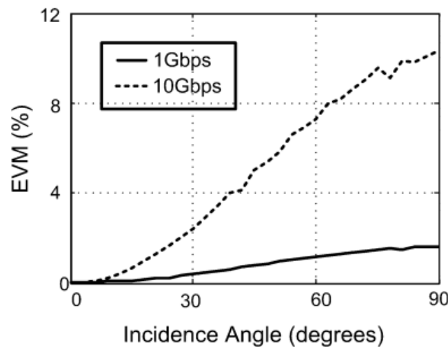
Figure 1.20 – EVM vs. incidence angle for two different signal bandwidths (750-MHz and 7.5-GHz)
