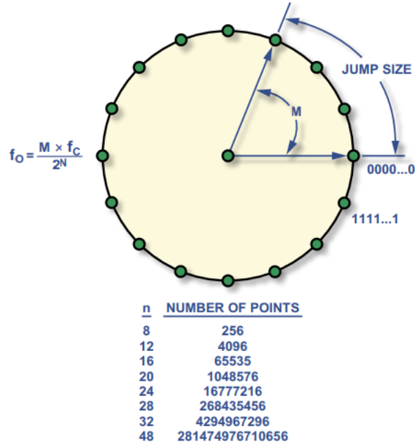
Figure 2.2 - Digital phase wheel graphical representation
