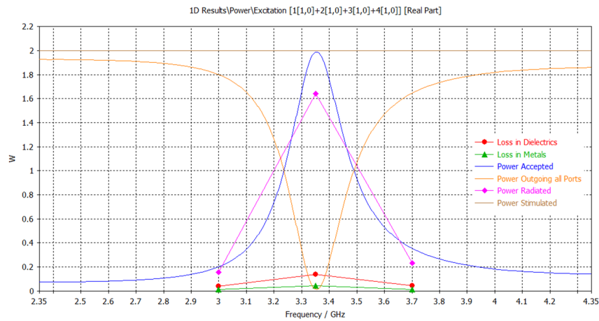
Figure 4.10 – Power accounting
