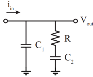
Figure 2.5 – Lead/lag filter schematic
