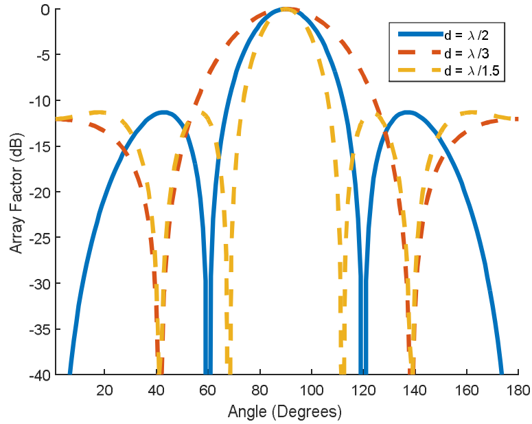
Figure 1.3 – Array factor of a 1-D linear phased array ( N=4 , \Phi_0=90^\circ ). d=\lambda/2 , \lambda/3 and \lambda/1.5
