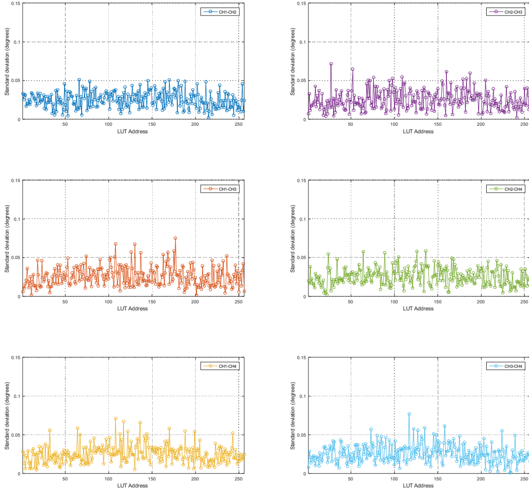
Figure 3.22 – LUT address vs. std. deviation for CH1-CH2, CH1-CH3, CH1-CH4 (LUTa =0 to LUTa =255)
