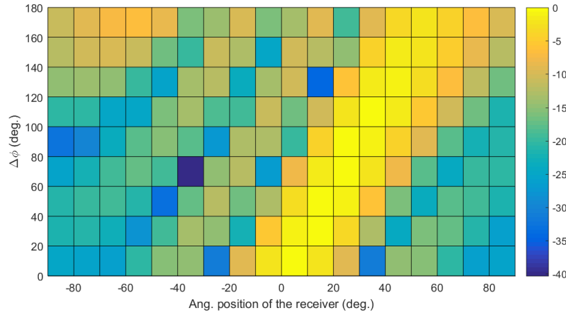
Figure 4.18 – Normalized RSS for various values of \Delta\phi and different angular positions of the receiver
