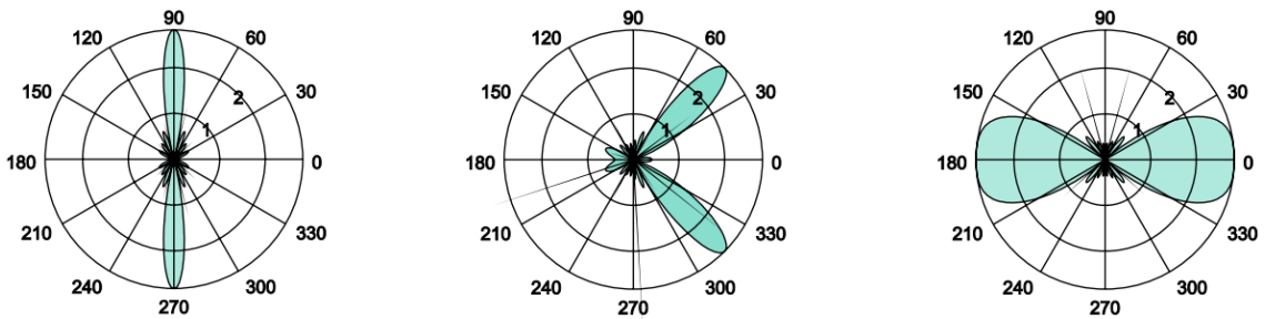
Figure 1.1 – Array factor of a 1-D linear phased array ( N=8 , d=\lambda/2 ). \Phi_0=90^\circ , 45^\circ and 0^\circ
