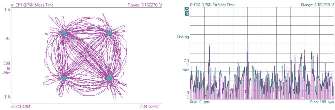
Figure 4.17 – QPSK constellation and EVM (200 symbols) at the receiver when transmitting broadside ( \Delta\phi = 0^\circ )
