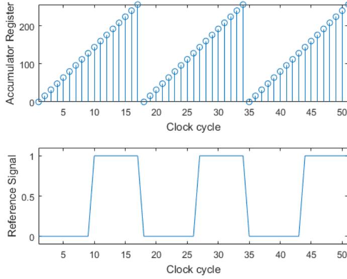
Figure 2.22 – Output of a 4-bit accumulator register and output of a comparator when phase word is 0000
