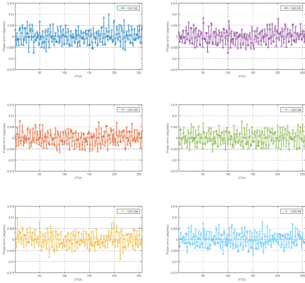
Figure 3.18 – PTW vs. phase error for CH3-CH4 (PTW=0 to PTW=255)
