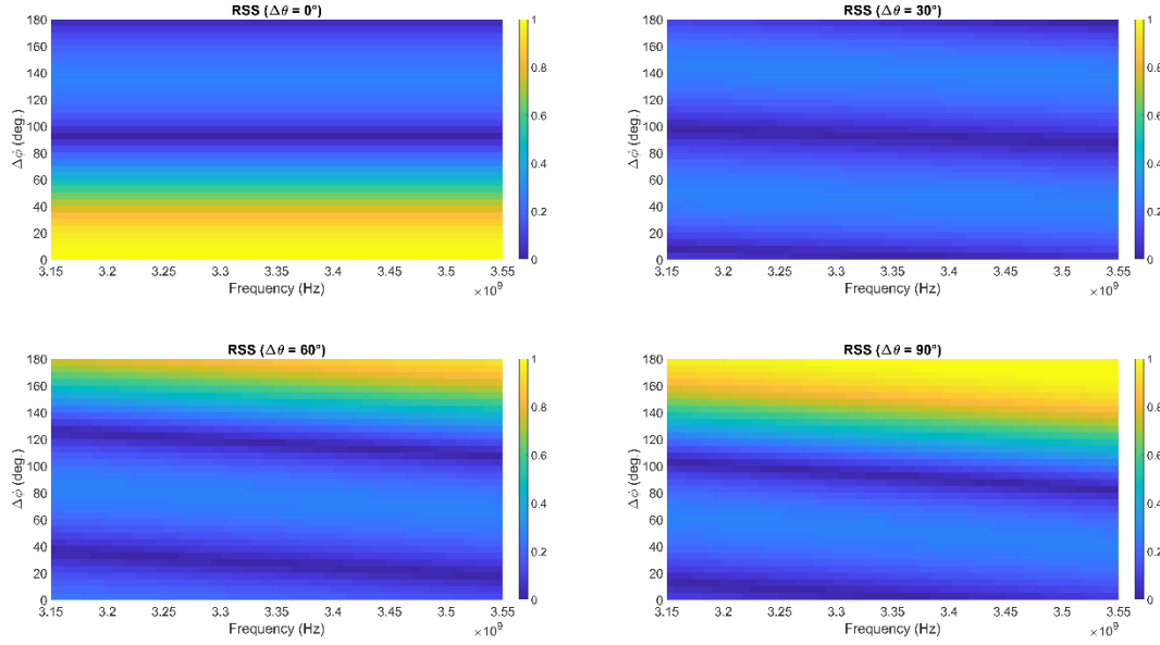
Figure 4.20 – Normalized RSS (linear scale) calculated for four angular positions of the receiver when the mutual phase shifts at the antennas is varied among various values
