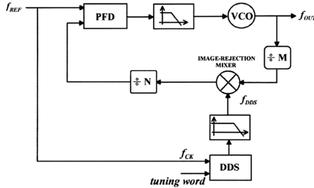
Figure 2.10 – DDS-based PLL for 2.4-GHz frequency synthesis
