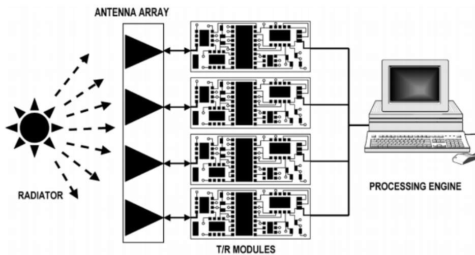
Figure 1.24 – Phased array system based on T/R modules
