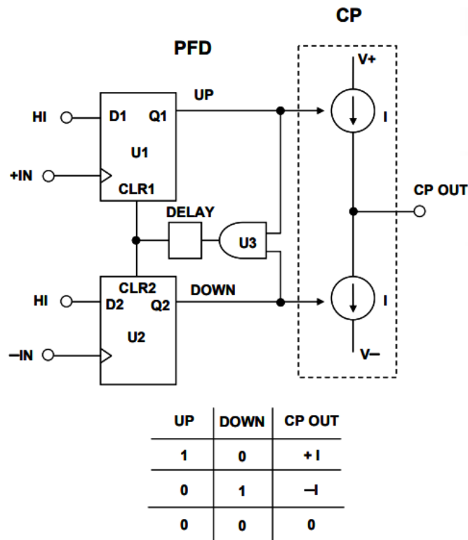
Figure 2.4 – Schematic diagram of the PFD driving the CP
