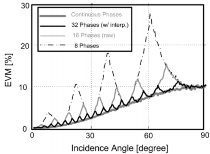
Figure 1.21 – EVM vs. incidence angle for 8 (3-bit), 16 (4-bit), 32 (5-bit) or continuous phase shifts available
