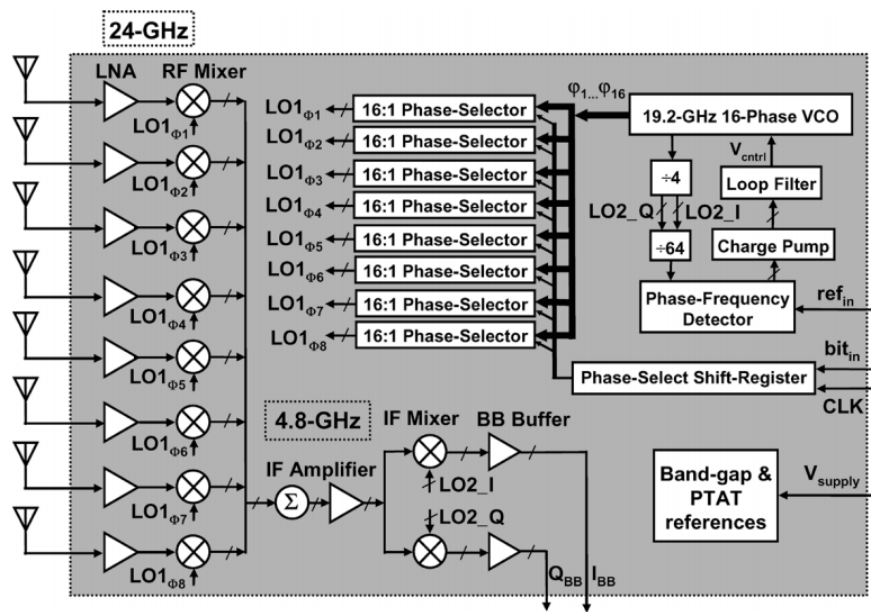
Figure 1.19 – Block diagram of the fully integrated 24-GHz phased-array receiver
