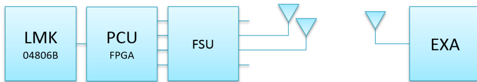
Figure 3.15 – Measurement setup diagram (frequency domain, FSU outputs – 2 channels)
