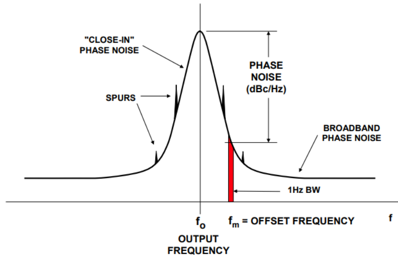
Figure 2.6 – Conceptual representation of noise and spurs in PLLs
