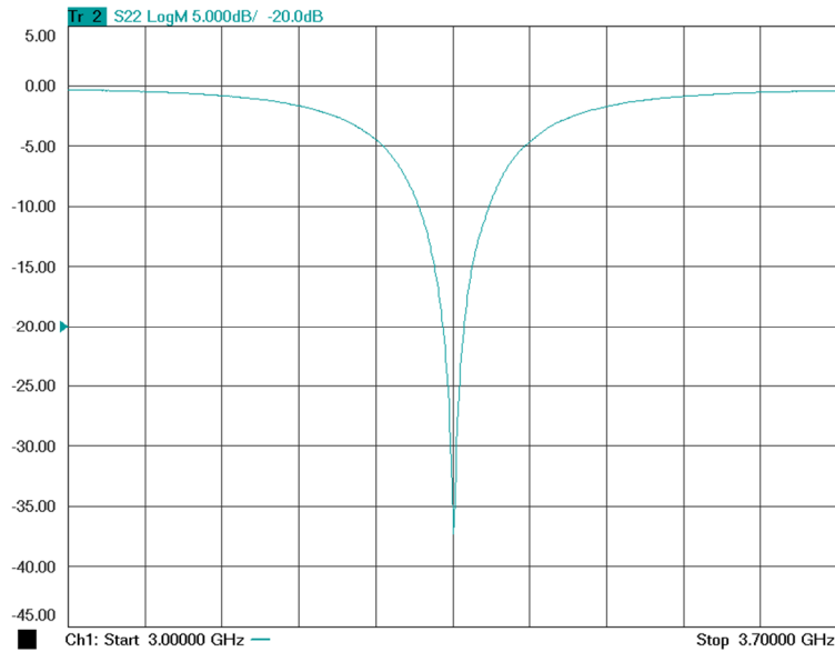
Figure 4.16 – Reflection coefficient at input port (dB)
