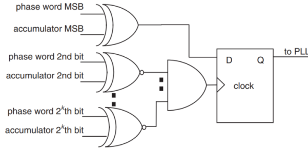
Figure 2.20 – Circuit diagram of the implemented comparators
