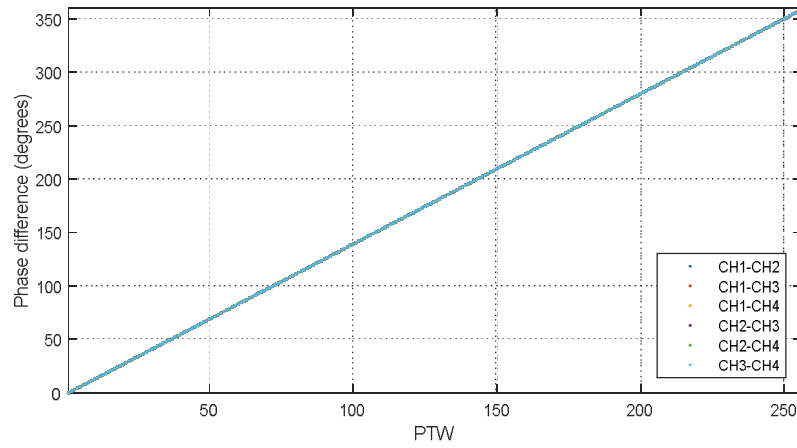
Figure 3.17 – PTW vs. phase difference trans-characteristic (PTW=0 to PTW=255)
