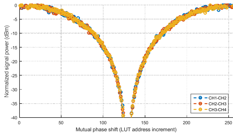
Figure 3.23 – Mutual phase shift vs. normalized power (LUTa=0 to LUTa =255)
