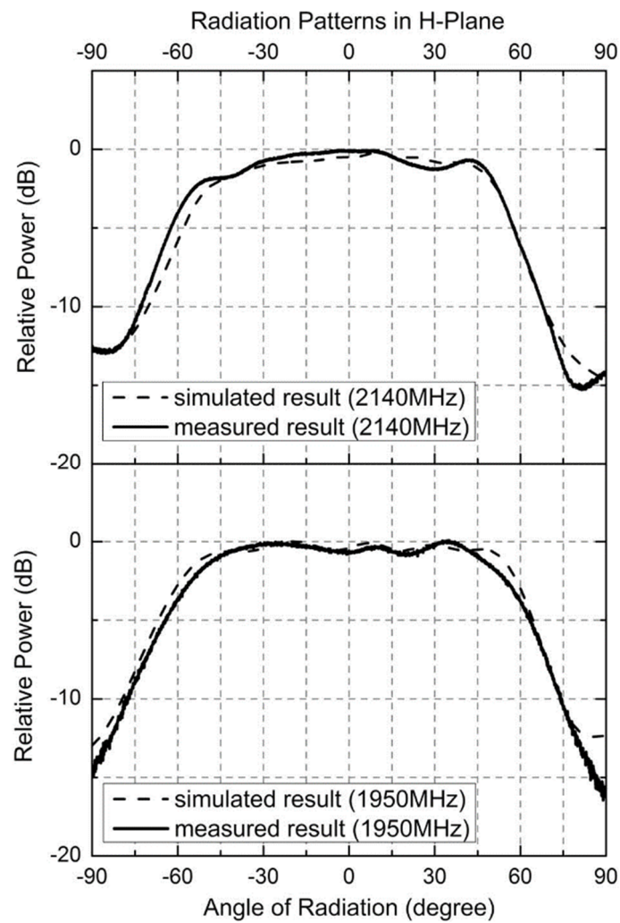
Figure 2.15 – Simulated radiation patterns of the antenna elements employed in the phased array
