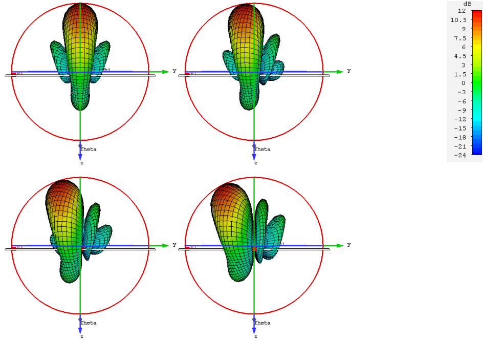
Figure 4.7 – 3D reconstruction of the radiation pattern for a set of four different values of \Delta\varphi ( 0^\circ , 30^\circ , 60^\circ , 90^\circ )
