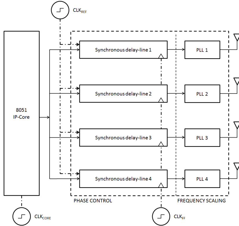
Figure 3.6 – Block diagram of the BSU
