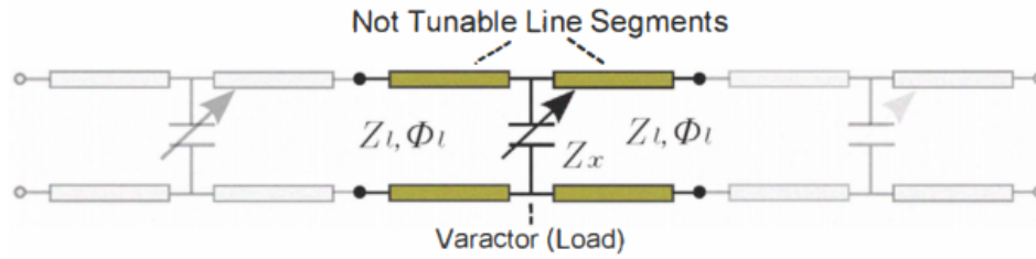
Figure 1.8 – Periodically loaded line with shunt LC based varactors
