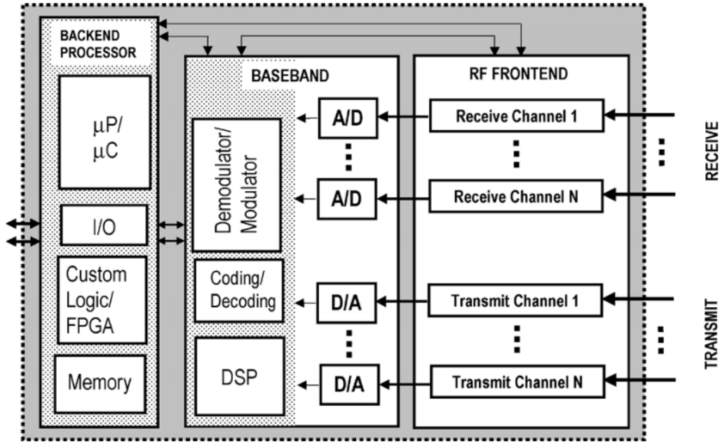
Figure 1.26 – Reference block diagram of a SoC architecture for phased arrays
