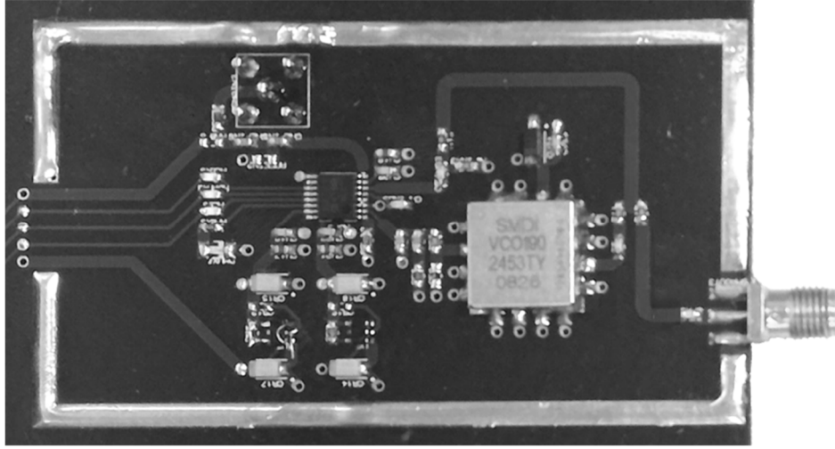
Figure 4.2 – LO synthesizers PCB (one channel)
