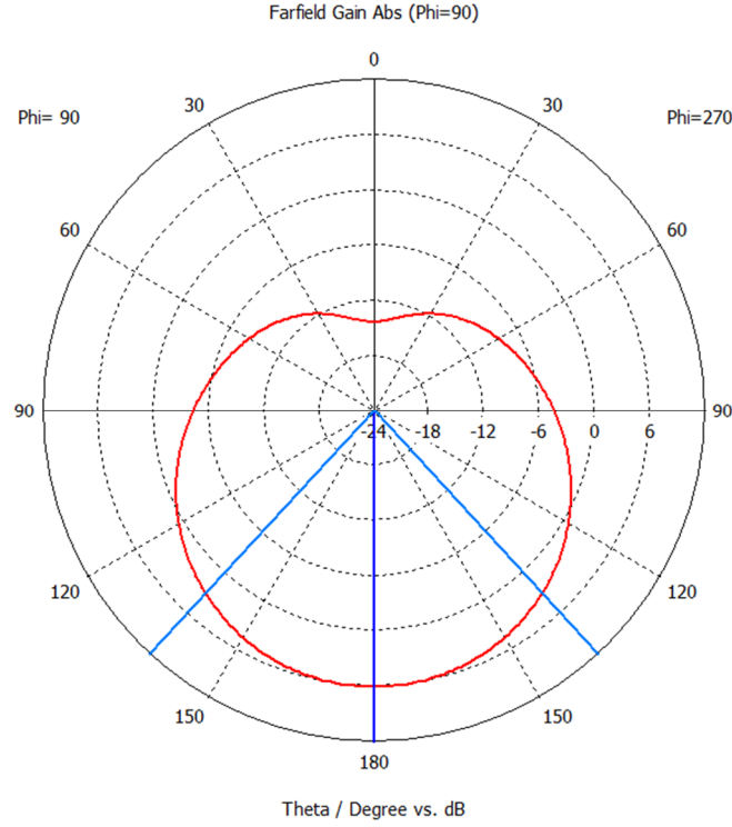
Figure 4.14 – Radiation pattern of the single antenna in the YZ-cut
