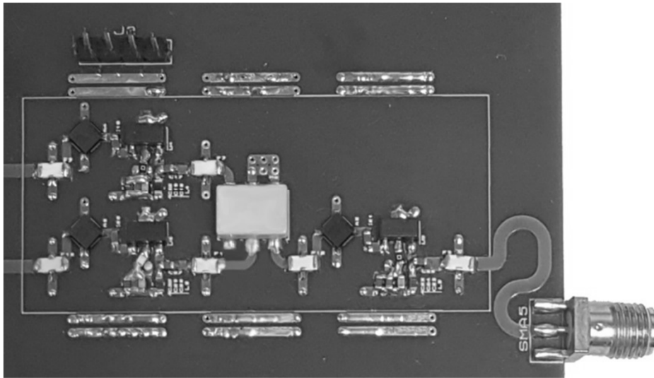
Figure 4.3 – Active up-conversion PCB (one channel)
