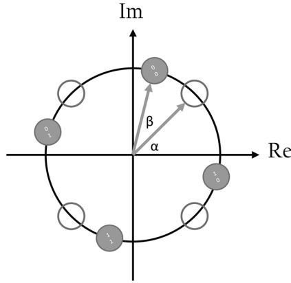
Figure 4.21 - IQ plane representation of \alpha (phase rotation assigned to the PSK symbol) and \beta (phase shift assigned for beam steering)
