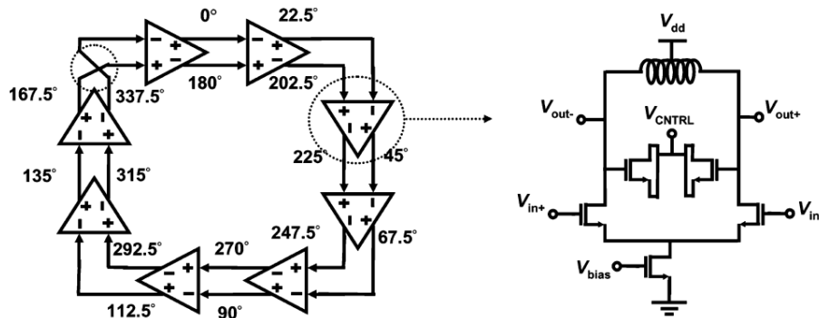
Figure 1.18 – Schematic diagram of the 16-phases 19.2-GHz CMOS ring VCO
