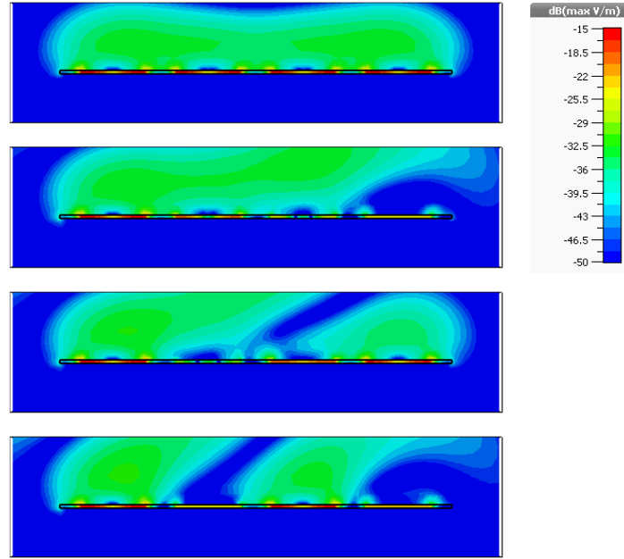
Figure 4.8 – Reconstruction of the electric field (absolute value) for a set of four different values of \Delta\varphi ( 0^\circ , 30^\circ , 60^\circ , 90^\circ ).
