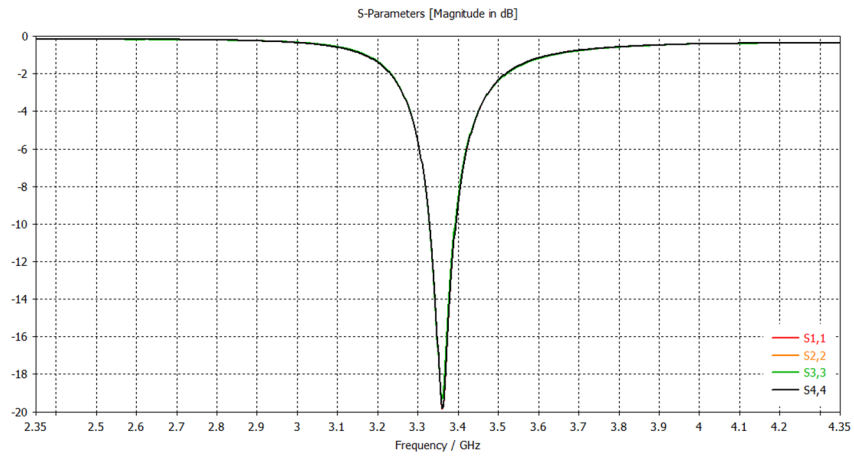
Figure 4.9 – Reflection coefficient at input ports (dB)
