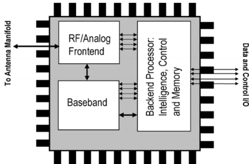
Figure 1.25 – High-level block diagram of a SoC architecture for phased arrays
