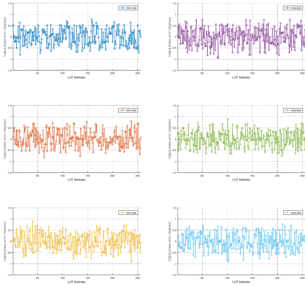
Figure 3.21 – LUT address vs. phase error for CH1-CH2 (LUTa =0 to LUTa =255)
