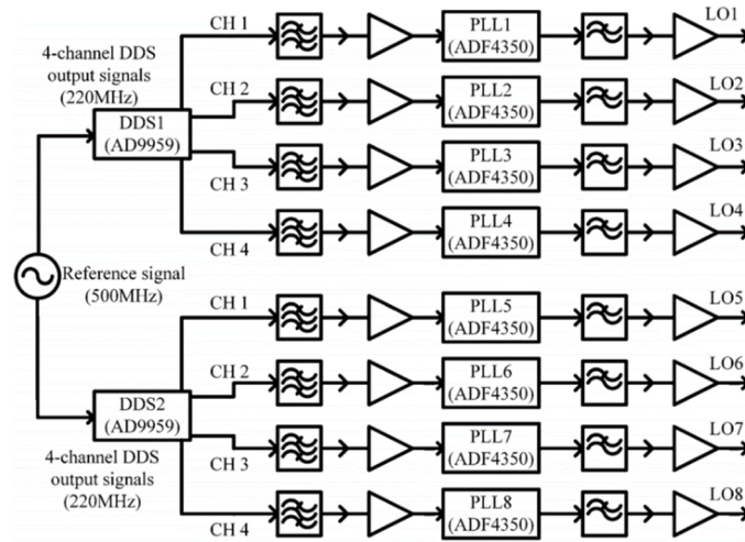
Figure 2.12 – System architecture of the proposed phased array
