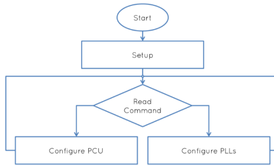
Figure 3.10 – High-level flow chart of the firmware code
