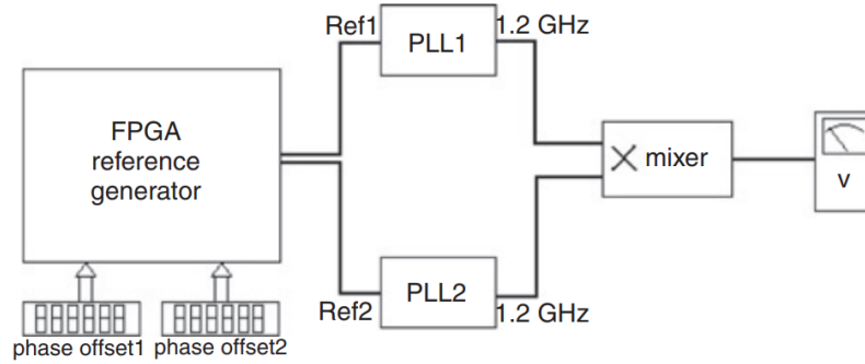
Figure 2.18 – Measurement setup for indirect quantification of phase shifts
