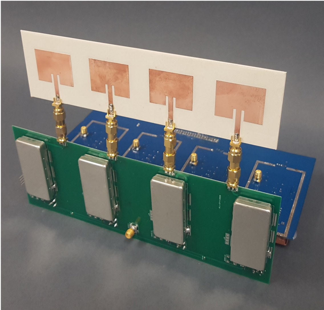
Figure 4.5 – Phased array transmitter prototype
