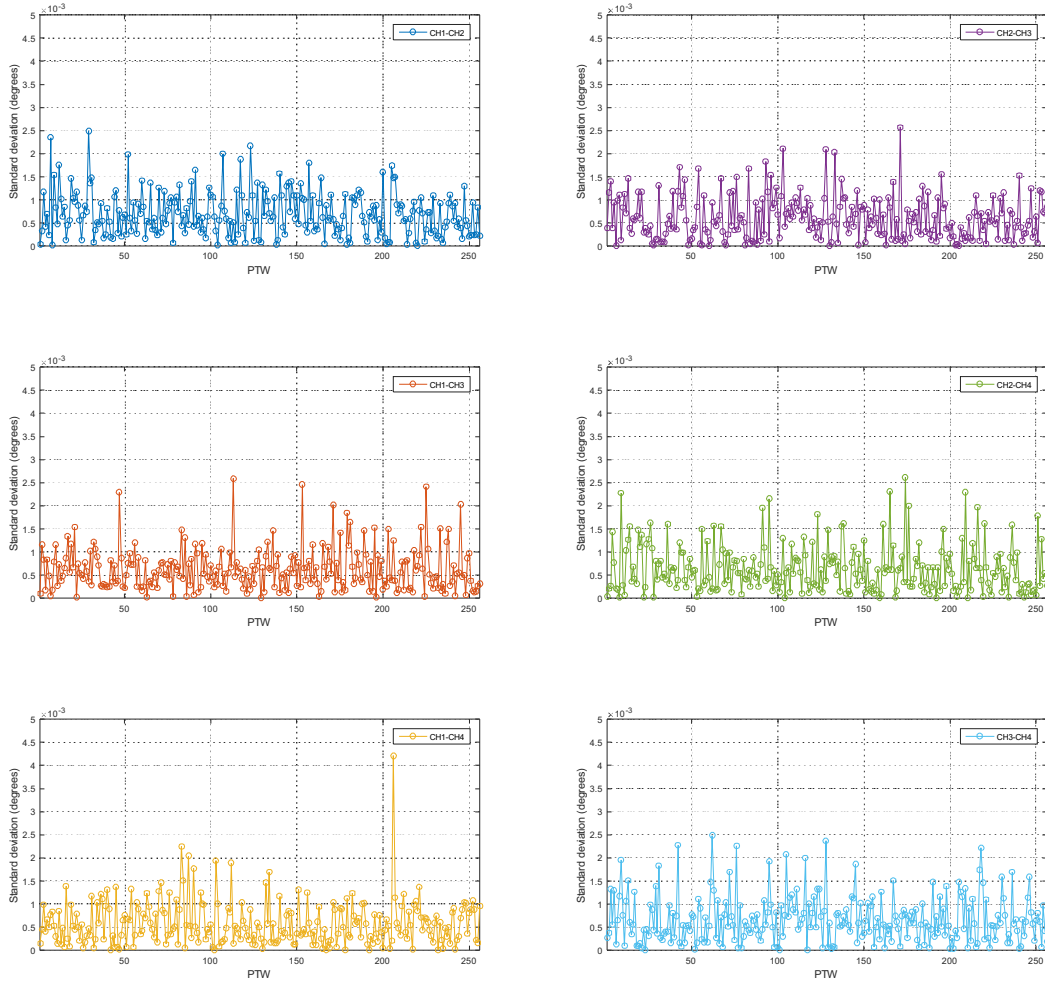
Figure 3.19 – PTW vs. standard deviation for CH1-CH2, CH1-CH3, CH1-CH4 (PTW=0 to PTW=255)
