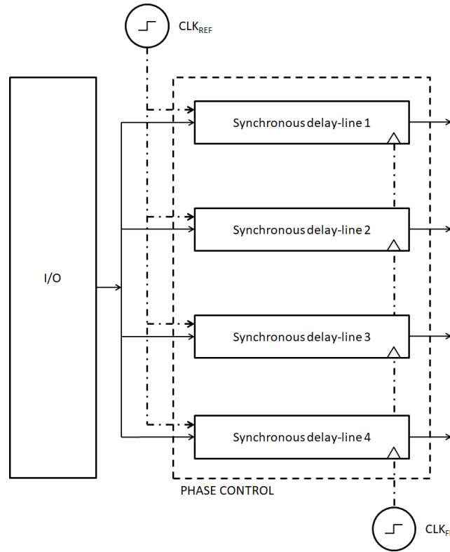
Figure 3.2 – Block diagram of a 4 channel PCU based on SDL with programmable lengths
