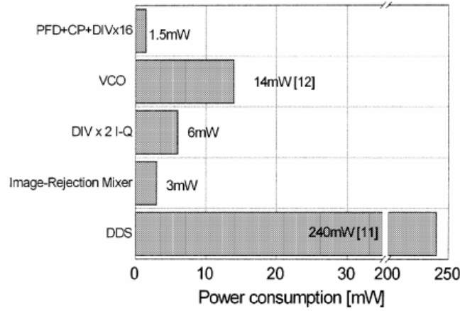
Figure 2.11 – Budgetary power consumption of the proposed DDS-PLL solution
