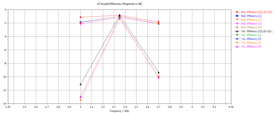
Figure 4.12 – Radiation efficiency of the single antennas and of the overall array
