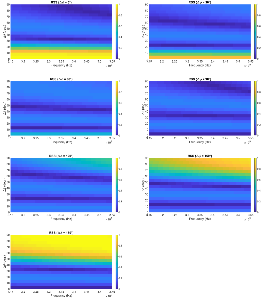
Figure 4.19 – Normalized RSS (linear scale) calculated for seven mutual phase shifts when the receiver is placed in various angular positions
