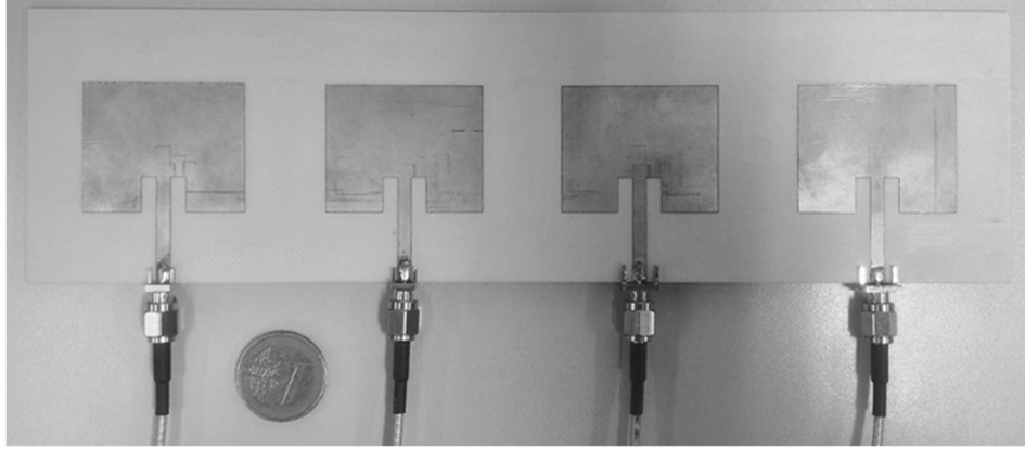
Figure 3.16 - Linear array of patch antennas connected to the outputs of the FSU
