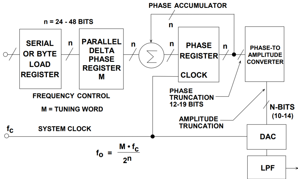
Figure 2.1 – Block diagram of a DDS
