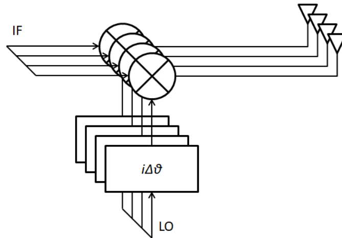
Figure 1.16 – LO phase shifting architecture block diagram
