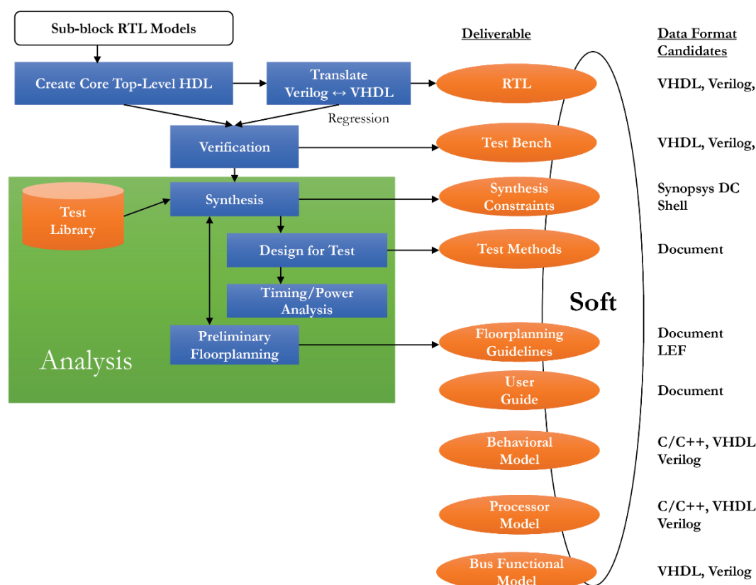
Figure A.0.3 – Design flow for soft IP cores
