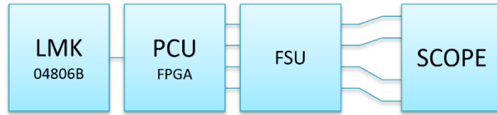
Figure 3.14 – Measurement setup diagram (time domain, FSU outputs)
