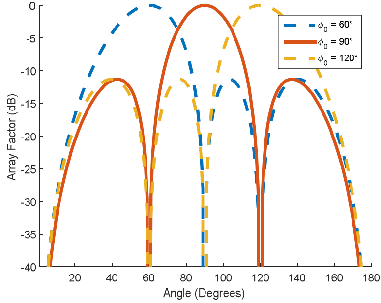
Figure 1.2 - Array factor of a 1-D linear phased array ( N=4 , d=\lambda/2 ). \Phi_0=60^\circ , 90^\circ and 120^\circ
