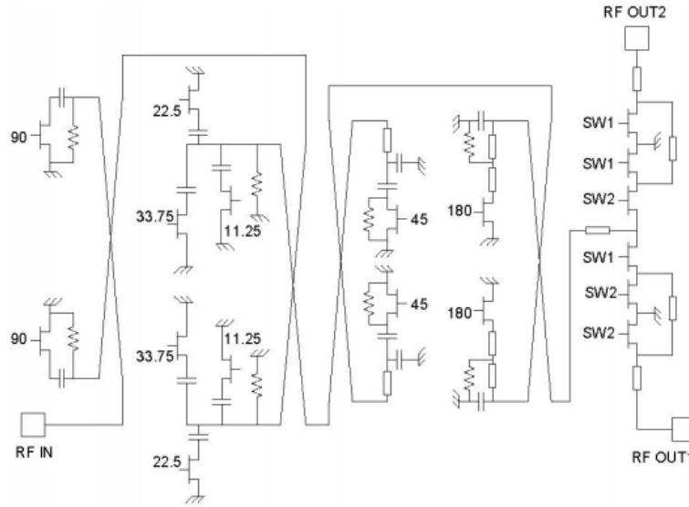
Figure 1.9 – Schematic diagram of the 5-bit phase shifter MMIC with SPDT switch
