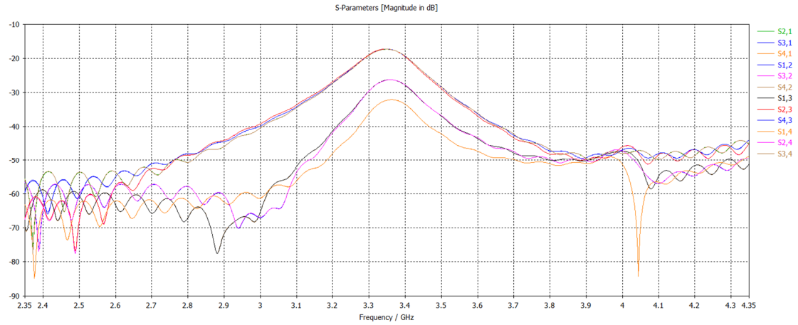
Figure 4.11 – Coupling among the four input ports (dB)
