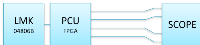
Figure 3.13 – Measurement setup diagram (time domain, PCU outputs)
