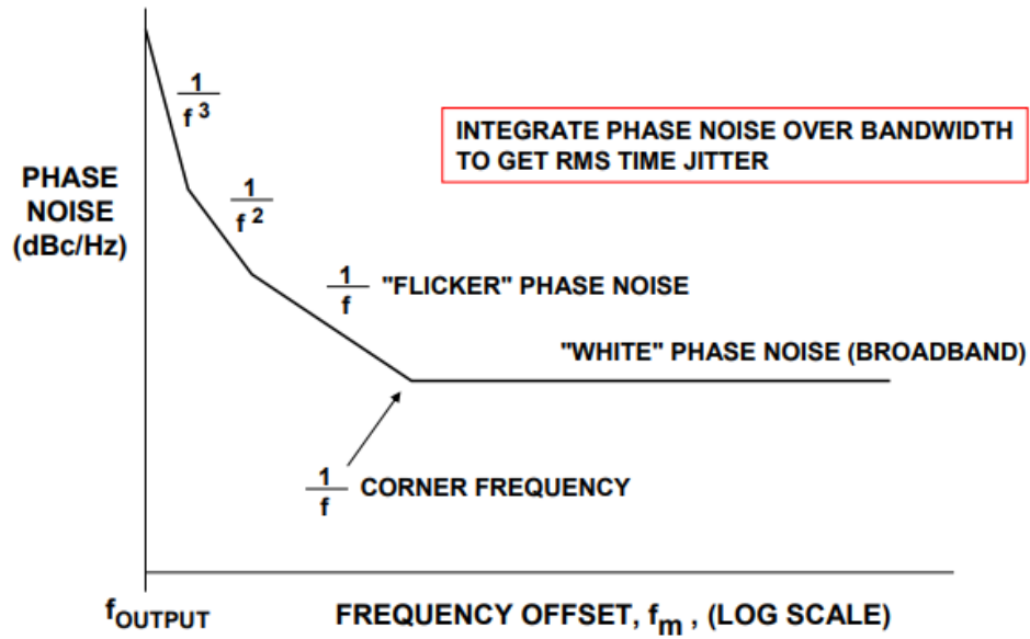
Figure 2.7 – Conceptual diagram of phase noise (dBc/Hz) vs. offset from output frequency
