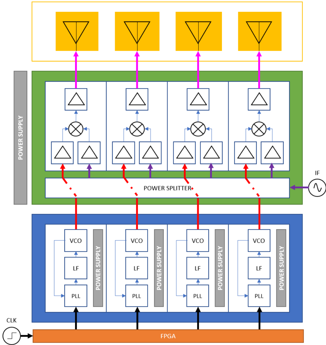
Figure 4.1 – System architecture of the proposed phased array transmitter
