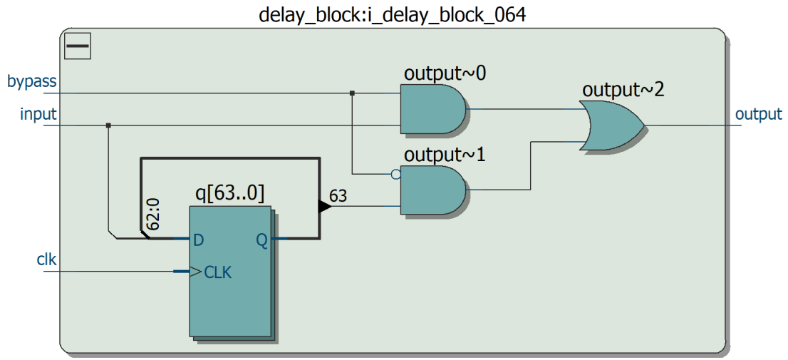
Figure 3.5 – RTL netlist view of a delay block ( k = 7 )
