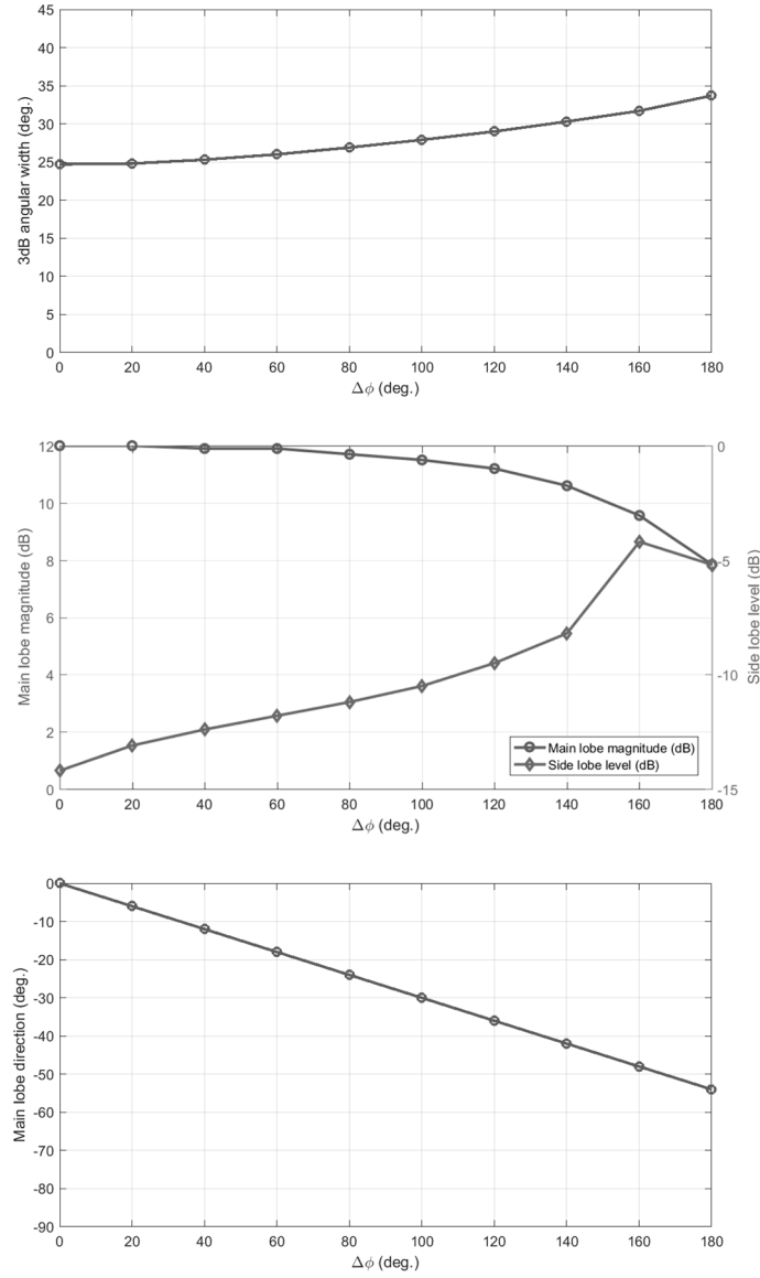
Figure 4.15 – 3-dB angular width, main lobe magnitude (compared to SLL) and main lobe direction vs. \Delta\phi
