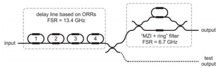
Figure 1.12 – Schematic diagram of the delay unit
