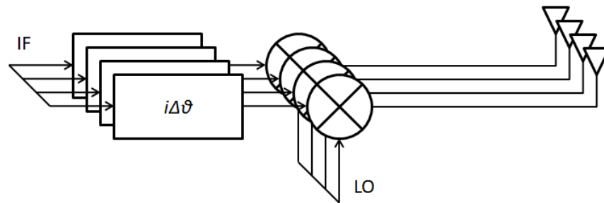
Figure 1.13 – IF phase shifting architecture block diagram
