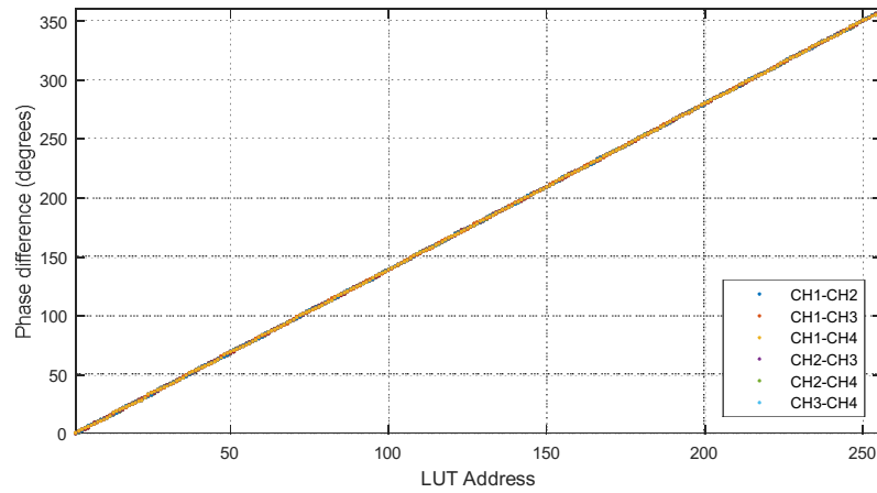
Figure 3.20 – LUT address vs. phase difference trans-characteristic (LUTa =0 to LUTa =255)
