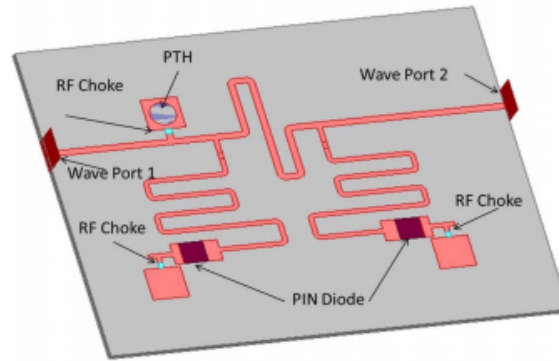
Figure 1.7 – Layout of the loaded line topology for 5.625^\circ phase bit
