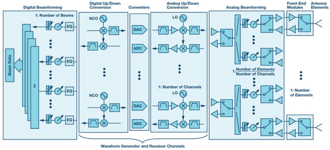
Figure 1.14 – AESA block diagram featuring analog and digital beamforming functions
