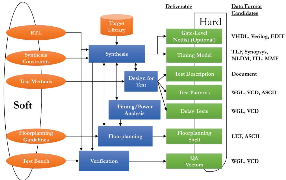
Figure A.0.4– Design flow for hard IP cores
