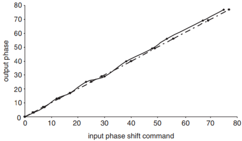
Figure 2.17 – Measured vs. ideal output phase characteristics
