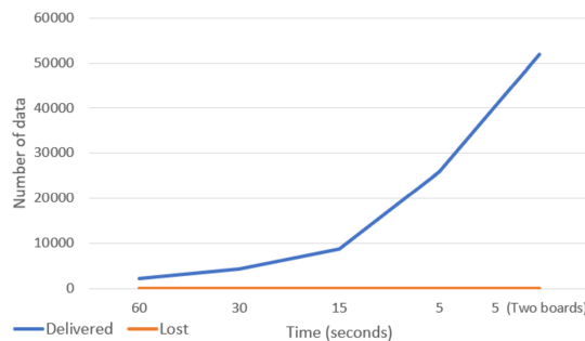
FIGURE 4.6: Results of QoS test.
