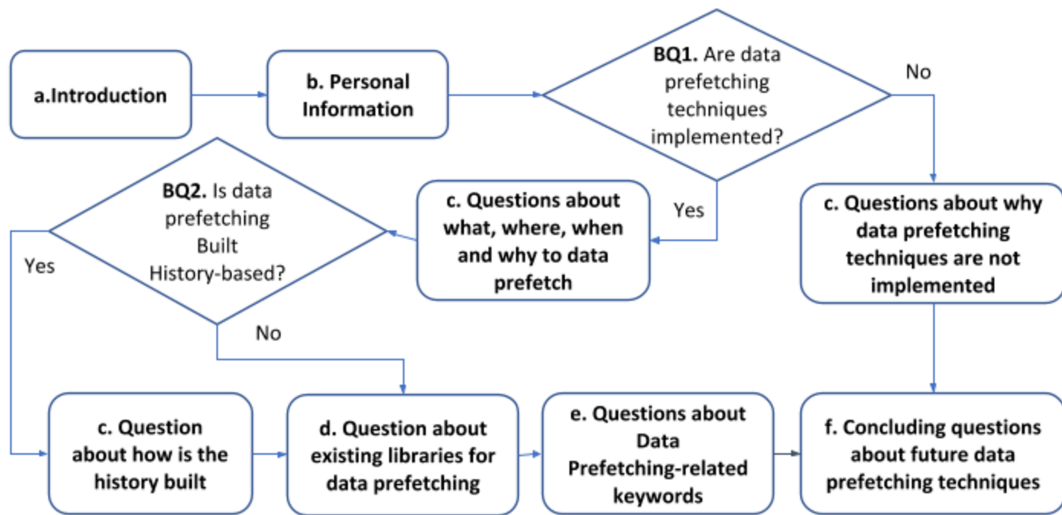
FIGURE 6.3: Questionnaire flow.
