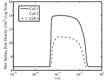
Figure 4.26: Temporal evolution of Maximum Surface Pore Density for three different cells when a time window of 1 s is considered; Rectangular unipolar pulse type, voltage amplitude 60 V, duration T = 100 \mu\text{s} , rise time t_r = 40 \mu\text{s} , fall time t_f = 40 \mu\text{s} .
