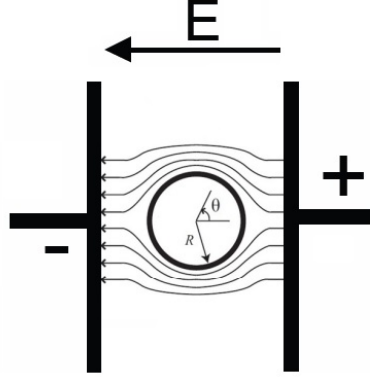
Figure 1.7: Isolated spherical cell exposed to a DC homogeneous electric field.
