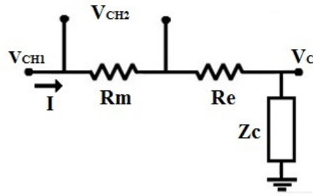
Figure 4.12: Equivalent circuit of the system used in the experiments.
