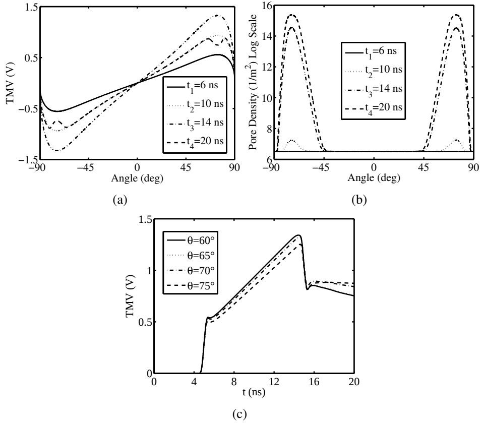
Figure 3.12: (a) TMV and (b) pore density around the cell perimeter for muscular-like cell at different time instants, (c) TMV temporal evolution at different cell membrane placement. Electric field intensity 100 kV/cm, pulse duration T = 10 ns.
