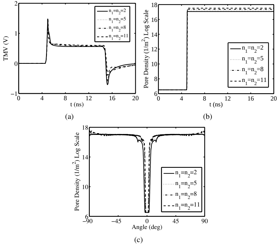
Figure 3.5: Temporal evolution of (a) TMV and (b) pore density at the top of the cell ( \theta = 90^\circ ), (c) pore density versus the polar angle at t = 20 \text{ ns} for different values of n_1 and n_2 . Pulse amplitude and duration equal to 100 \text{ kV/cm} and 10 \text{ ns} , respectively.
