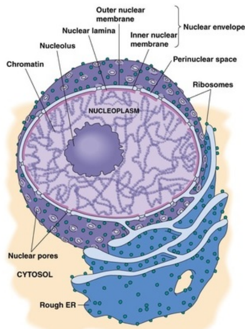
Figure 1.6: Nucleus structure.
