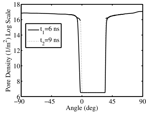
Figure 3.20: Pore density along the cell perimeter at different time, considered with respect to t_0 = 0 ns. Applied pulsed electric field having amplitude of 50 kV/cm, duration of 7 ns, rise time t_r = 2 ns and fall time t_f = 2 ns.
