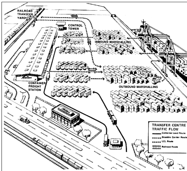
Figure 2.1 - Scheme of movements in a container terminal – Source: web
