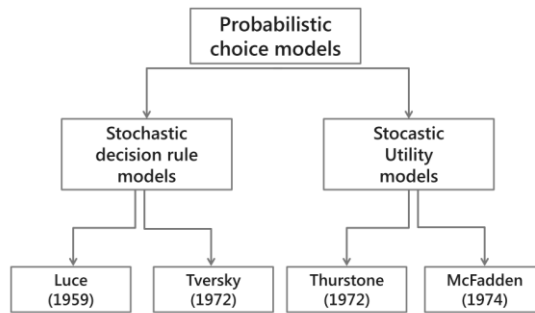
Figure 3.1 – The probabilistic choice models.
