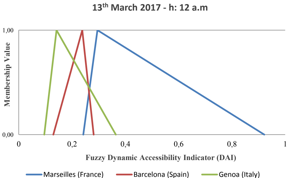
Figure 5.2- DAIs of the destination ports on 13 th March 2017 at 12 a.m.
