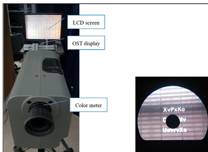
Figure 24 - Luminance contrast measurements: setup of the system (left) and the view from the color meter; the black point is the measurement area of the color meter.
