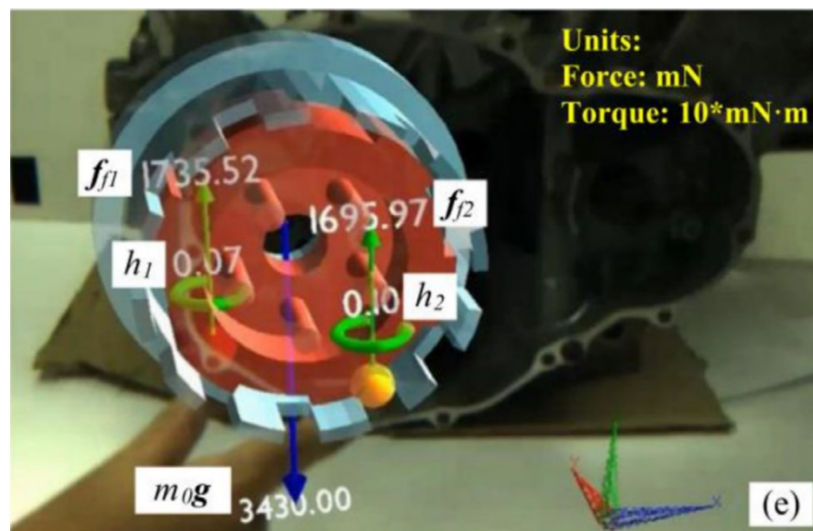
Figure 4 - Assembly planning through AR. The virtual component is overlaid on the real component. Forces are shown as arrows. Their magnitude is reported numerically. Source: (X Wang, Ong, & Nee, 2016).
