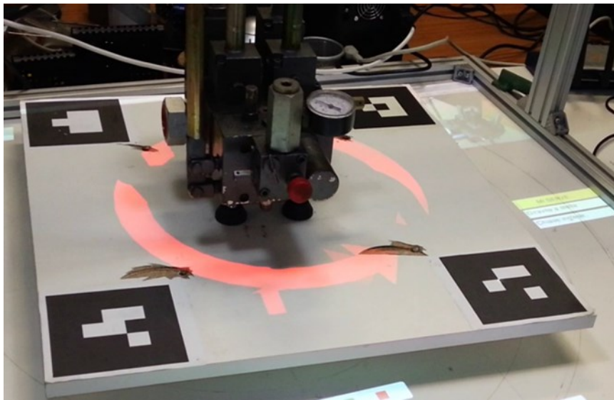
Figure 14 - The red circular arrow suggests the operator rotating counterclockwise the rotating base.
