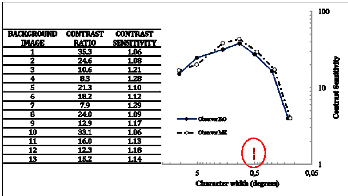
Figure 25 - Contrast measurements for the background images used in the experiment (table on the left); the plot of Contrast Sensitivity values (red points in the image on the right) reveals that with all the backgrounds, we are well below the legibility threshold in the readable zone, defined by the curves found in (Legge et al., 1987)
