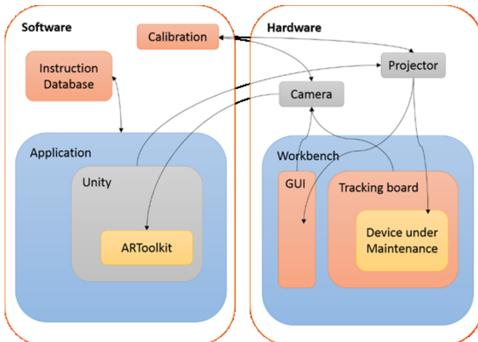
Figure 10 - The System architecture.
