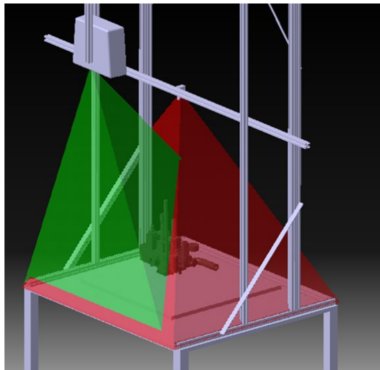
Figure 11 – The CAD design of the SAR-aided MWS prototype.
