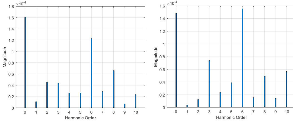
FIGURE 4.12: FFT of high frequency pressure measurements at 1080 rpm (left) and 1200 rpm (right).
