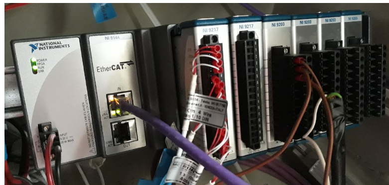
FIGURE 3.24: Second cRIO chassis with its I/O modules.
