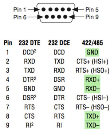
FIGURE 3.19: RS-485 Pinout.
