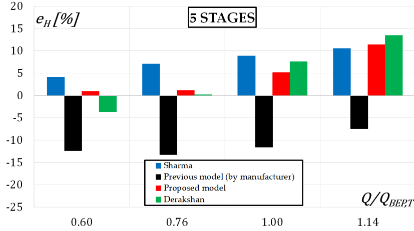
FIGURE 5.9: Comparison of models in terms of head prediction error, e_H , in the prediction of the curve in turbine mode of the 5-stages pump.
