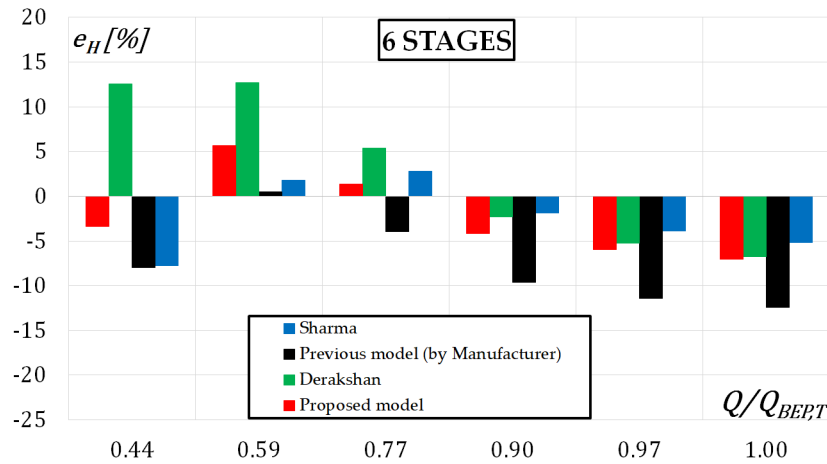
FIGURE 5.10: Comparison of models in terms of head prediction error, e_H , in the prediction of the curve in turbine mode of the 6-stages pump.
