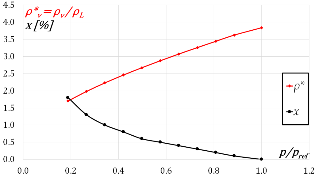
FIGURE 7.6: Values of the considered two-phase properties: mass vapor fraction, x , and non-dimensional vapor density, \rho_v^* , vs. pressure.
