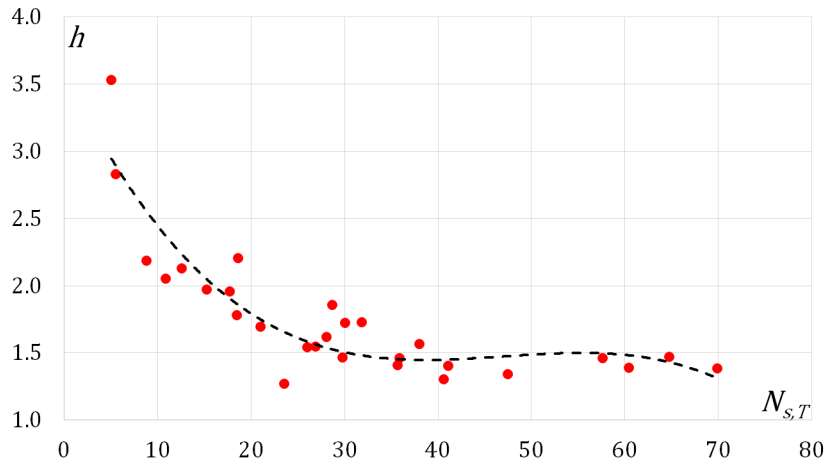
FIGURE 5.2: Head prediction factor, h , vs. specific speed number in turbine mode, N_{s,T} .
