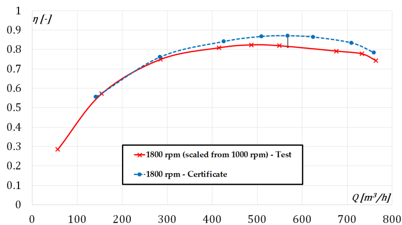
FIGURE 4.11: Experimental and certificate efficiency, \eta , vs. discharge, Q , under pump operation mode 1000 rpm .
