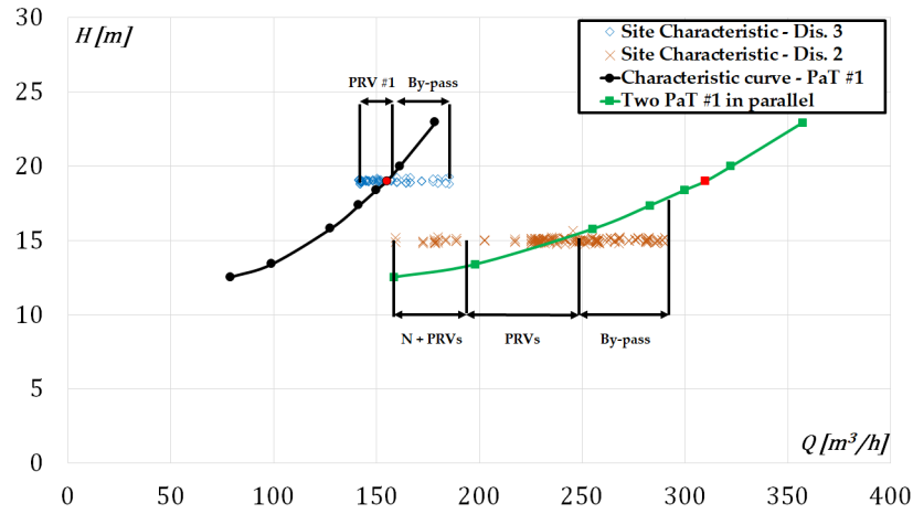
FIGURE 6.12: Characteristic curve of PaT # 1 during the night (in black) and characteristic curve of two PaT # 1 in parallel during the day (in green) with their regulation methods.
