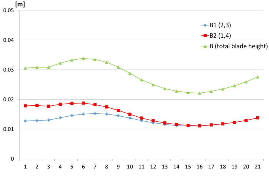
Figure 4.14: Blade height, resulting from the imposed functions and calculation.
