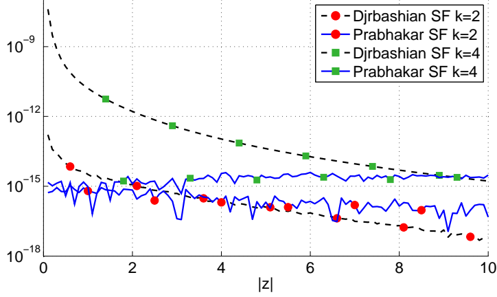
Figure 1: Comparison of errors provided by Djobashian and Prabhakar SFs for \alpha = 0.6 , \beta = 1.0 and \arg(z) = \pi .
