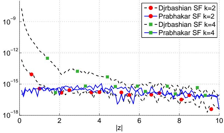
Figure 2: Comparison of errors provided by Djobashian and Prabhakar SFs for \alpha = 0.8 , \beta = 1.2 and \arg(z) = \pi/2 .
