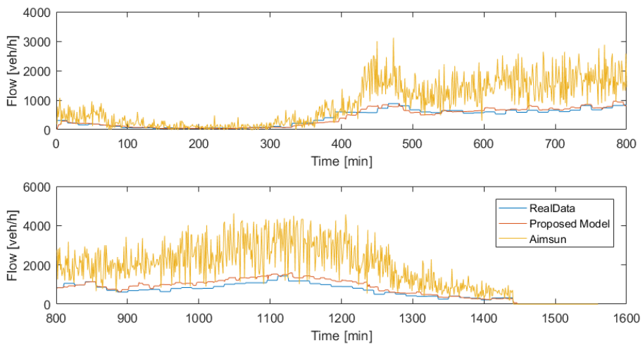
Fig. 21 - Flow estimations of the proposed model for passenger car class compared to Aimsun results and real observations for link 4 (Greenshields model)
