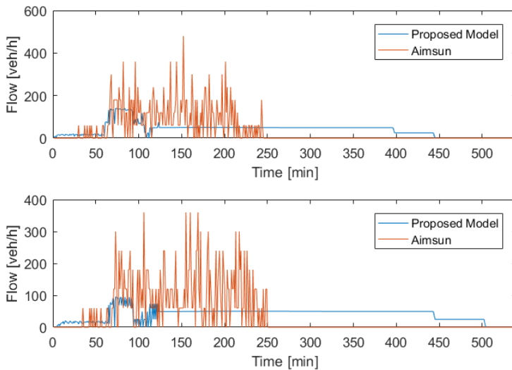
Fig. 38 - Estimated flow obtained by Aimsun and the proposed model for Bus class for link 1-2 (Greenshields relation)
