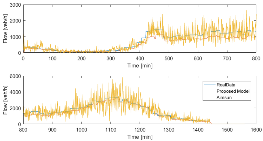
Fig. 15 - Flow estimations of the proposed model passenger car class compared to Aimsun results and real observations for link 2 (Greenshields model)
