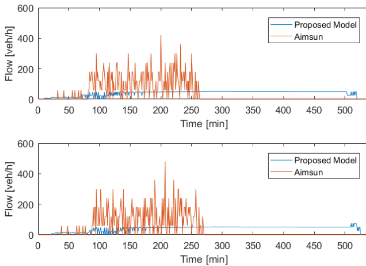
Fig. 42 - Estimated flow obtained by Aimsun and the proposed model for HGV class for link 3-4 (Greenshields relation)
