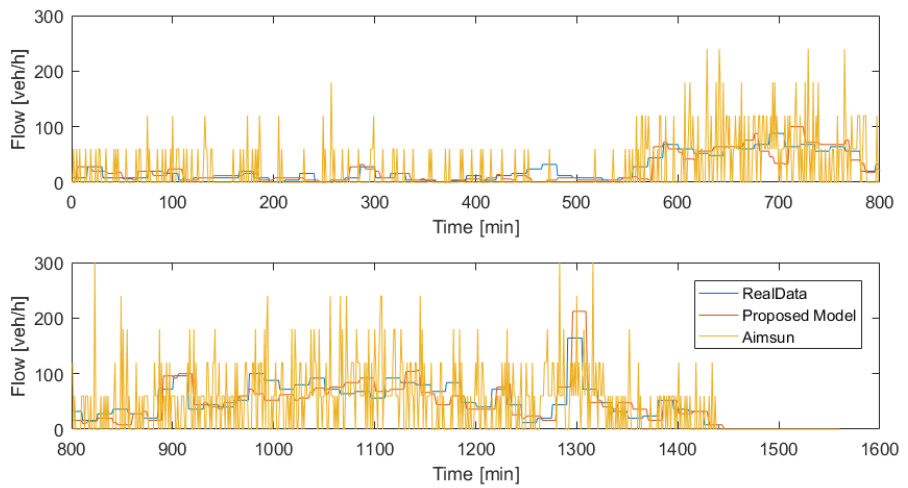
Fig. 17 - Flow estimations of the proposed model for HGV class compared to Aimsun results and real observations for link 2 (Greenshields model)
