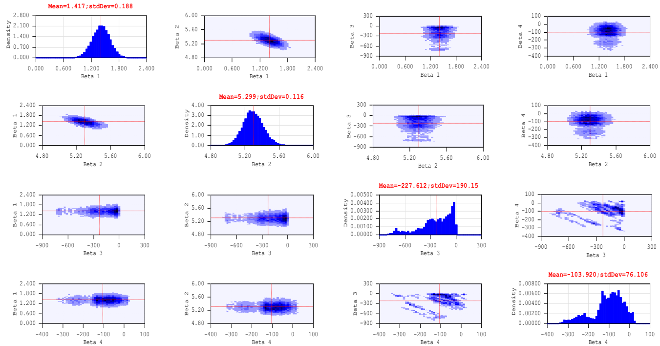
figure 6.39– TCEV posterior plot for Finniss River - Gitchams Xng
