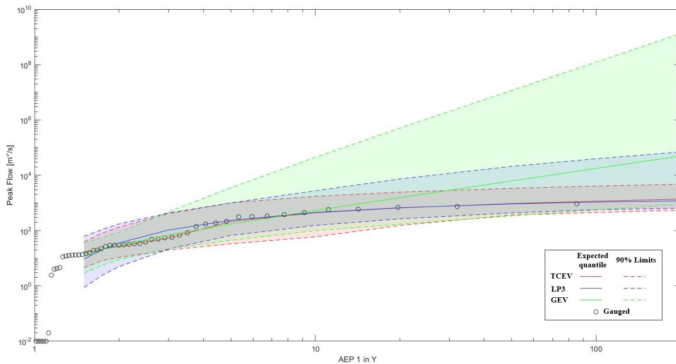
figure 6.26 – TCEV, LP3 and GEV probability plots for Bell Creek at Craiglands
