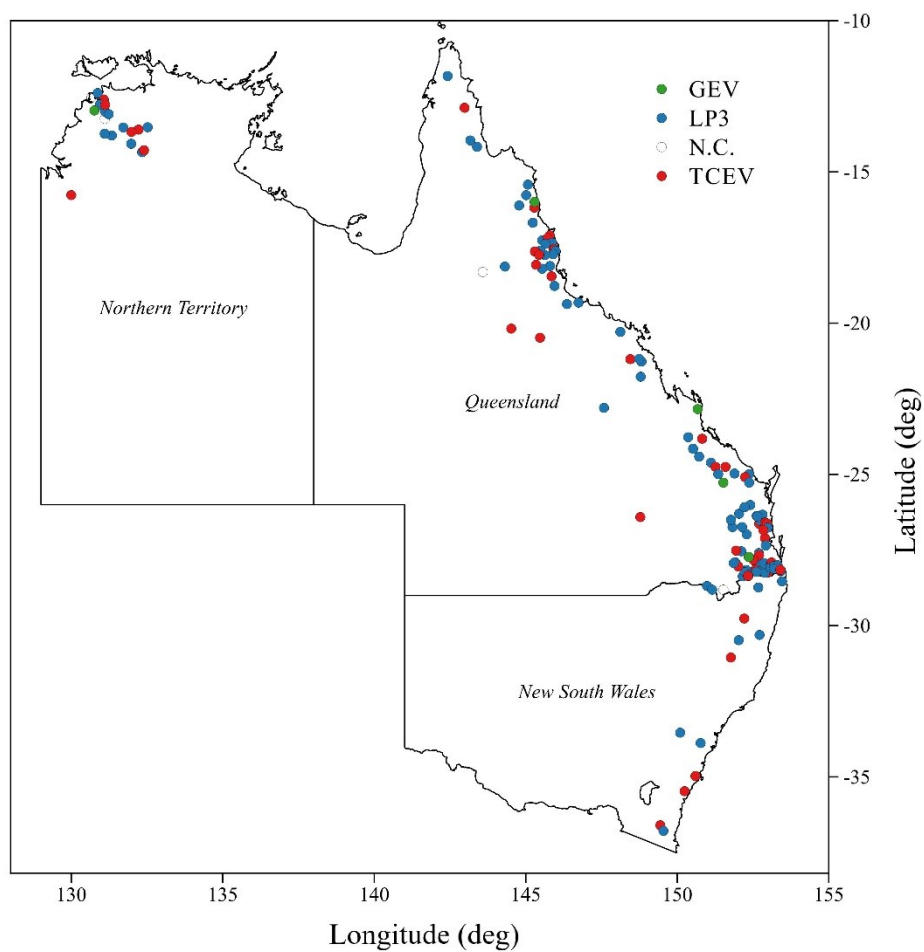
fig. 6.41 – Corrected version of Akaike Information Criterion results (N.C. stands for Not Computable)
