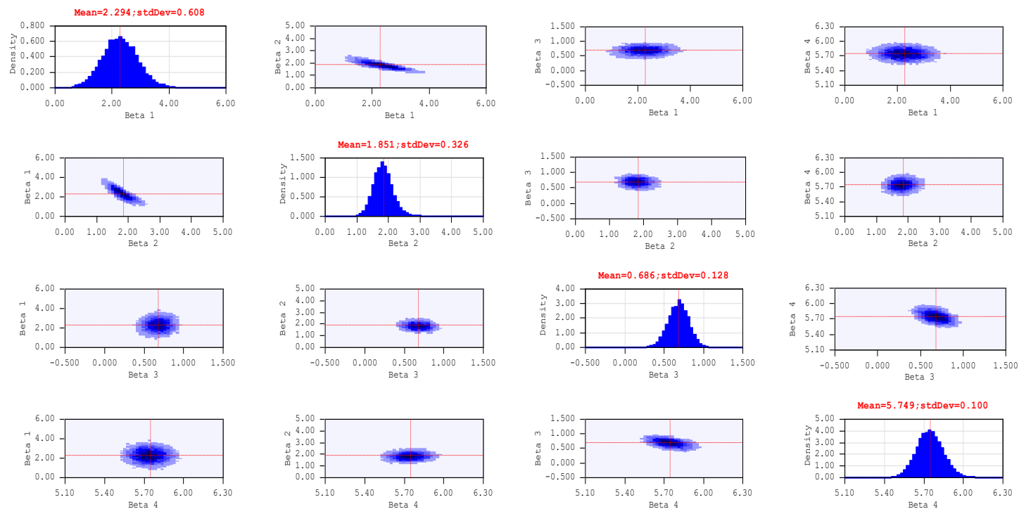
figure 6.30 – TCEV posterior parameters plots for Albert River at Bromfleet
