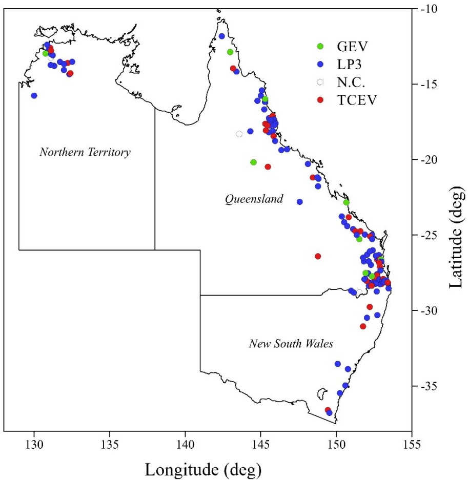
fig. 6.42 – Bayesian Information Criterion results (N.C. stands for Not Computable)
