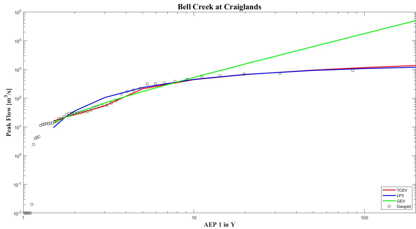
figure 6.25– TCEV, LP3 and GEV expected quantiles probability plots for Bell Creek at Craiglands
