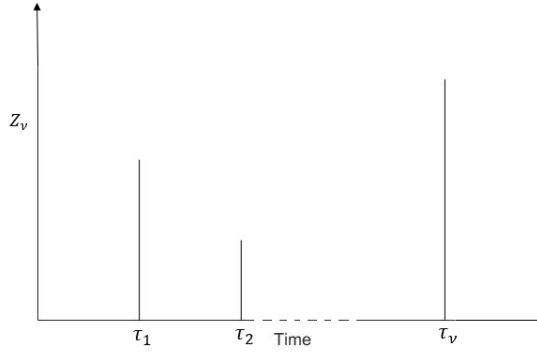
Figure 2.2 – A realization of the stochastic process of flood peak exceedances
