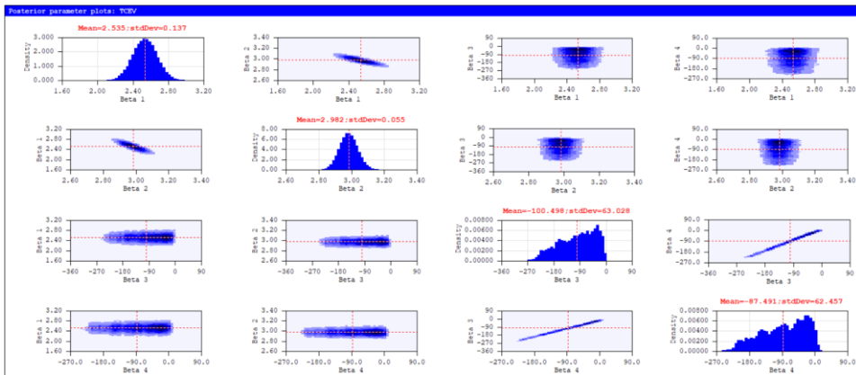
fig. 5.1 – Posterior parameters plot of TCEV (from a Gumbel distributed sample)
