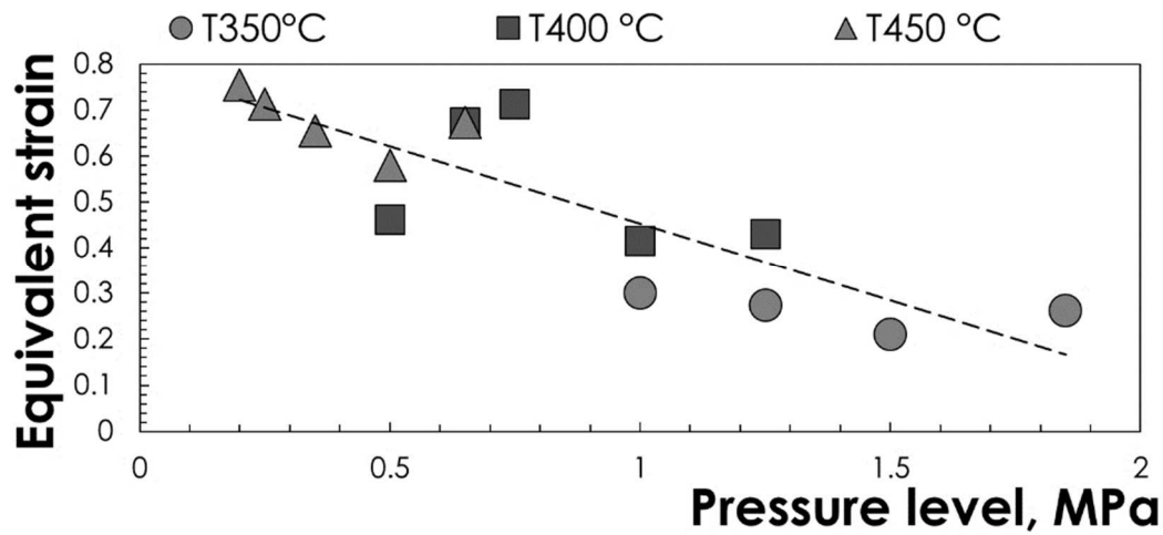
Figure 75 Equivalent strain at the dome apex according to temperature and pressure for CP method.
