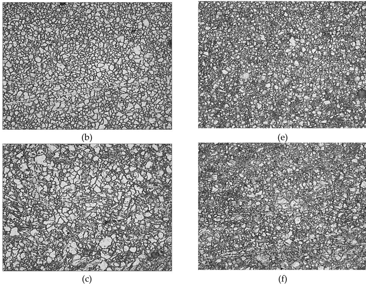
Figure 129: Microstructure of tested samples after SPF according to: (i) feed rate, 200 (a), 400 (b) and 600mm·min -1 , at a fixed step down of 0.1mm; (ii) step down, 0.1 (d), 0.2 (e) and 0.3mm, at a fixed feed rate of 200 mm·min -1 .
