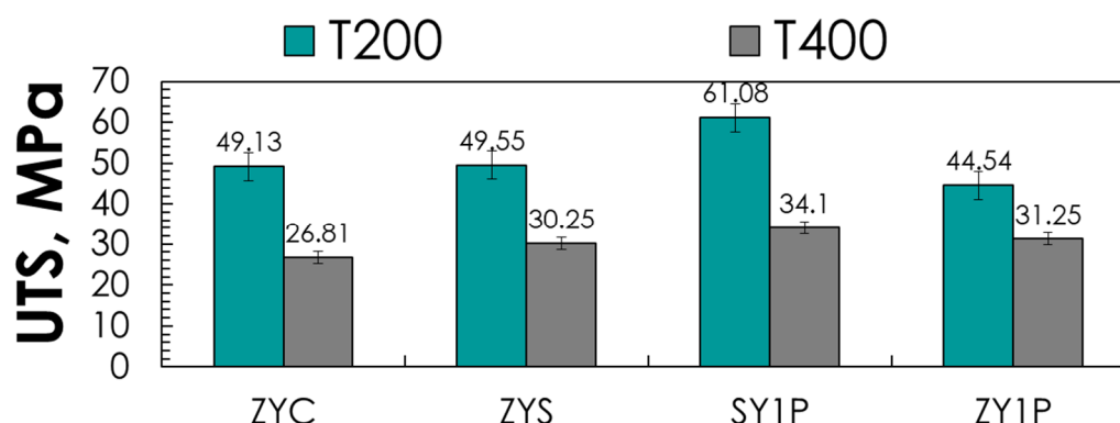
Figure 53 UTS according to temperature for Mg-based alloy with three alloying elements.
