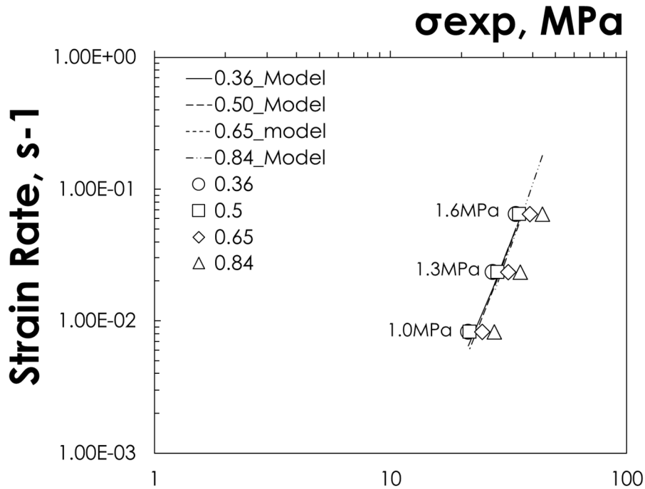
Figure 103 Comparison between analytical and experimental results in terms of the strain rate according to the stress for the highest values of pressure (1.0, 1.3 and 1.6MPa) investigated.
