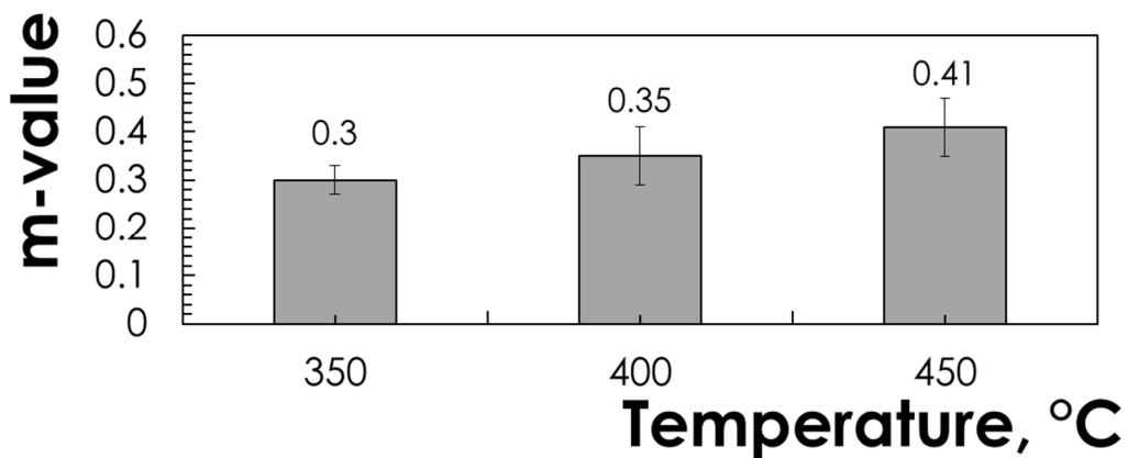
Figure 68 m-value obtained from CP-tests.
