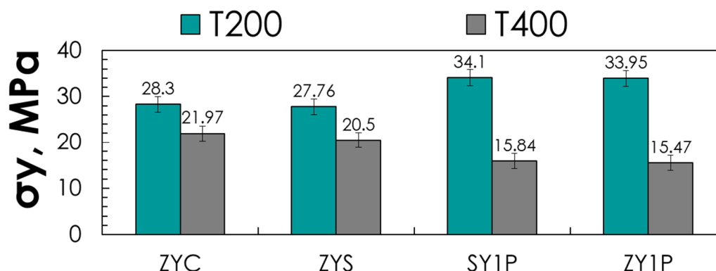
Figure 52 \sigma_y according to temperature for Mg-based alloy with three alloying elements.
