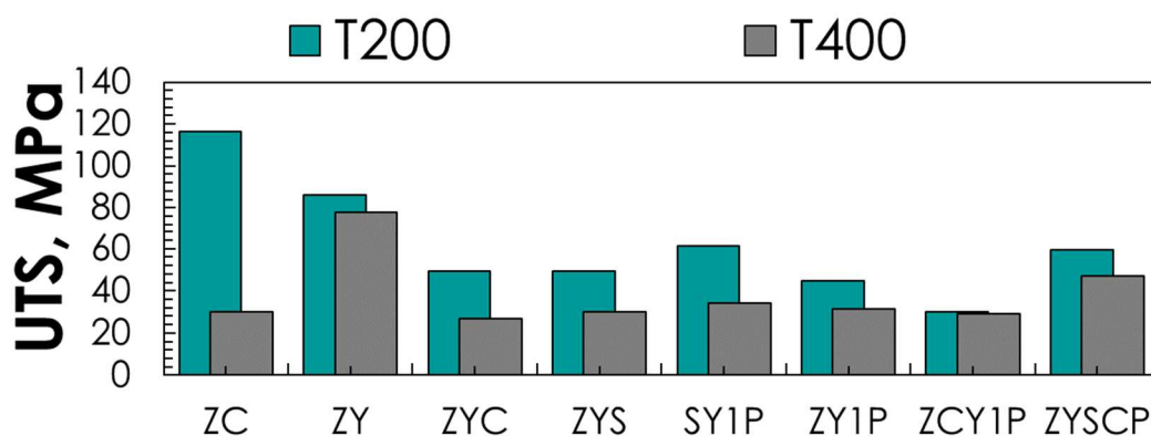
Figure 59 UTS change with temperature for all Mg-based alloys investigated.
