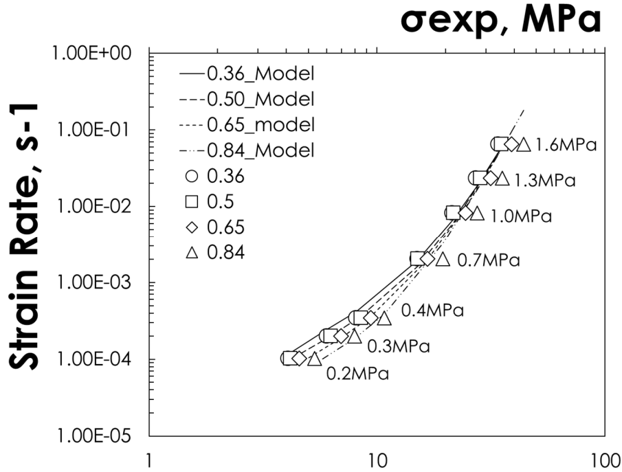
Figure 104 Analytical/experimental results comparison in terms of strain rate according to stress.
