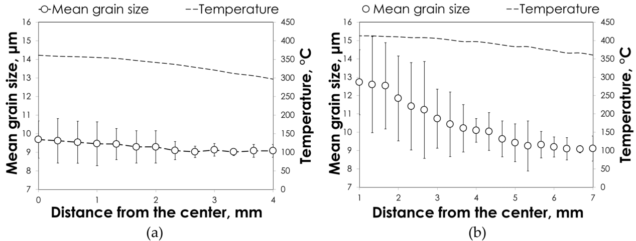
Figure 140: Experimental results: temperature and microstructure for 200 (a) and 250W (b).
