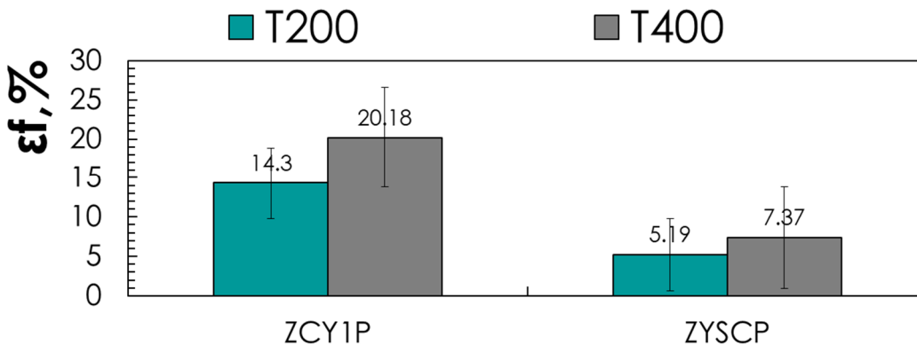
Figure 57 \epsilon_f change with temperature for Mg-based alloy with three alloying elements.
