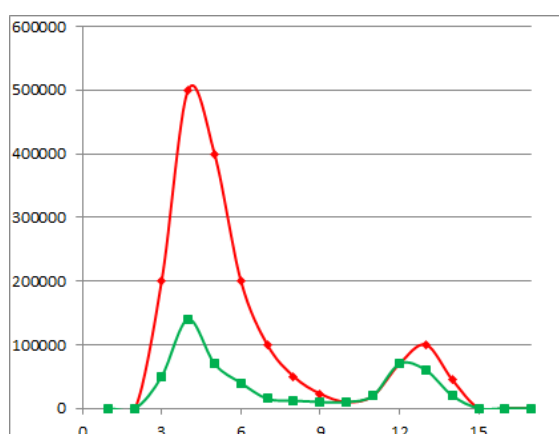
Figure 1.3.21. Distribution of the medium diameter (µm) for U937 live (green) and death (red) cells sonicated at 1 MHz.
