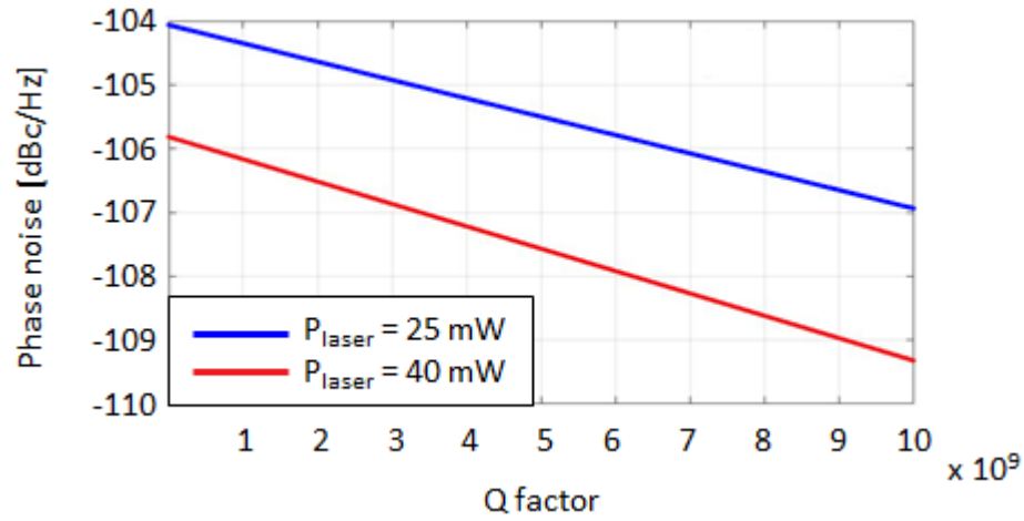
Fig.4.16. Phase noise trend of LCMW (output power \approx 10 dBm) vs ring resonator Q-factor, for P_{laser} equal to 25 mW(blue) and 40 mW(red).
