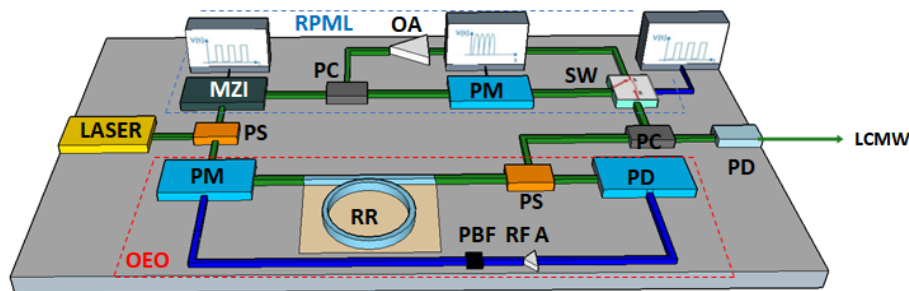
Fig.4.14. Design scheme of linearly chirped microwave waveform ( LCMW ) generator, ( PS : power splitter, MZI : Mach-Zehnder modulator, PC : power combiner, OA : optical amplifier, PM : phase modulator, SW : switch, PD : photodiode, RR : ring resonator, RF A : electric amplifier, RPML : recirculating phase modulation loop, OEO : optoelectronic oscillator, PBF : pass-band filter). Optical connections are in green, electrical ones are in blue.
