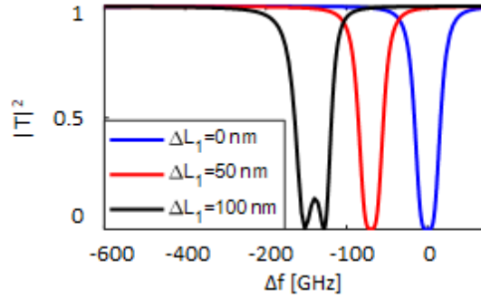
Fig. 3.15. PhCRR transmission as function of \Delta f at three different values of \Delta L_1 [101] © 2019 IEEE.
