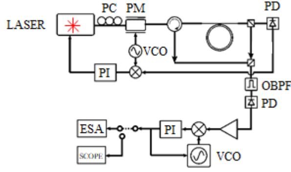
Fig. 2.8. Brillouin-based gyroscope architecture [67], ( PC : polarization controller, PM : phase-modulator, PI : proportional integral servo, OBPF : optical band-pass filter, ESA : electrical spectrum analyzer, VCO : voltage-controlled oscillator, PD : photodiode).
