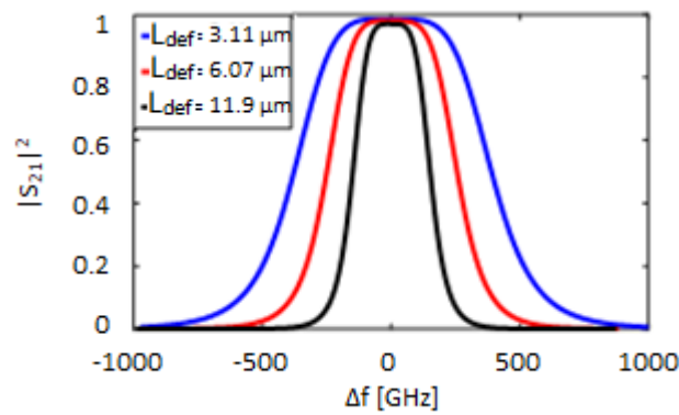
Fig. 3.18. Transmission spectra S_{21} of sidewall grating with N_t = 128 and N_d = 6 for several values of the L_{def} compliant to Eq. (3.3) [101] © 2019 IEEE.
