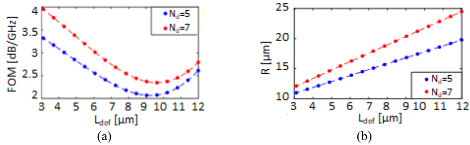
Fig. 3.19. (a) Figure-of-merit FOM (ER/BW) ; (b) PhCRR radius R as a function of L_{def} , for PhCRRs with N_t = 256 and N_d = 5 (blue curve), and N_d = 7 (red curve). The dotted points refer to defects lengths L_{def} that are compliant to Eq. (3.3) [101] © 2019 IEEE.
