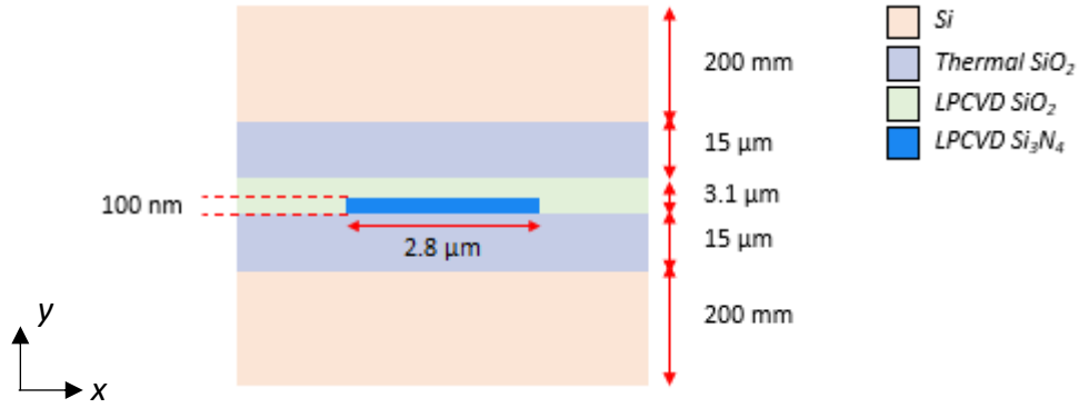
Fig. 2.31. Si 3 N 4 – based waveguide 100 nm thick and 2.8 μm wide ( LPCVD : Low Pressure Chemical Vapour Deposition).
