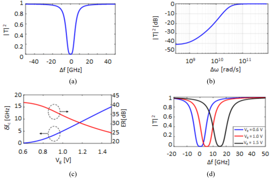
Fig. 3.22. (a) Transmission spectrum of the PhCRR with N_t = 256 , N_d = 7 , L_{def} = 3.11 \mu\text{m} ( k^2 = 20\% ) and Bode plot (b) of the 1 st order Butterworth low pass filter ( \omega is the angular frequency [rad/s] and \Delta\omega is the angular frequency shift from the operating angular frequency). (c) Shifting of the central frequency and ER trends as a function of the applied voltage V_g , with some examples of the transmission spectra after voltage tuning (d) ( f_0 \approx 193.2877 THz) [101] © 2019 IEEE.
