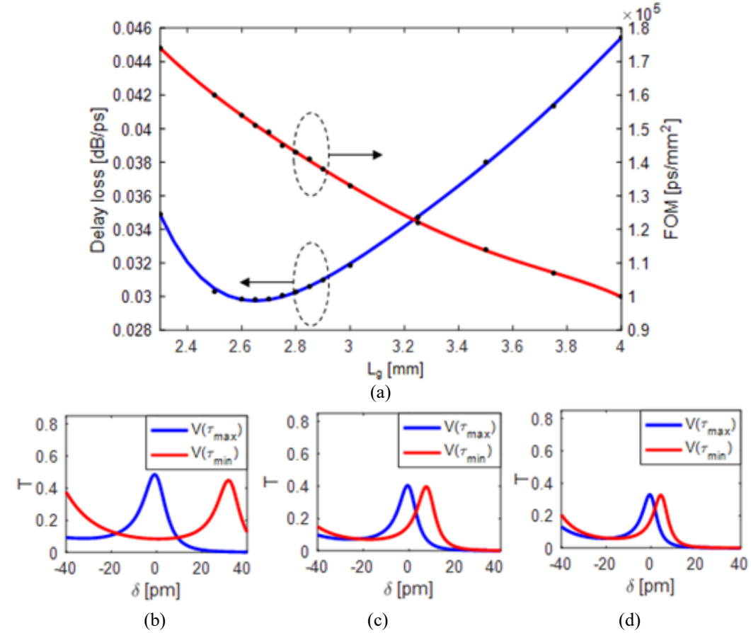
Fig. 4.11. (a) Delay loss (blue line) and FOM (red line) as a function of L_g . Transmission spectra at the band edge of the Bragg grating with (b) L_g = 2.3 mm ( \lambda_0 = \lambda(\tau_{max}) = 1547.67 nm), (c) L_g = 2.6 mm ( \lambda_0 = \lambda(\tau_{max}) = 1547.65 nm), and (d) L_g = 2.9 mm ( \lambda_0 = \lambda(\tau_{max}) = 1547.63 nm), when V(\tau_{max}) and V(\tau_{min}) are applied to the graphene electrodes. Reprinted with permission from [65] © The Optical Society.
