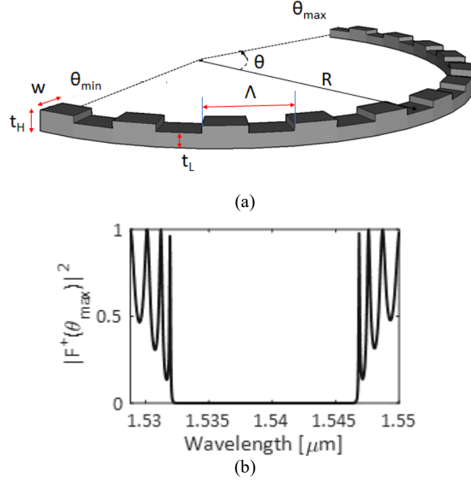
Fig. 2.26. Schematic of a bent \text{Si}_3\text{N}_4 top grating (a) and its transmission power ( |F_g^+(\theta_{\max})|^2 ) spectrum.
