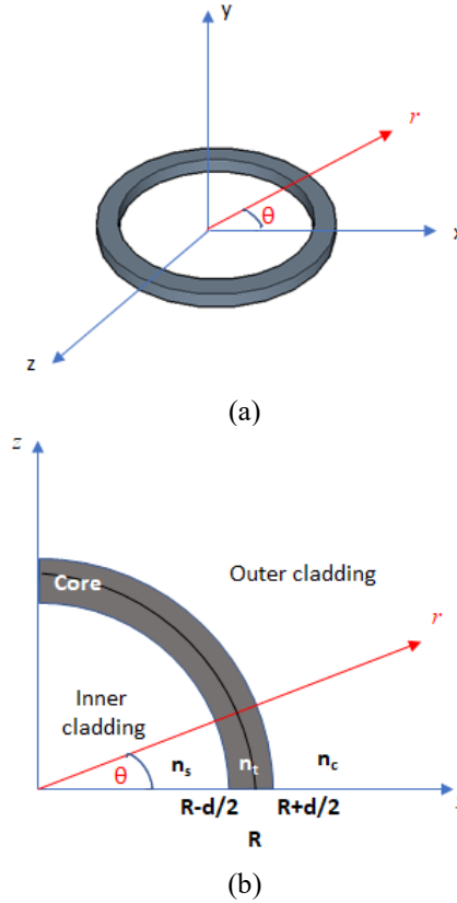
Fig. 2.23. (a) 3D waveguiding ring in Cartesian (blue lines) and Cylindrical (red lines) coordinates. (b) 2D focus on a ring resonator section, ( n_s = refractive index of inner cladding, n_t = refractive index of core, n_c = refractive index of outer cladding, R = radius of curvature, d = waveguide width).
