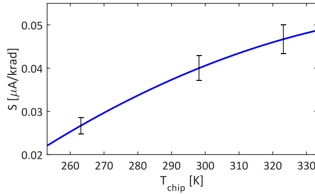
Fig. 2.12. S [ \mu\text{A}/\text{krad} ] vs T_{\text{chip}} [K]. Reprinted with permission from [95] © The Optical Society.
