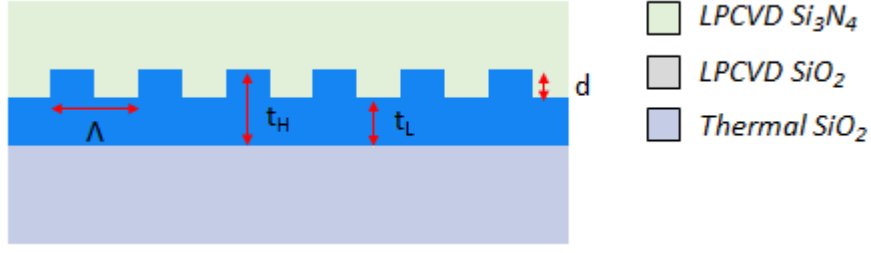
Fig.2.33. Si 3 N 4 -based top grating, ( \Lambda : period; t_H : maximum thickness; t_L : minimum thickness; d : modulation depth).
