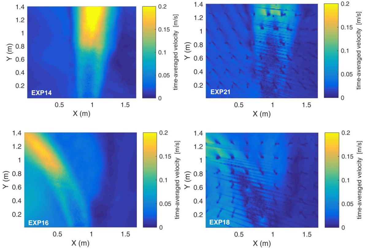
Figure 5. Time-averaged velocities in the horizontal layer at z=0 : top line no rotation; left column no obstructions
