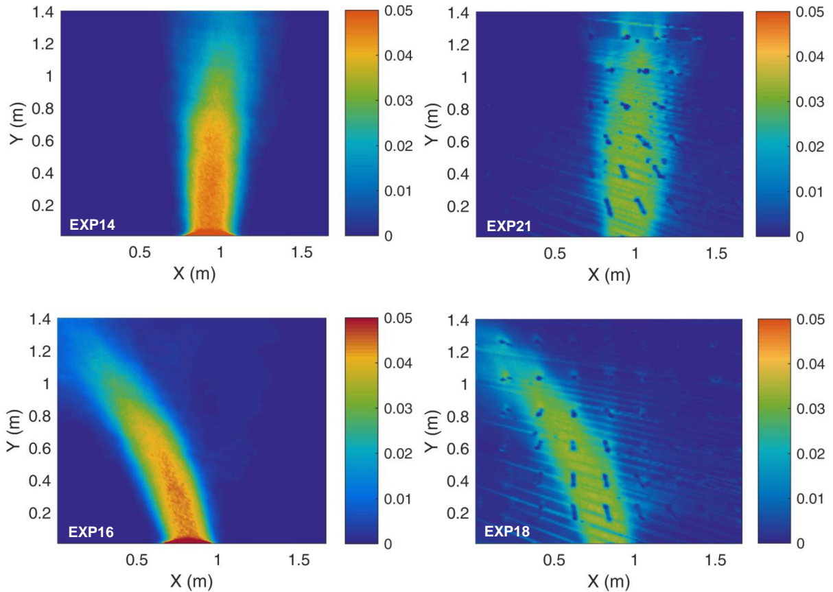
Figure 7. Time-averaged turbulent Reynolds stresses \overline{u'v'} [ \text{m}^2/\text{s}^2 ] in the horizontal layer at z=0 : top line no rotation; left column no obstructions
