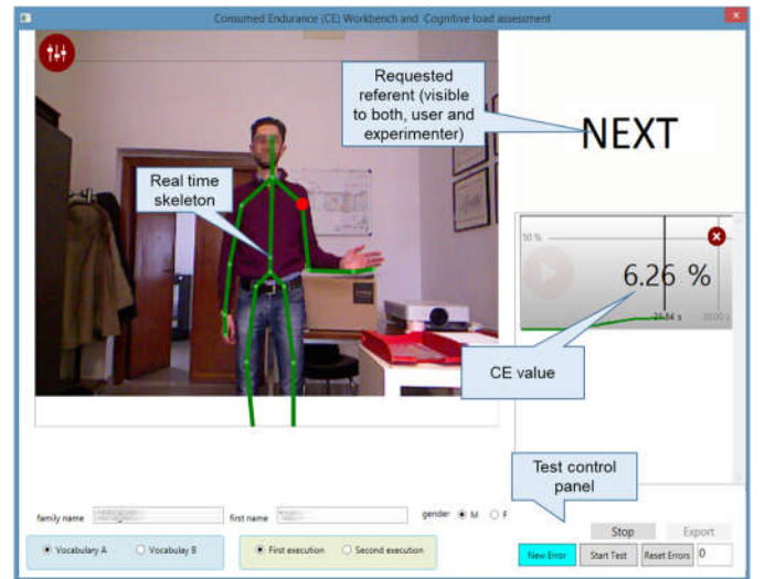
Fig. 3. Experimenter view of VocVal. Participants can see only the required command.
