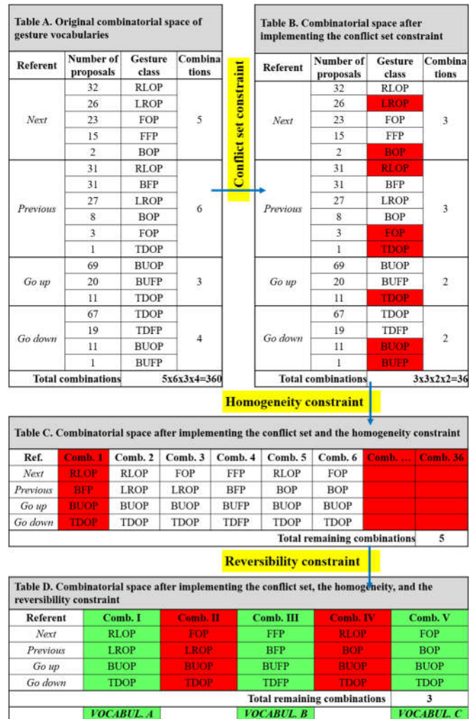
Fig. 5. Filtering process for the identification of the optimal gesture vocabulary. After implementing conflict set, homogeneity and reversibility constraints, the original combinatorial space of vocabularies decreases from 360 (Table A) to 3 (Table D) possible vocabularies. The acronyms utilized in the figure are described in Fig. 4.
