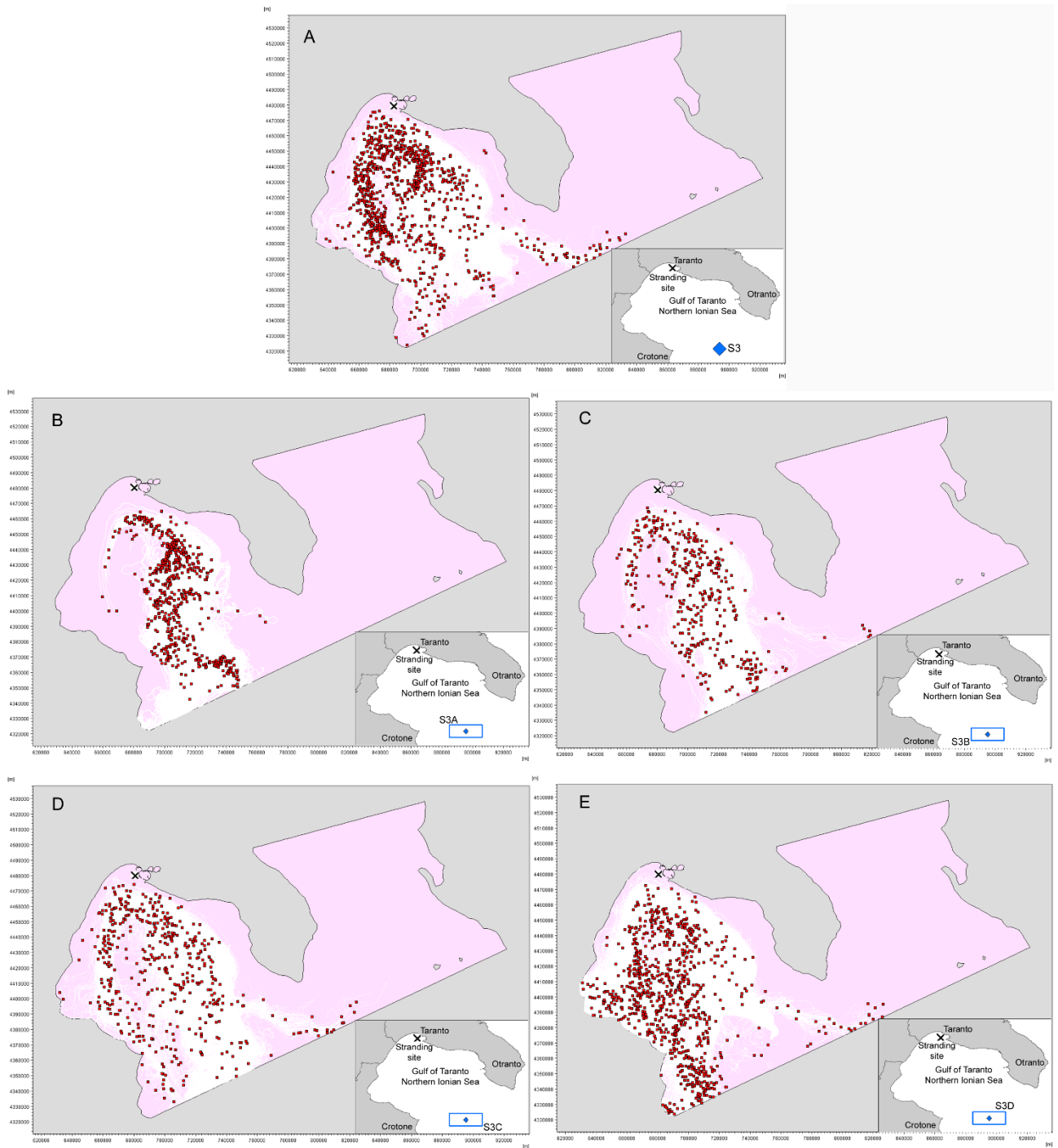
Fig. B4. The cloud of virtual particles (1000 in number) released 30 days prior to the finding date, starting from: a) S3; b) S3A; c) S3B; d) S3C; e) S3D.
