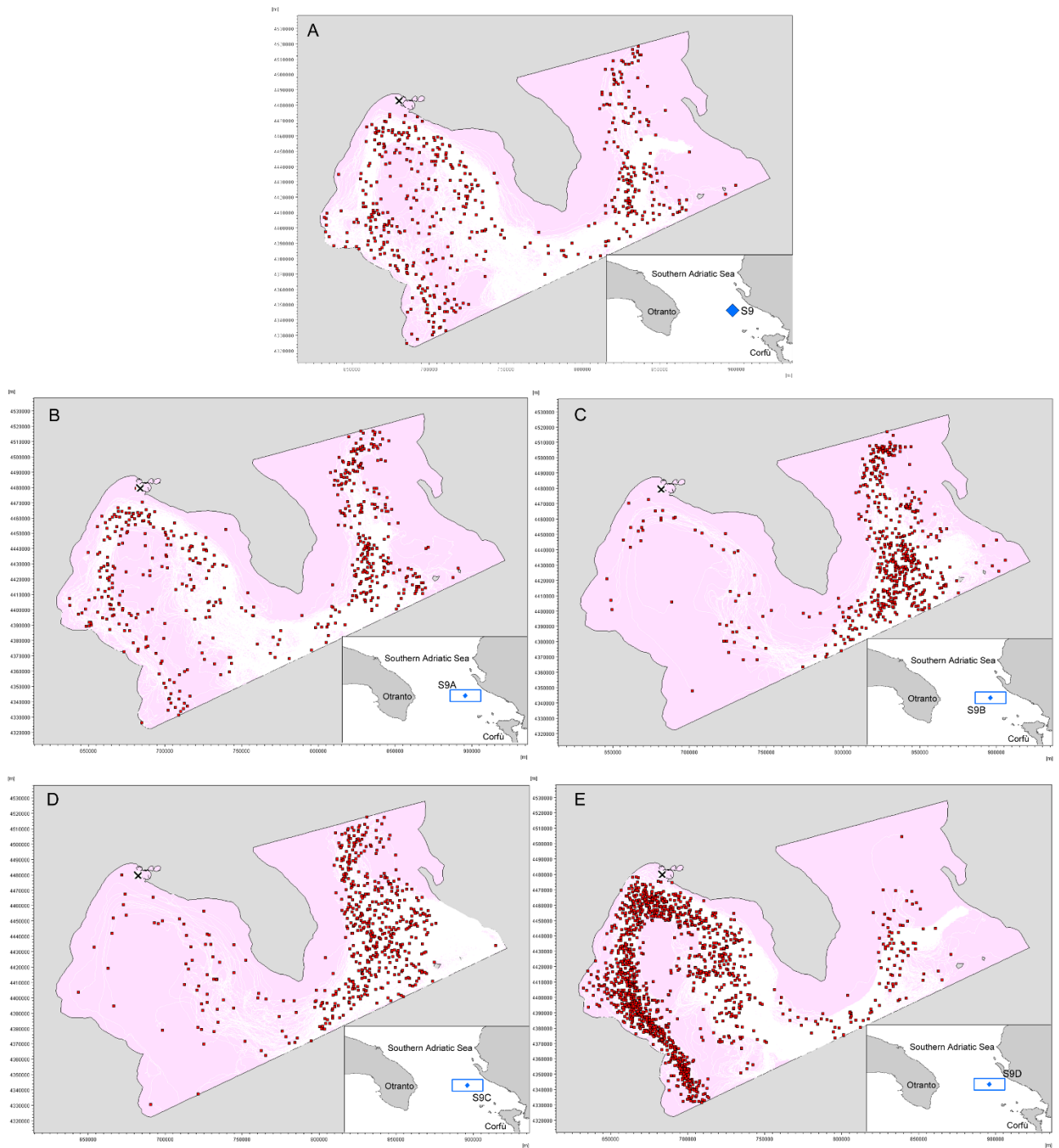
Fig. B3. The cloud of virtual particles (1000 in number) released 20 days prior to the finding date, starting from: a) S9; b) S9A; c) S9B; d) S9C; e) S9D.
