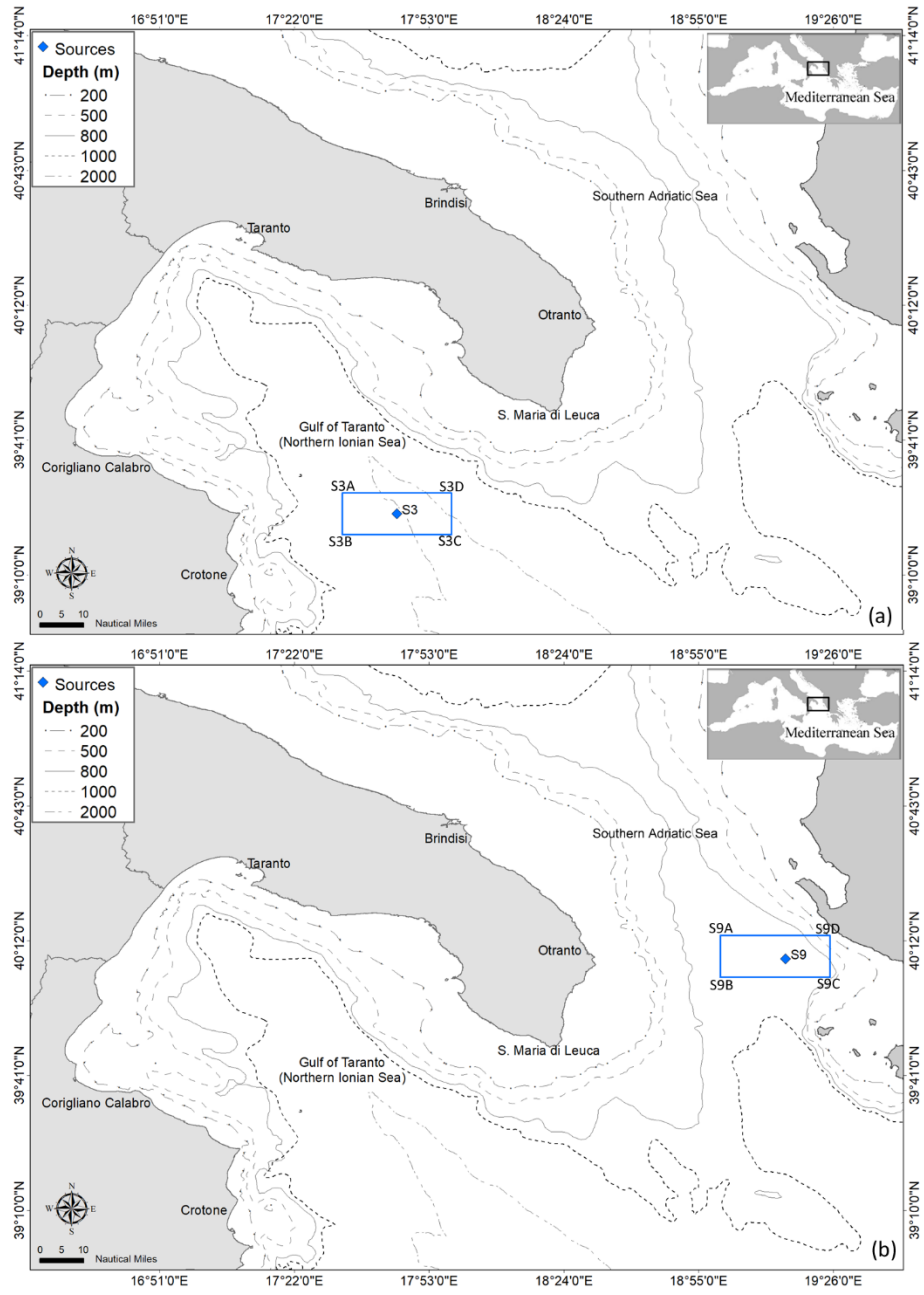
Fig. B1. Map of the 37x20 km 2 areas identified around sources S3 and S9 with indication of respective vertices.
