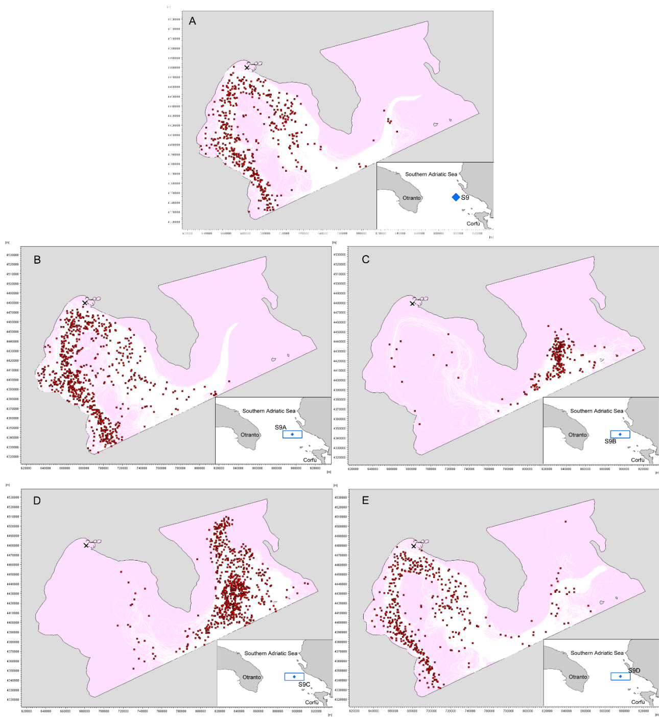
Fig. B5. The cloud of virtual particles (1000 in number) released 30 days prior to the finding date, starting from: a) S9; b) S9A; c) S9B; d) S9C; e) S9D.
