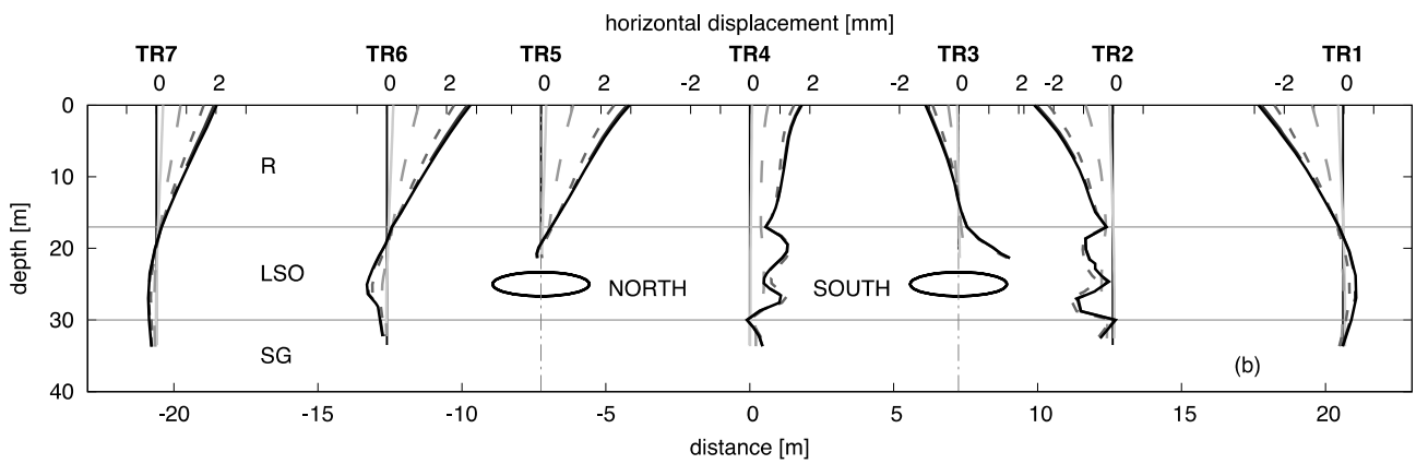
tunnel face distance from monitoring section [m] -19.6 ——— 0.0 - - - 19.6 - - - - 39.2 - - - - 58.8 ——— Fig. 17 - Class A predictions: profiles of incremental horizontal displacements for Trivecs: (a) North Tunnel, (b) South Tunnel
