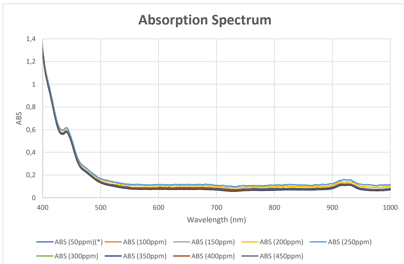
Figure 4.15. Absorption Spectrum of the Diesel-Water at 400-1000 nm.
