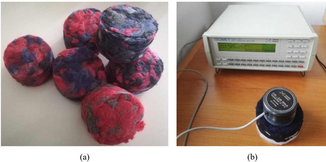
Figure 3.1. Samples (a) and apparatus for testing thermal properties (b).
