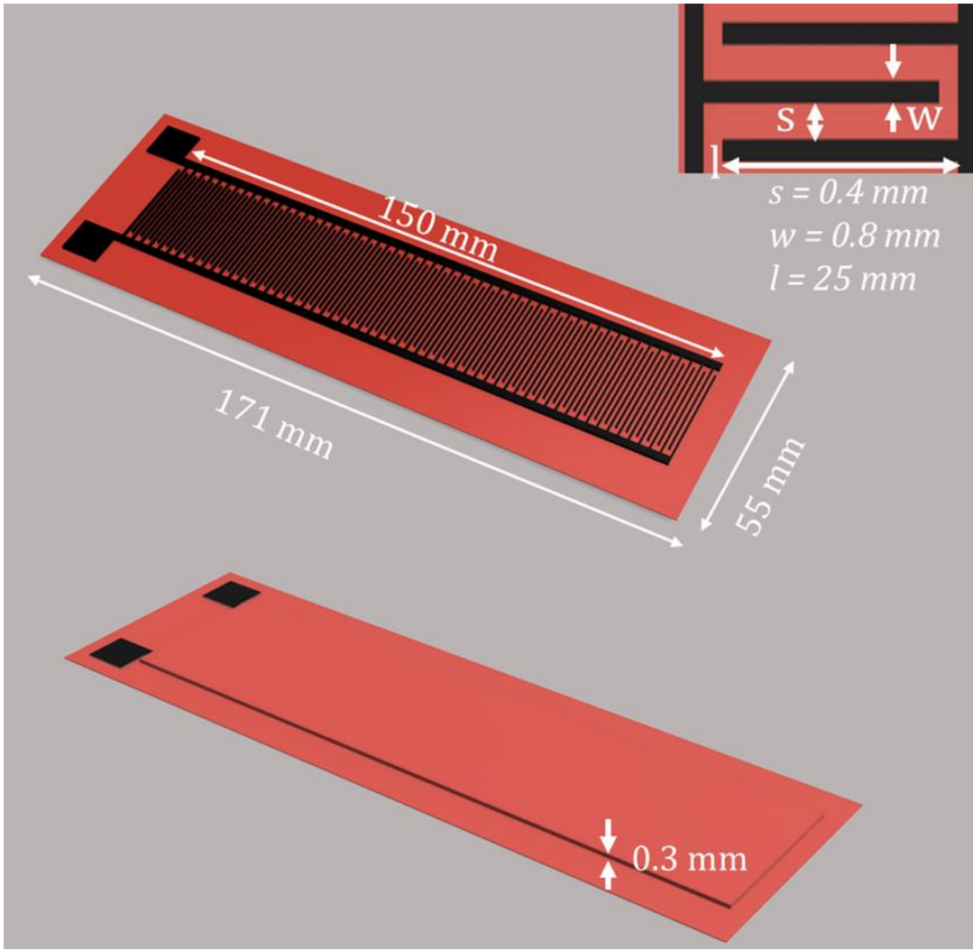
Fig. 2-19- CAD design of the proposed capacitive liquid level sensor.
