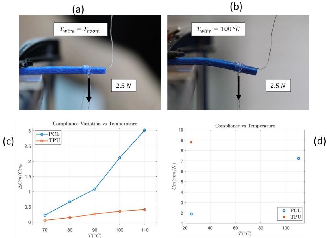
Fig. 4-2- a) Tested sample when T_{wire} = T_{room} , and b) T_{wire} = 100\text{ °C} . c) \Delta Cm / Cm_0 vs T for PCL and TPU, d) absolute compliance vs T for PCL and TPU.
