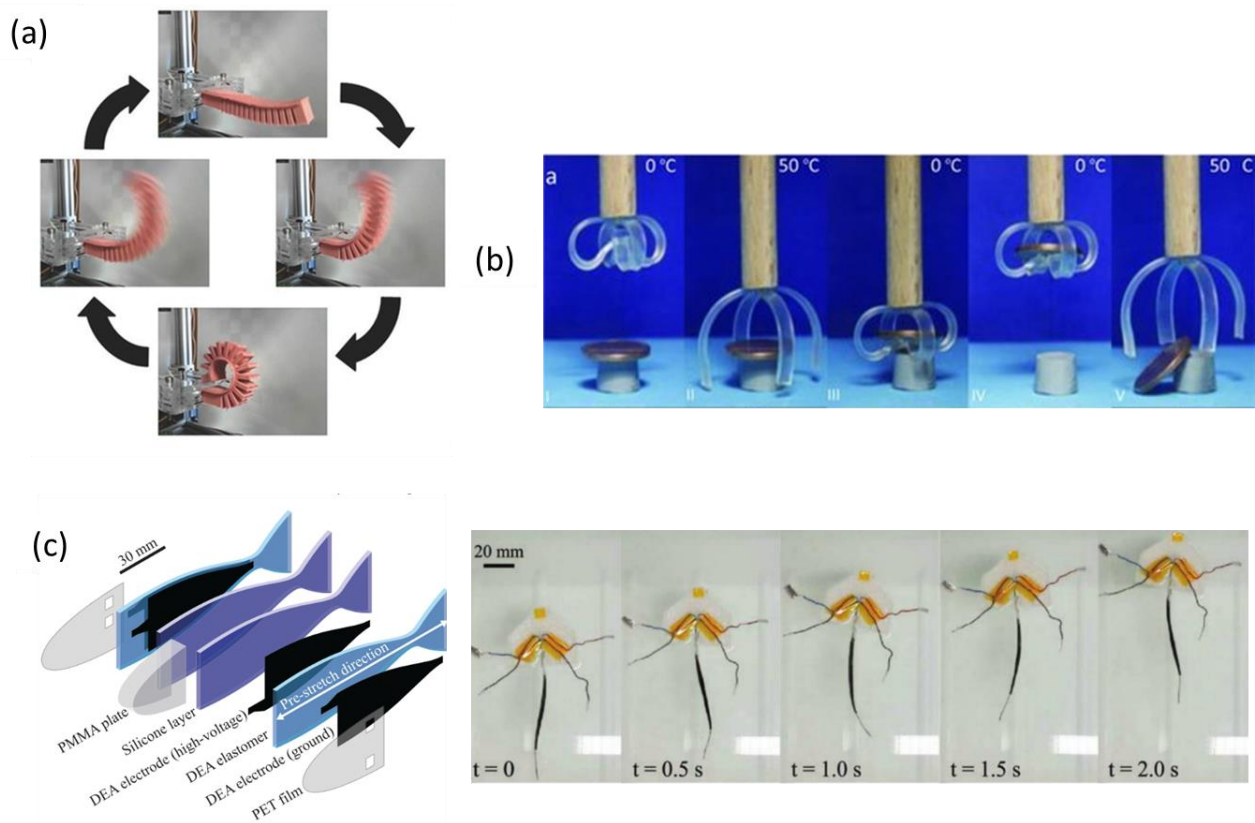
Fig. 3-2 Examples of actuation systems in soft robot: a) FFA gas-driven actuation system. Reprinted with permission from [116]. b) micro gripper based on SMP actuation system. Reprinted with permission from [117]. c) fish-inspired soft robot based on DEA actuation system, able to swim in water. Reprinted with permission from [77]
