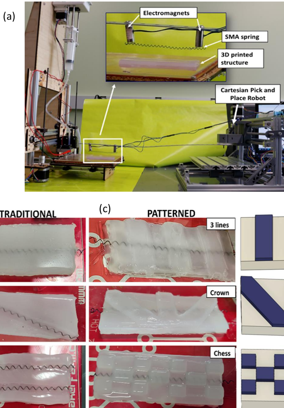
Fig. 3-15- a) CPPR used to automatically embed SMA into silicone skins, b) Traditional silicone skins, and c) Patterned silicone skins.
