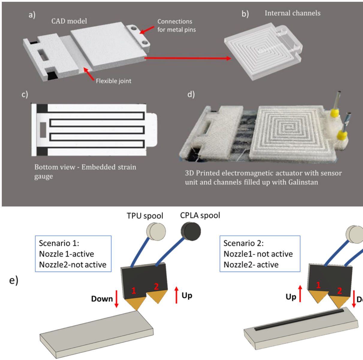
Fig. 3-24 Soft EM actuator: a) Computer Aided Design (CAD) model; b) internal channels; c) Bottom view: embedded strain gauge sensor (white = TPU, black = CPLA); d) 3D Printed EM soft actuator with embedded sensor and channels filled up with Galinstan; and e) Schematic diagram depicting the basic multi-material-extrusion working mechanism of Ultimaker 3.
