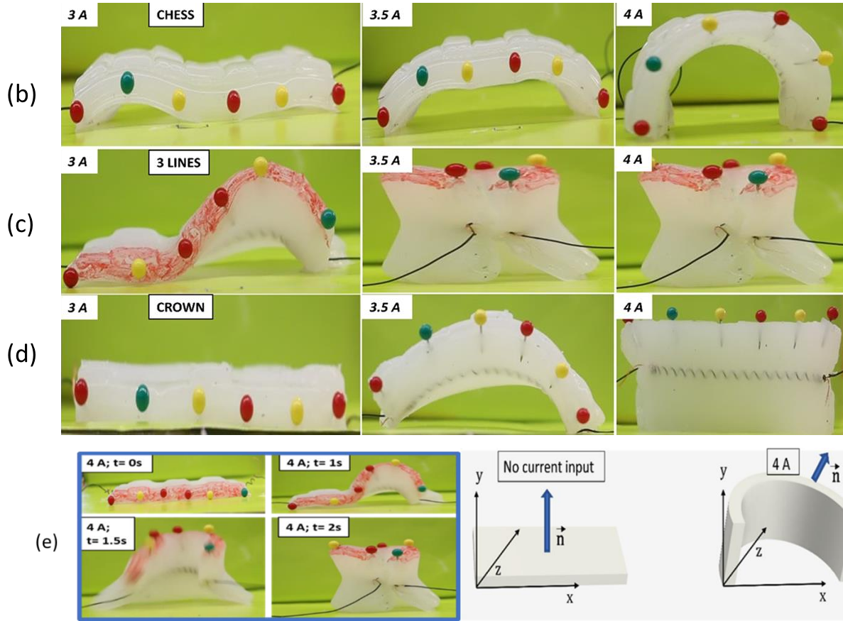
Fig. 3-17- a) Patterned silicone skins motions in x-y space at three different current inputs (average on 10 measurements), b) Chess structure motions at 3 different current inputs, c) Three lines structure motions at 3 different current inputs, and d) Crown structure motions at 3 different current inputs, e) Dynamic of the Three lines out of plane deformation.
