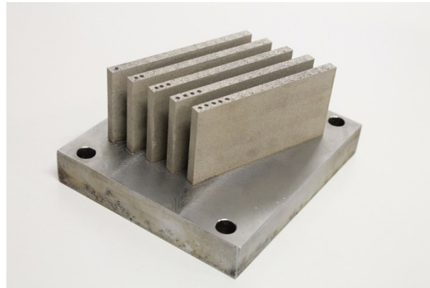
Figure 125. Substrates for laser-powder bed fusion.
