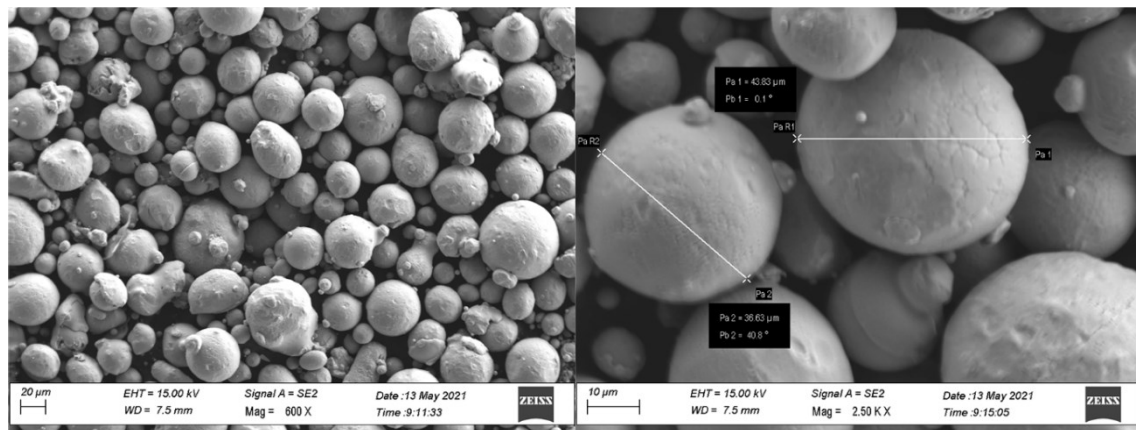
Figure 127. SEM images of the powdered AISI 316L used to make the L-PBF substrates. In the detail, the related dimensions are also mentioned.
