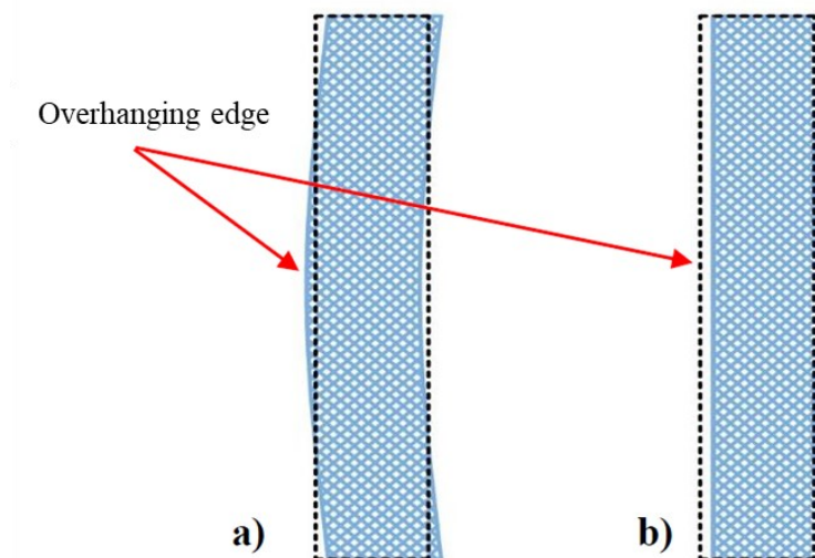
Figure 119. Schematic representation of the distortion phenomenon in the XY plane where the blue represents layer n ; the black line represents the laser scanning path of layer n+1 . (a) case with distortion; (b) case without distortion.
