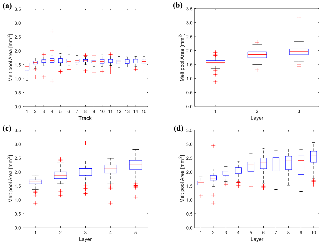
Figure 146. Trend of the melt pool area: (a) sample 1_C; (b) sample 3_C; (c) sample 5_C; (d) sample 10_C.
