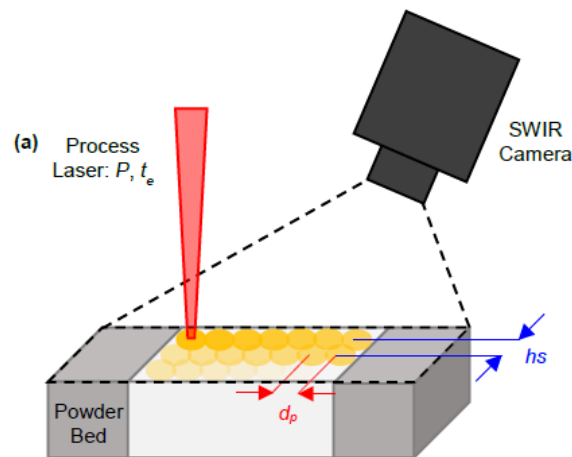
Figure 75. Schematic representation of the thermal monitoring system implemented in this work [119].
