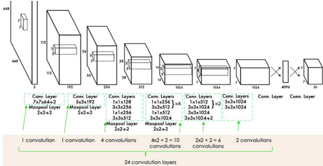
Fig. 2.13 A typical architecture of YOLO network
