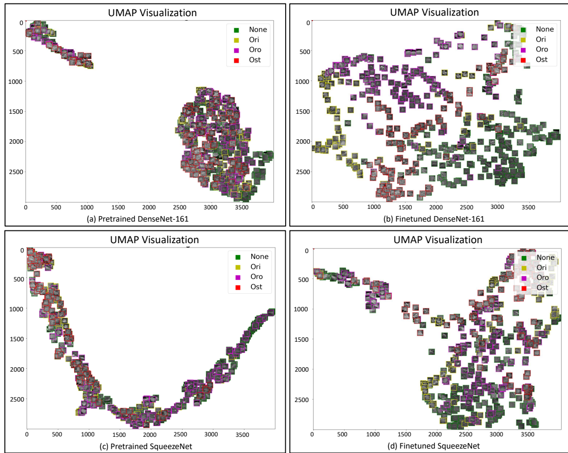
Fig. 7.4 The UMAP embedding plots of the features extracted from the pretrained (a,c) and fine-tuned (b,d) DenseNet-161 and SqueezeNet, respectively, on the validation set of 1st fold. It is distinctly visible that the fully TL paradigm does not allow a clear clustering of the features in low-dimensionality space, whereas the finetuned model is able to discover more discriminative features with respect to its pretrained-only version.
