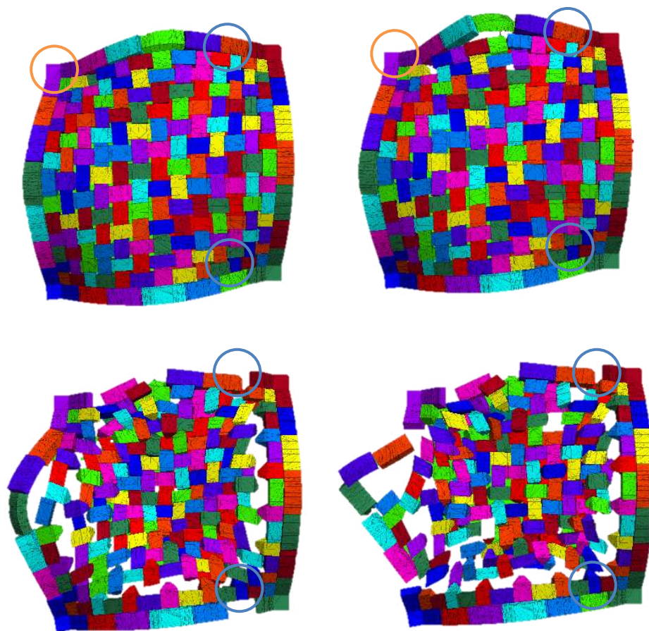
Figure 5-5. Deformed shape test set-up A: zenith view; in the blue circle the fixed abutments and in orange one the first ashlar that falls.
