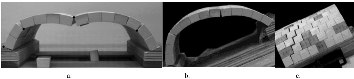
Figure 2-19. Barrel vault collapse mechanism: a. longitudinal openings of two adjacent abutments (hinge on the crown); b. tilting in-plane angle = 0^\circ ; c. tilting in-plane angle = 45^\circ (Shapiro, 2012).
