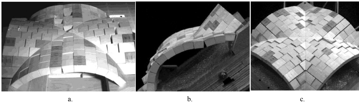
Figure 2-18. Cross vault collapse mechanism: a. longitudinal openings of two adjacent abutments (hinge on the crown); b. tilting in-plane angle = 0^\circ ; c. tilting in-plane angle = 45^\circ (Shapiro, 2012).
