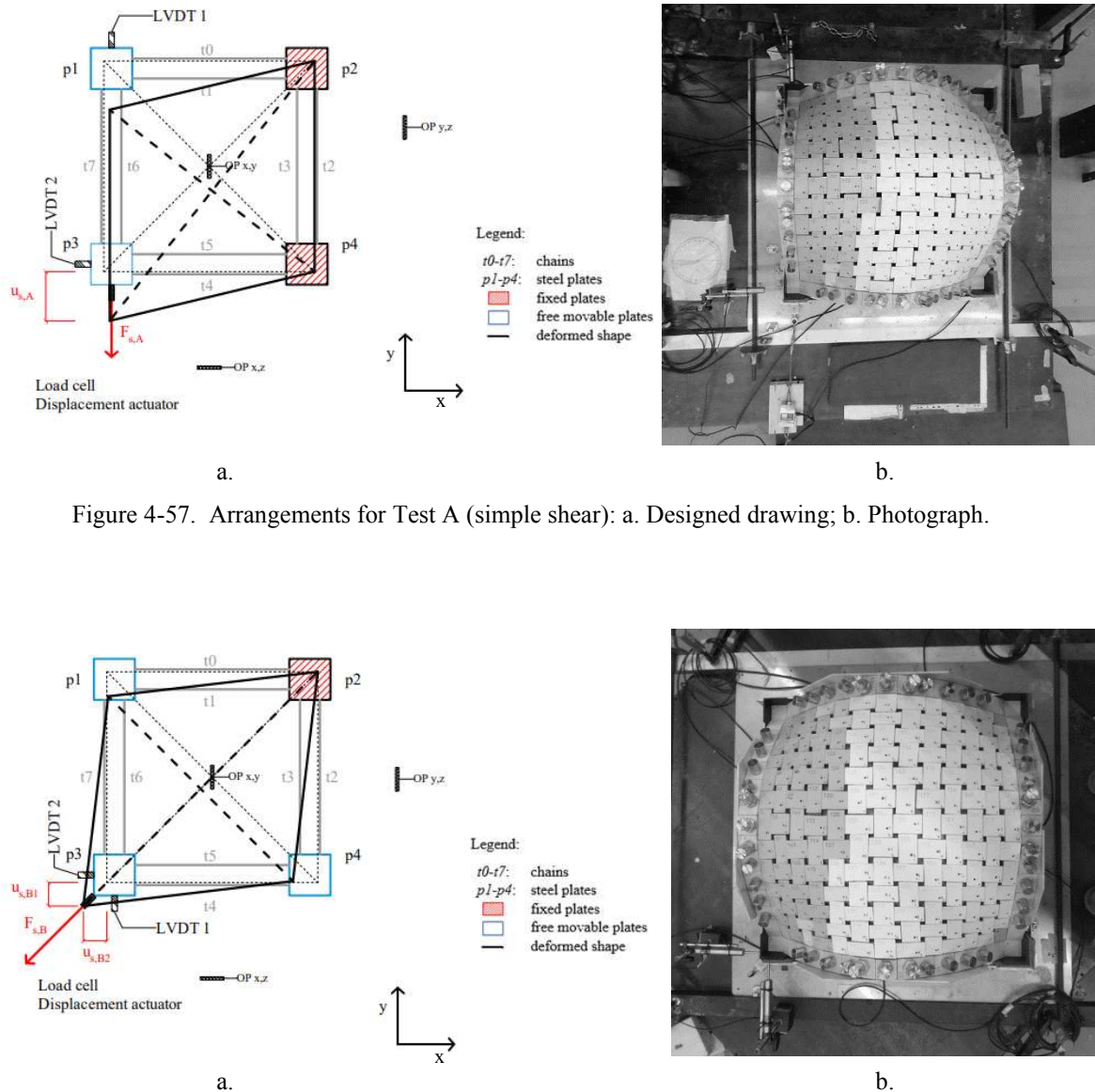
Figure 4-58. Arrangements for Test B (pure shear): a. Designed drawing; b. Photograph.
