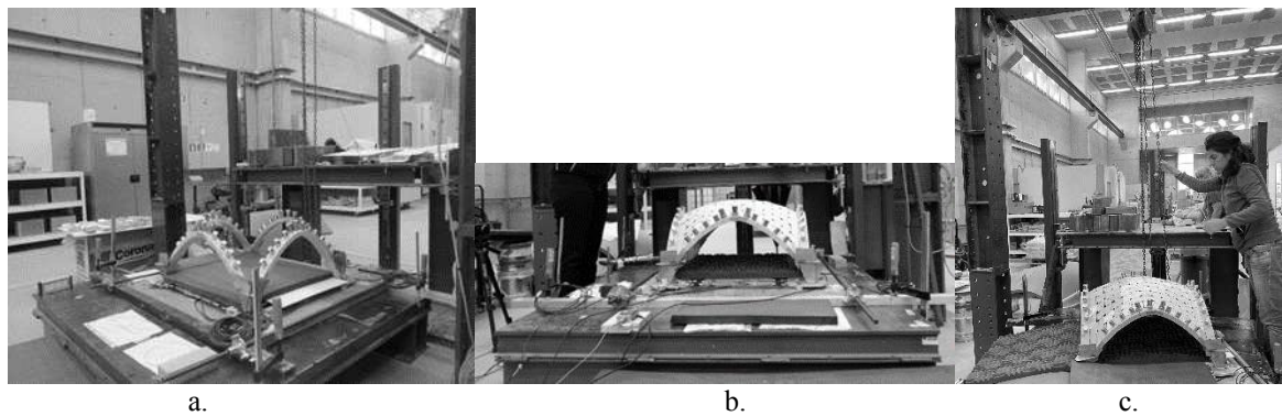
Figure 4-67. Set-up DSA Test: a. The tilting table; b. Detail of the hinges; c. System chain plus tackle pulley.
