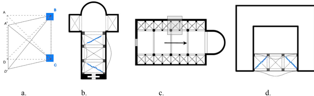
Figure 4-52. In-Plane horizontal shear: a. Displacement setting; b. Damage mechanisms in single nave churches, c. Damage mechanisms in three naves churches and d. Damage mechanisms in buildings. (Rossi et al., 2016).
