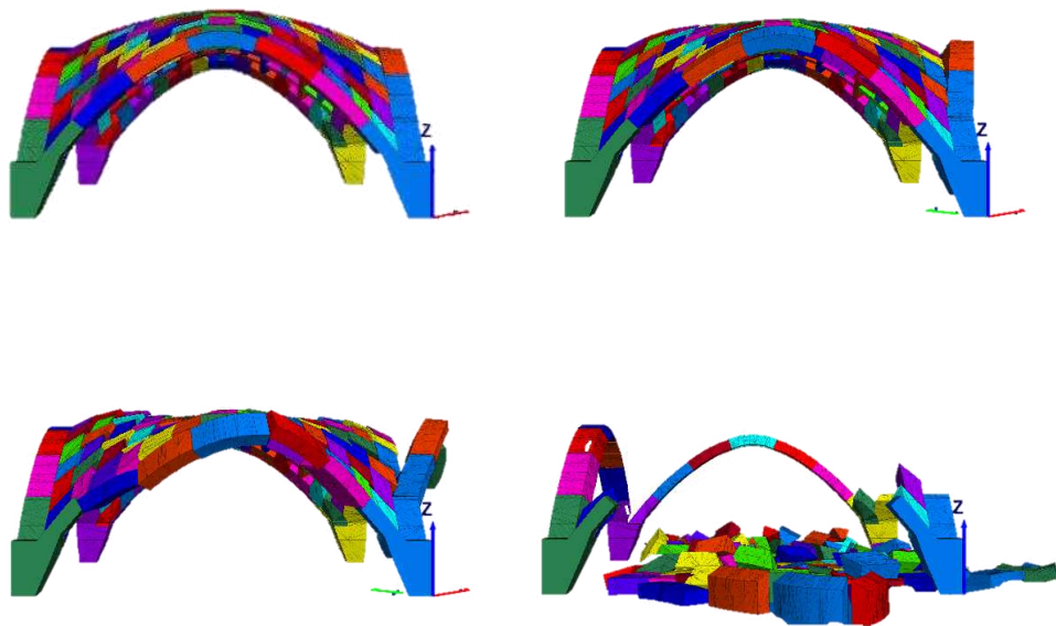
Figure 5-20. Damage results of the numerical tilting tests with \Phi = 45^\circ : damage evolution in the lateral view ( p1-p3 ).
