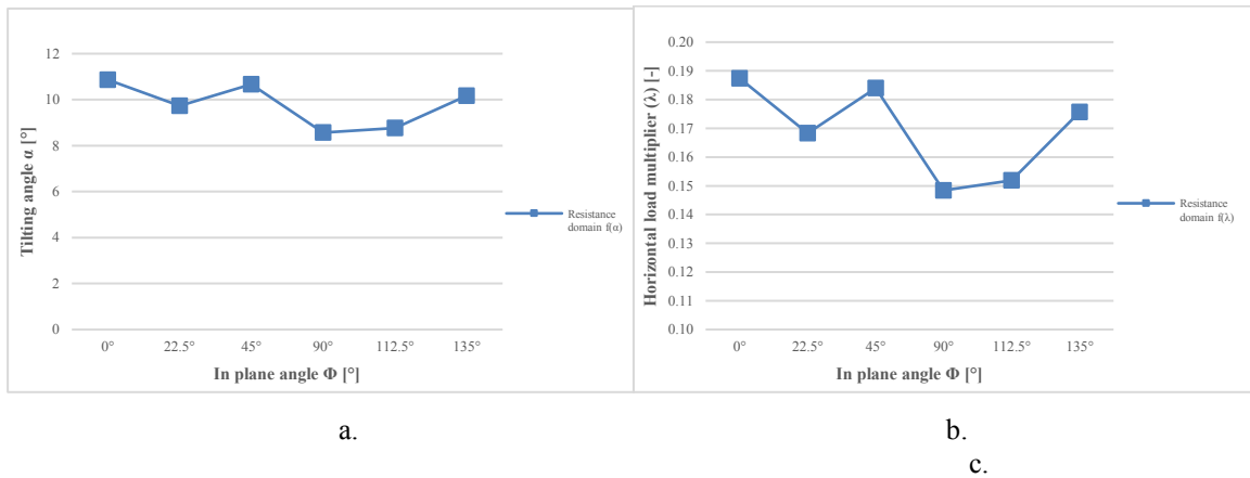
Figure 4-88. Representative curve of the resistance domain of the vault based on the direction of the seismic action: a. in function of tilting collapse angle ( \alpha ); b. in function of Horizontal load multiplier ( \lambda ).
