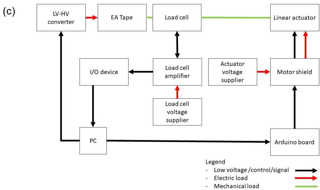
Figure 3.5 – The experimental set-up components. (a) The set-up includes a linear actuator that provides the pulling displacement, controlled by an Arduino board and a motor driver; the force is measured with a load cell: the load cell amplifier sends the force signal to an I/O device. The Arduino board and the load cell are driven with homemade Arduino and MATLAB codes, respectively. Two voltage suppliers provide the supply for the actuator and amplifier. (b) Details of the set-up adapted for pulling test on curved substrate. An additional curved substrate is fixed onto the flat one and a LV-HV converter is utilized to supply the EA tape. (c) Flow diagram of the set-up.
