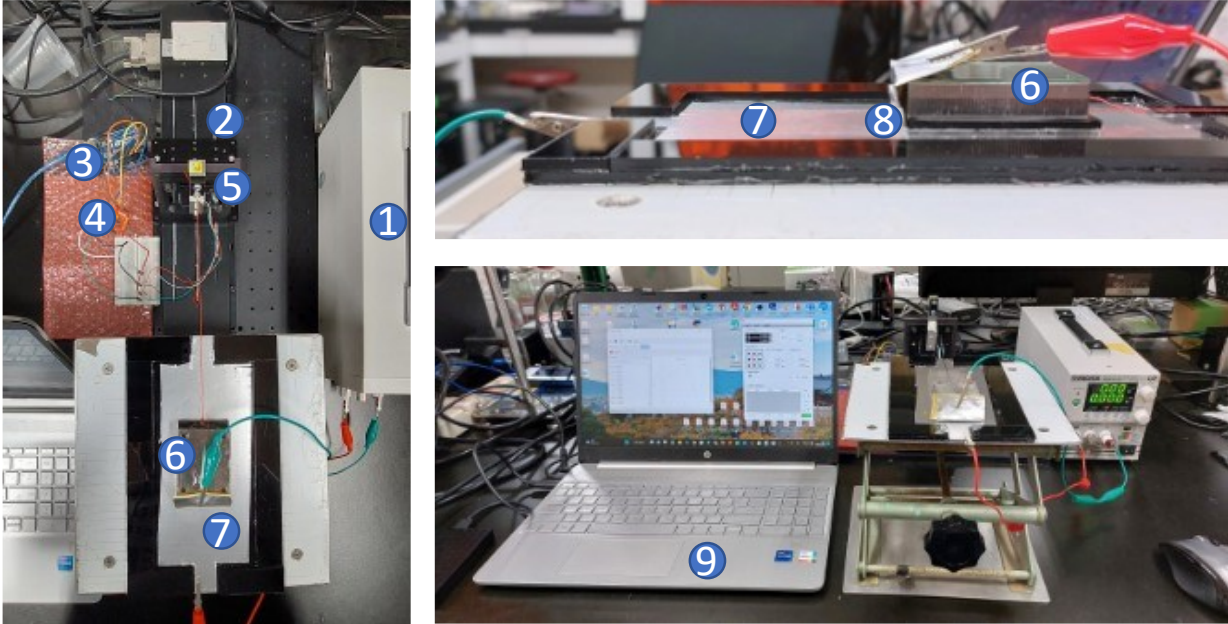
Figure 4.2 Views of the experimental set-up used for friction tests of hydrogels. The set-up is composed by: (1) voltage supplier, (2) linear stage, (3) Arduino board, (4) load cell amplifier, (5) load cell, (6) sliding mass, (7) substrate, (8) hydrogel, (9) pc, and a linear stage controller (not in the picture).
