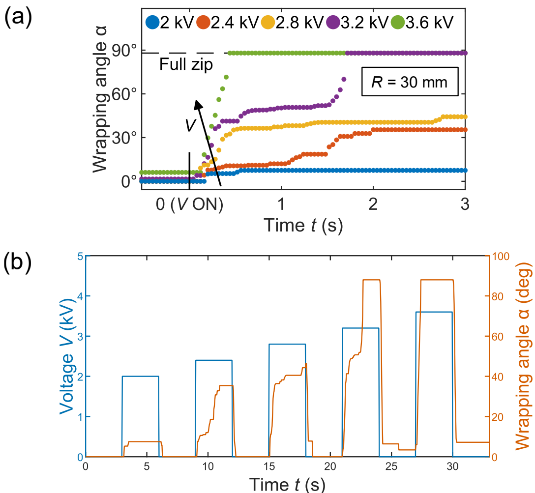
Figure 2.15 – (a) Dynamical tests of the zipping of an EA tape on a 30 mm paper-covered curved object (see Section 2.3.1.1). Only when a voltage equal to 3.2 kV is applied (like the V_{FULL ZIP} value predicted by the model for the quasistatic case) the tape fully wraps the object. For higher voltage (3.6 kV) the wrapping is faster. (b) Complete zipping and unzipping cycles (3 sec voltage on, 3 sec voltage off). Reproduced with permission from Mastrangelo et al. [1].
