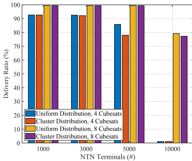
FIGURE 3.8: Delivery Ratio.
