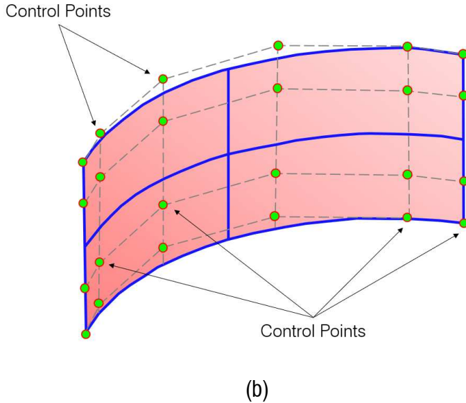
Fig. 4.10 - NURBS geometries: example of NURBS curve (a) and NURBS surface (b).
