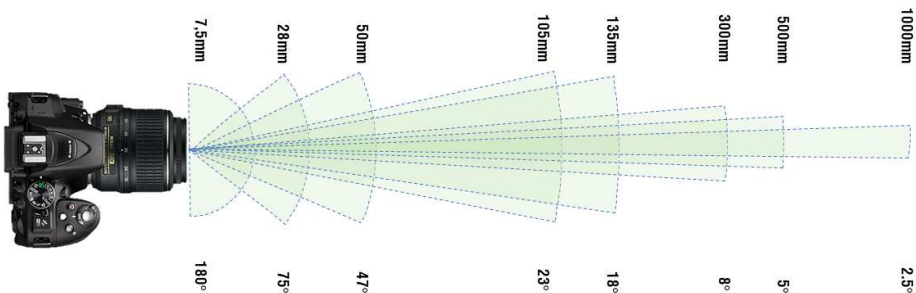
Fig. 1.3 - Angle of field and focal lengths.
