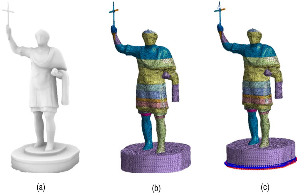
Fig. 6.11 - Parametric 3D model for FEM analysis: NURBS processed in Rhino software (a), structural mesh (b), base constraint condition (c).
