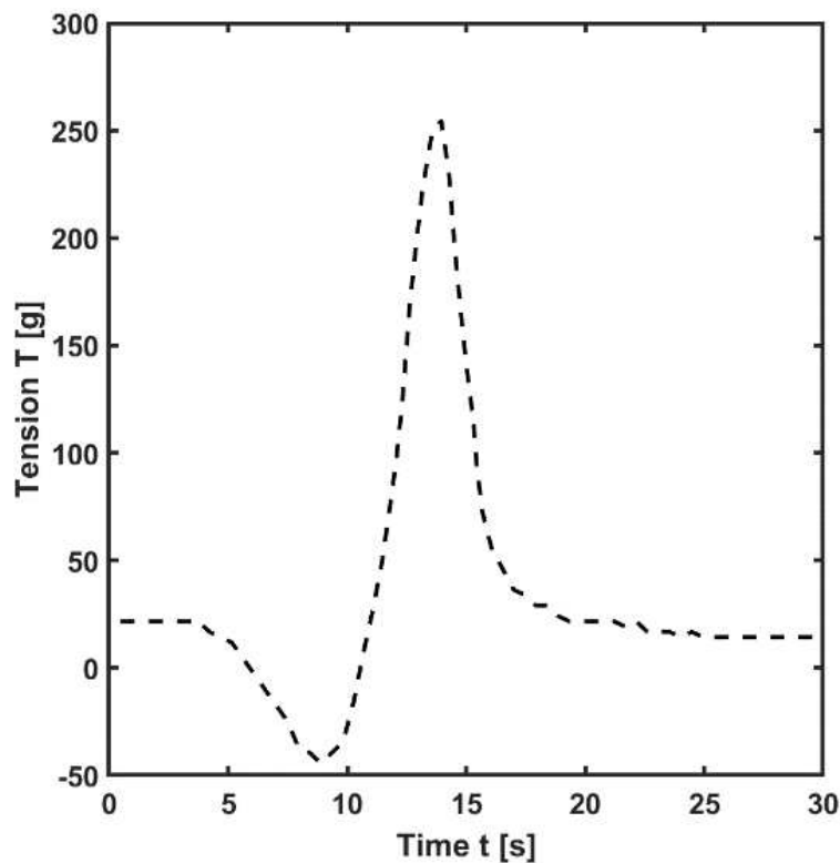
Figure 4.2.6 Drawing tension T as a function of the fabrication time t .
