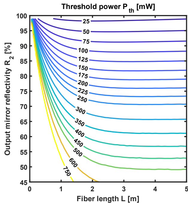
Figure 5.2.6 Threshold power P_{th} as a function of the fiber length L and the output mirror reflectivity R_2 . Dopant concentration N_{Er} = 5 \times 10^{25} \text{ ions/m}^3 , input mirror reflectivity R_1 = 99\% .
