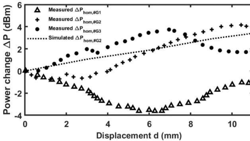
Figure 3.4.13 Measured peak power change \Delta P_{m,hom} versus the displacement d for the high order mode of the grating #G1 (triangle markers), #G2 (cross markers), #G3 (circle markers) and simulated peak power change \Delta P_{s,hom} for the grating #G2 (dotted curve) [68].
