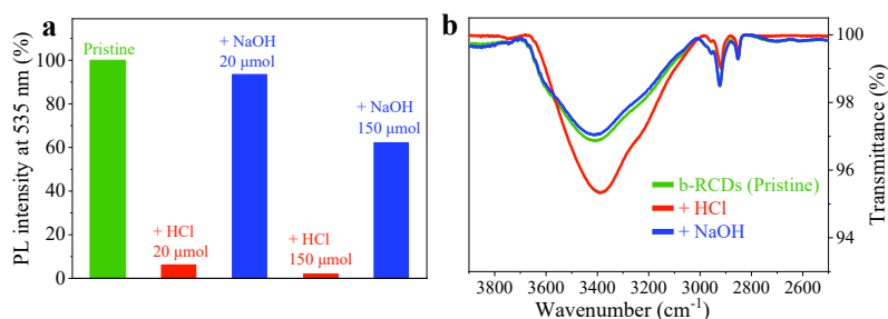
Figure 3.10: (a) PL intensity at 535 nm for pristine b-RCDs and after cyclic addition of HCl aq and NaOH aq , expressed as a percentage of the initial intensity; (b) O–H stretching band observed in the FT-IR spectra of b-RCDs before and after subsequent addition of HCl and NaOH [2].
