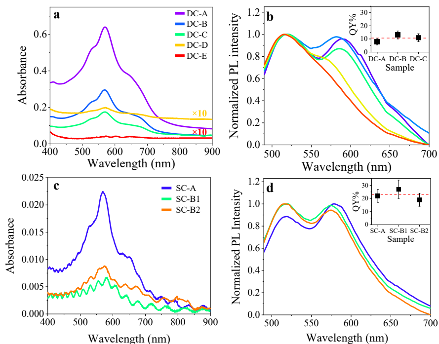
Figure 5.3: UV-Vis absorption and normalized PL ( \lambda_{exc} = 465 nm) spectra of (a, b) drop casted and (c, d) spin-coated DCD nanocomposites; the inset of (b, d) reports the PLQYs ( \lambda_{exc} = 465 nm) of the nanocomposite samples; the dashed red line is a guide to the eye, and it is traced in correspondence of the weighted average of the PLQYs (where weights are the experimental errors) [1]
