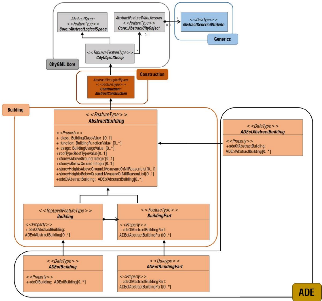
CityGML UML Structure of Building Thematic Class
