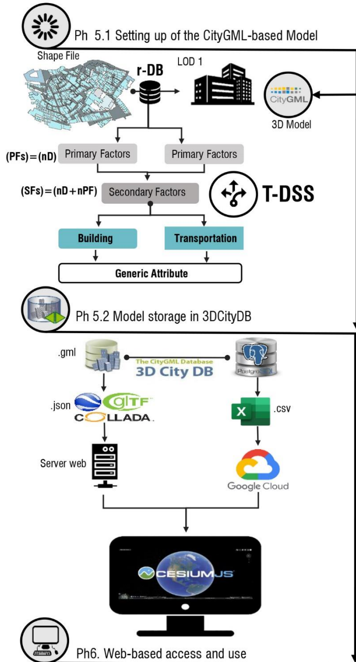
Figure 26 - Conceptual structure relating to the phases and tools for the development of the parametric model CityGml-based
