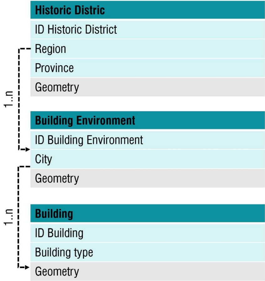
Figure 8 - The logical-relational model In detail, entity classes are represented by an attribute table, the columns of which are defined as fields and the rows as records/tuples. Each row defines the specific entity.
