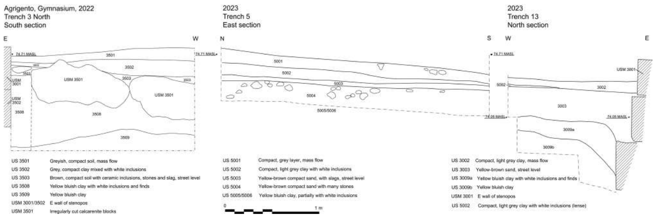
Fig. 3. Stenopos connected sections: trench 3N south, trench 5 east, trench 13 north (B. Kupke, M. Trümper, J. Winzek).
