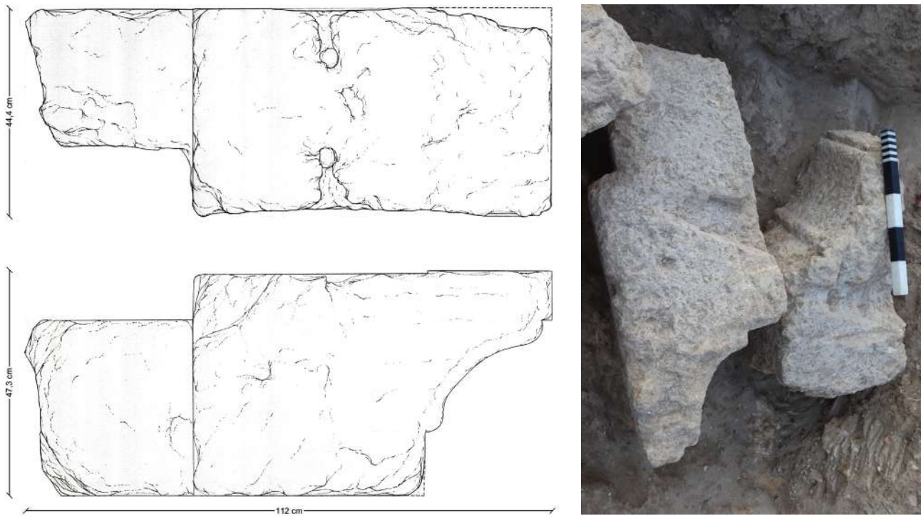
Fig. 47a,b. Moulded crown blocks: a. drawing of Cor 1 (M. Delfino); b. view of the blocks (R. Schönell).
