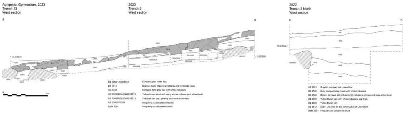
Fig. 4. Stenopos west sections: trench 3N, trench 5, trench 13 (B. Kupke, M. Trümper, J. Winzek).
