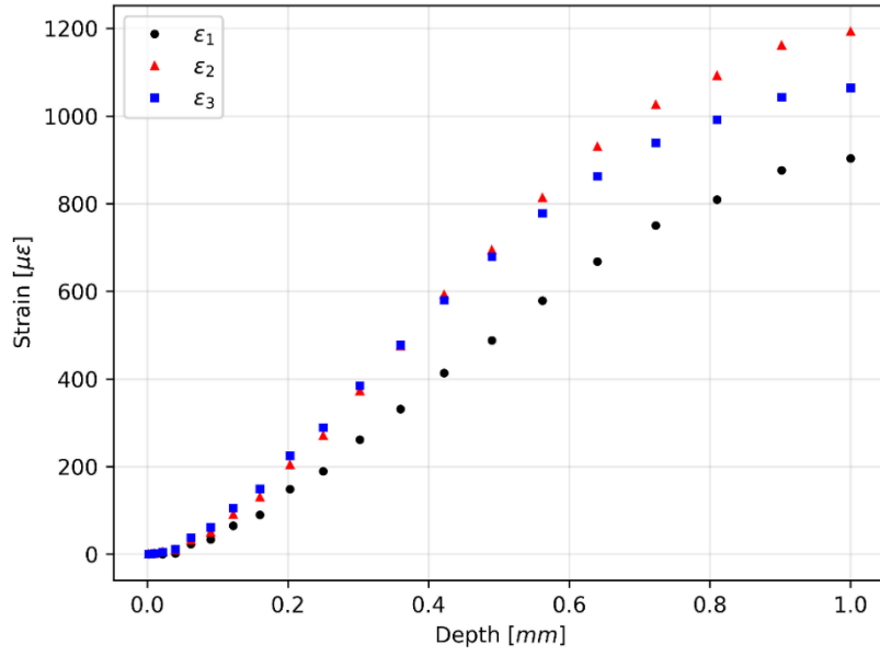
Figure 65. Measured strain variation with depth in the three strain gauges directions.
