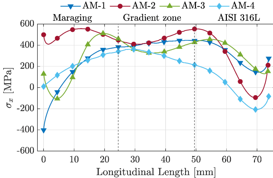
Figure 56. Comparison of residual stresses throughout the longitudinal length of the four specimens, extracted from the contour method stress maps along a horizontal line at 0.3 mm below the top surface.
