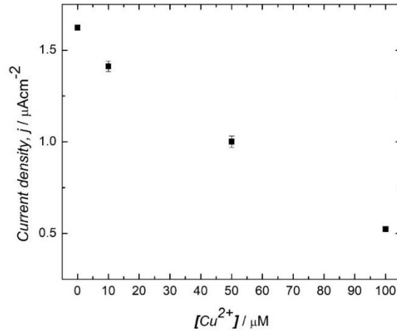
Figure 4.31: Relationship between CuSO 4 concentrations and current density during chronoamperometry at E APP : +0.40 V. R 2 : 0.998 for bioelectrodes prepared by immobilizing WT cell cultured in YPD. Error bars indicate one standard deviation.
