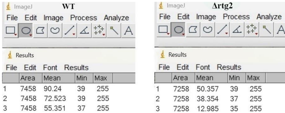
Figure 6.6: Numerical results from wild type ( WT ) and RTG2-lacking strain ( \Delta rtg2 ) without and with NaCl stress using ImageJ software. In both panels ( WT and \Delta rtg2 ), 1, 2 and 3 were referred to control cells, 0.4 and 0.8 M NaCl treated cells, respectively. The mean of each sample corresponded to the numerical results calculated using ImageJ protocol [240].
